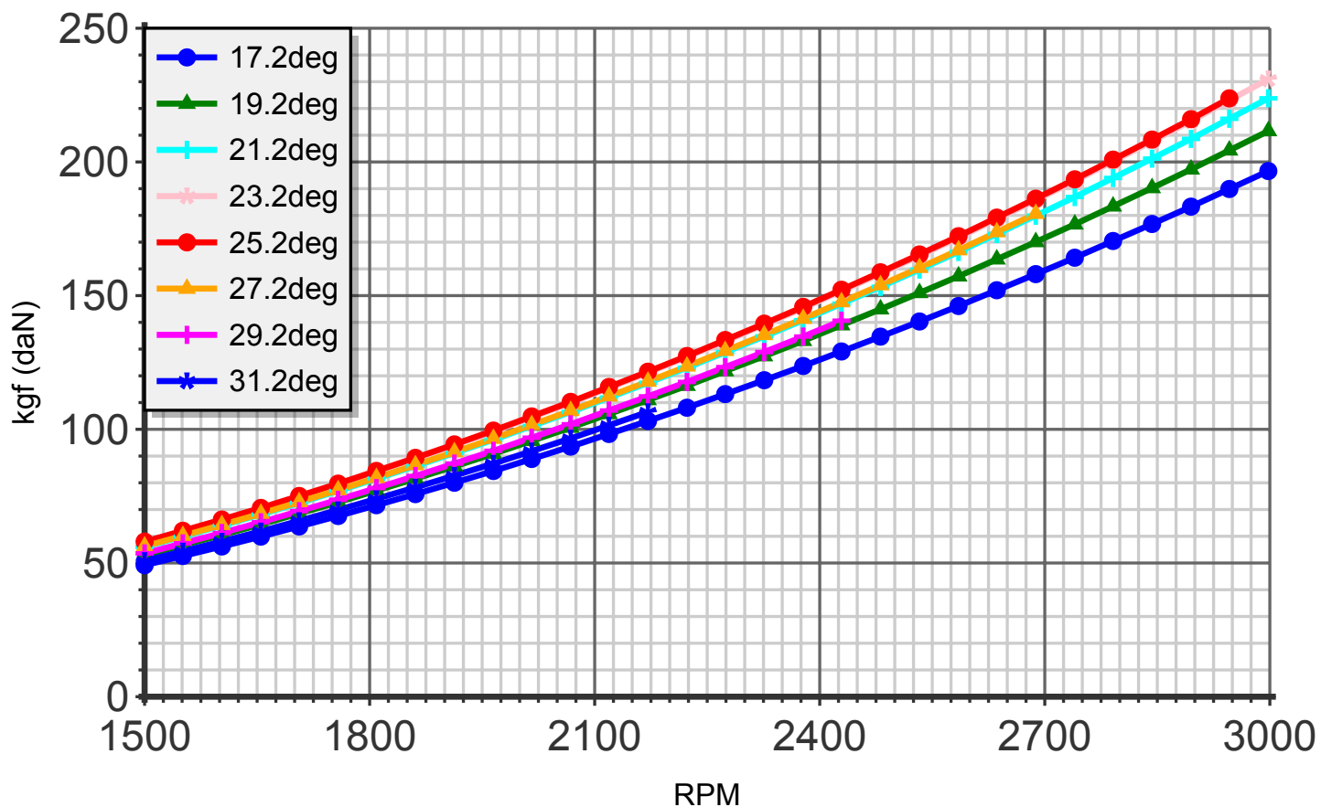
Thrust (blade:2 diameter:165cm C4)
