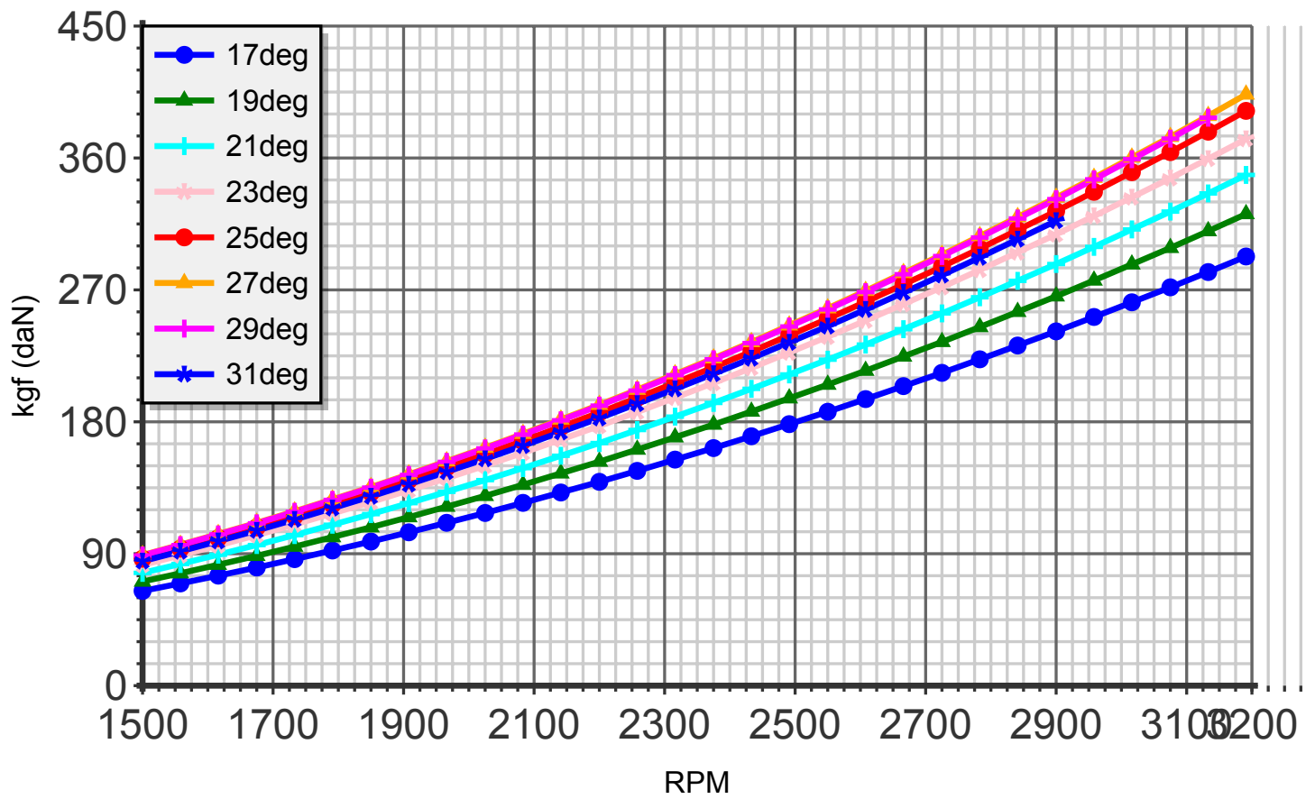
Thrust (blade:4 diameter:152cm C4)
