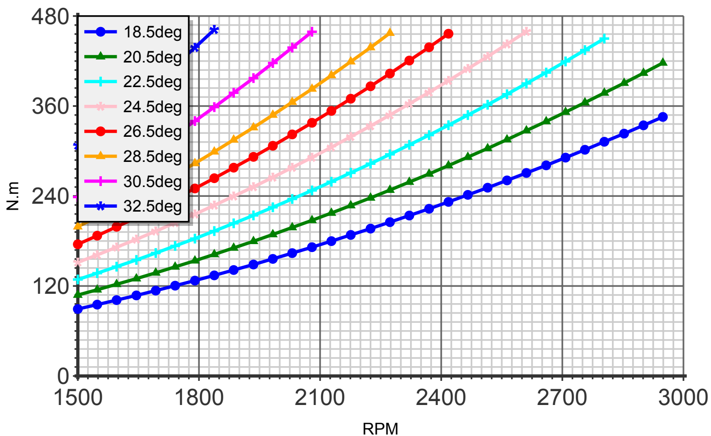
Torque (blade:3 diameter:170cm C8)
