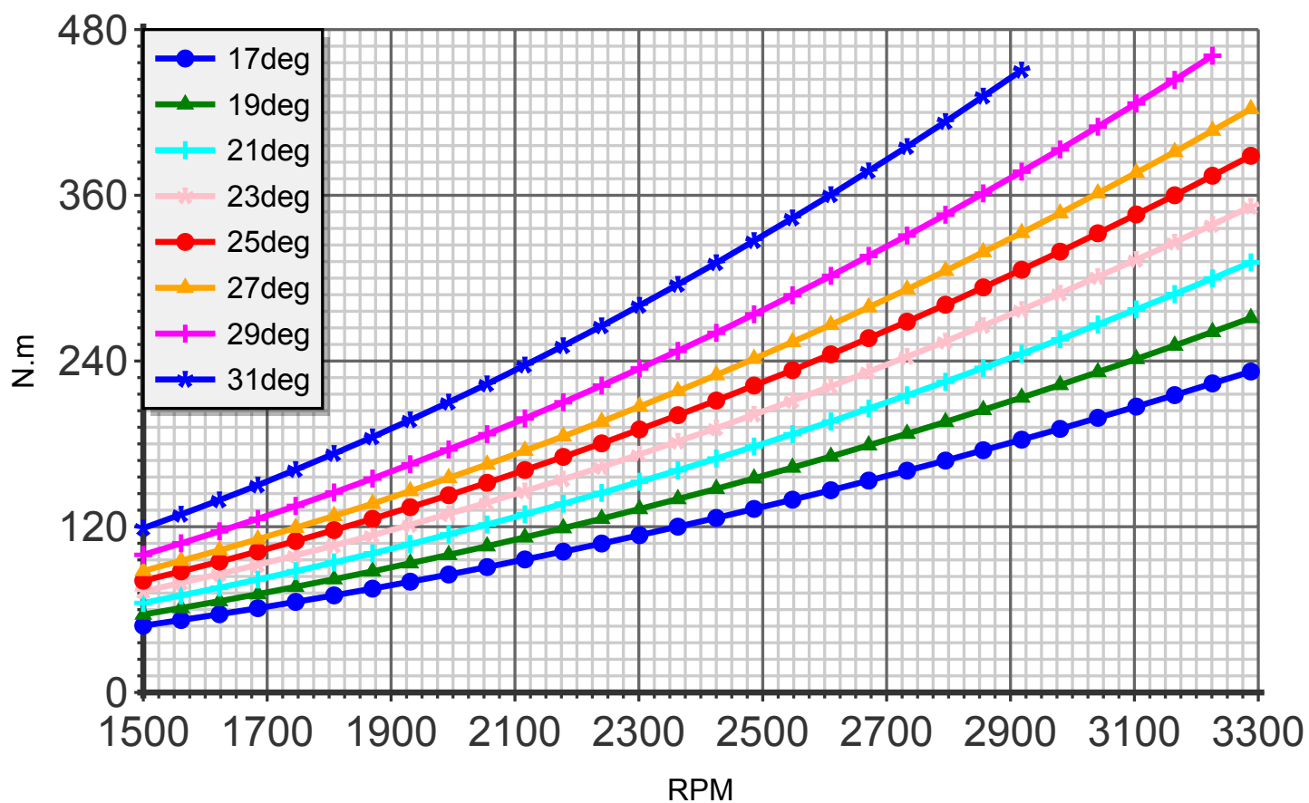
Torque (blade:3 diameter:150cm C4)
