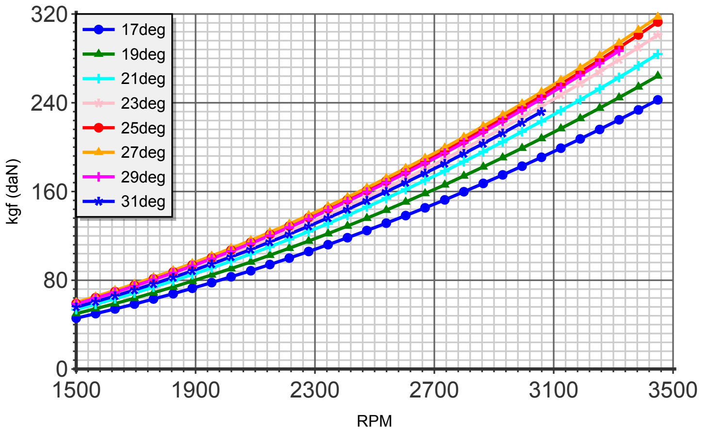
Thrust (blade:3 diameter:145cm C4)
