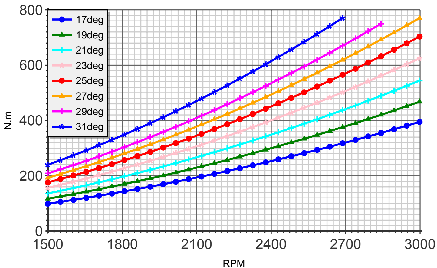
Torque (blade:5 diameter:164cm C4)
