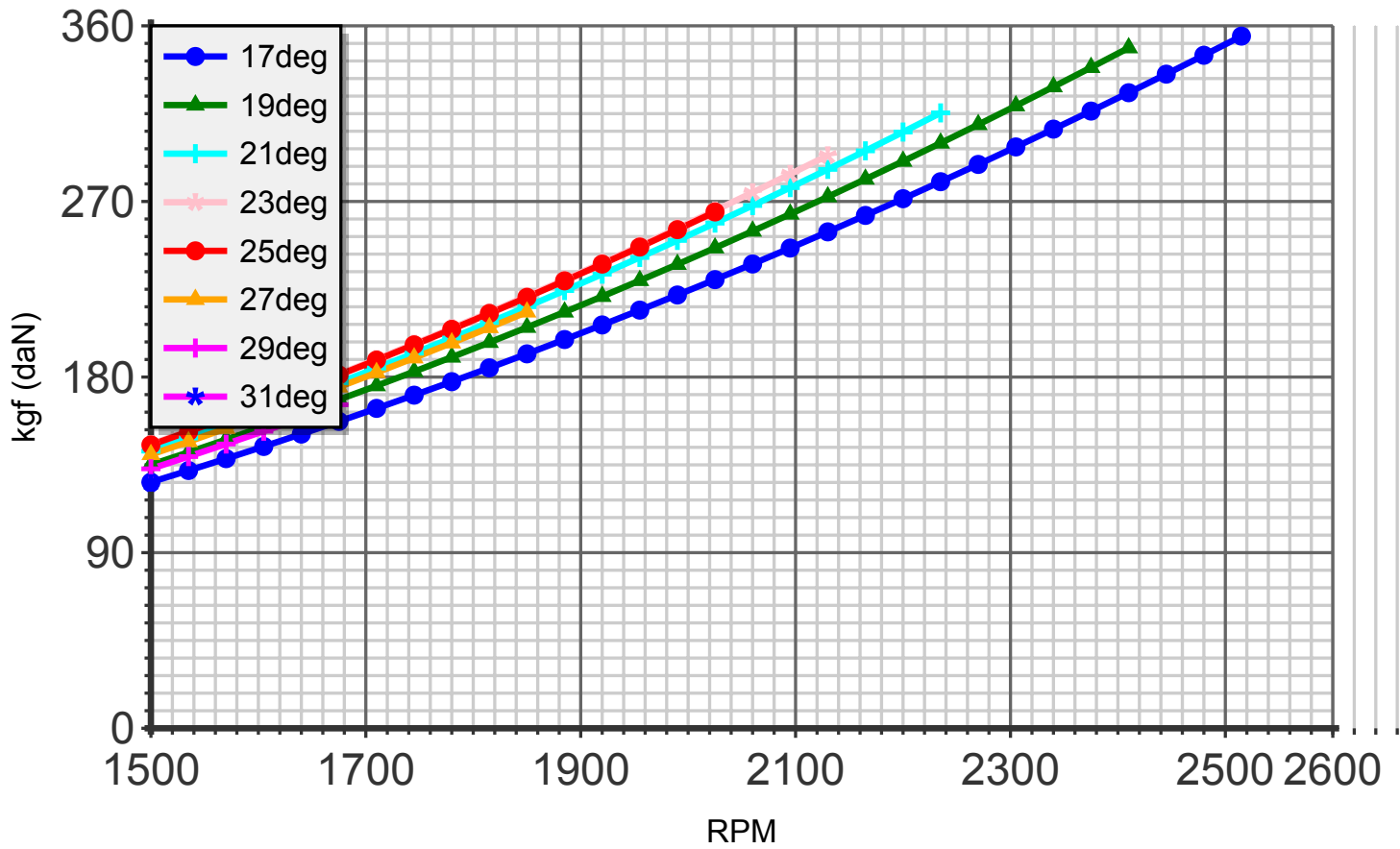
Thrust (blade:3 diameter:195cm C4)
