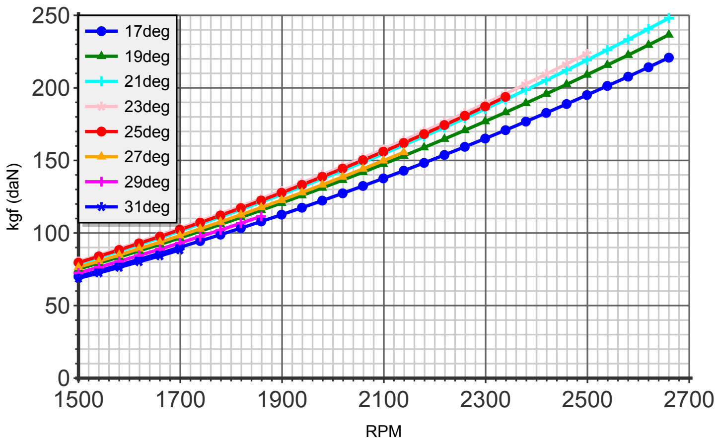
Thrust (blade:2 diameter:185cm C4)
