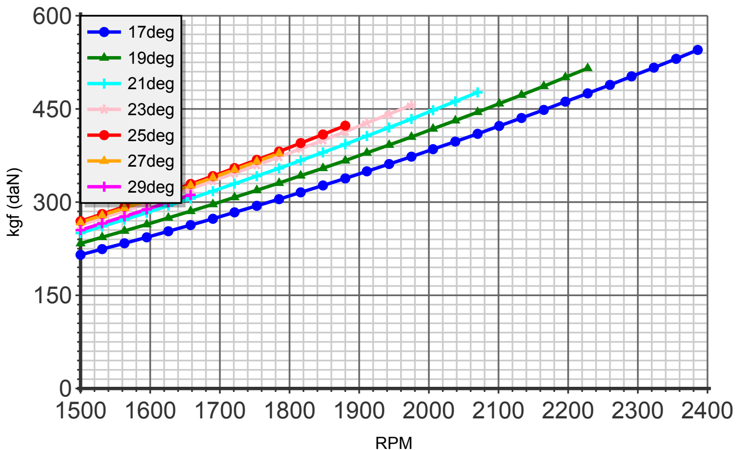
Thrust (blade:5 diameter:204cm C4)
