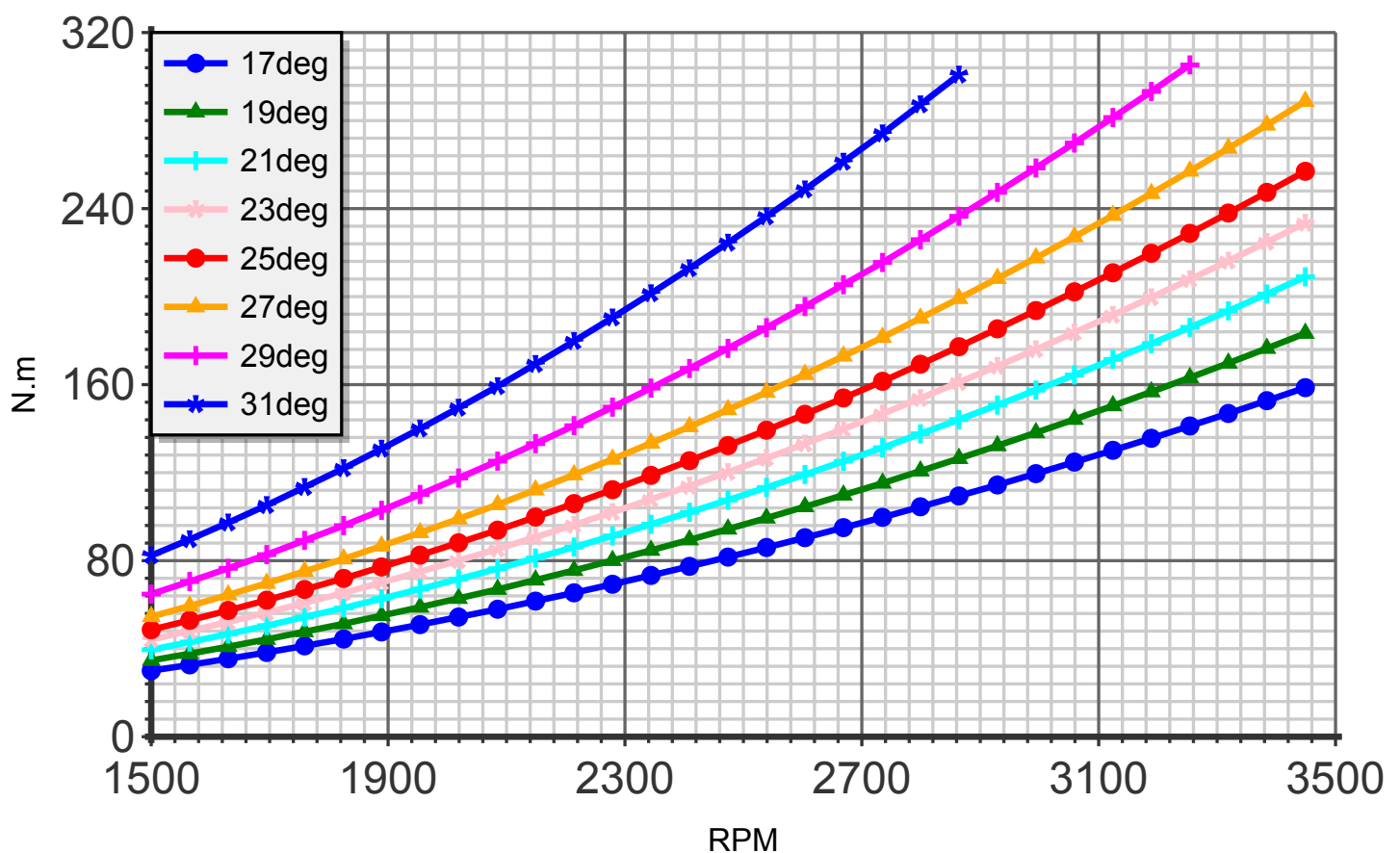
Torque (blade:2 diameter:145cm C4)
