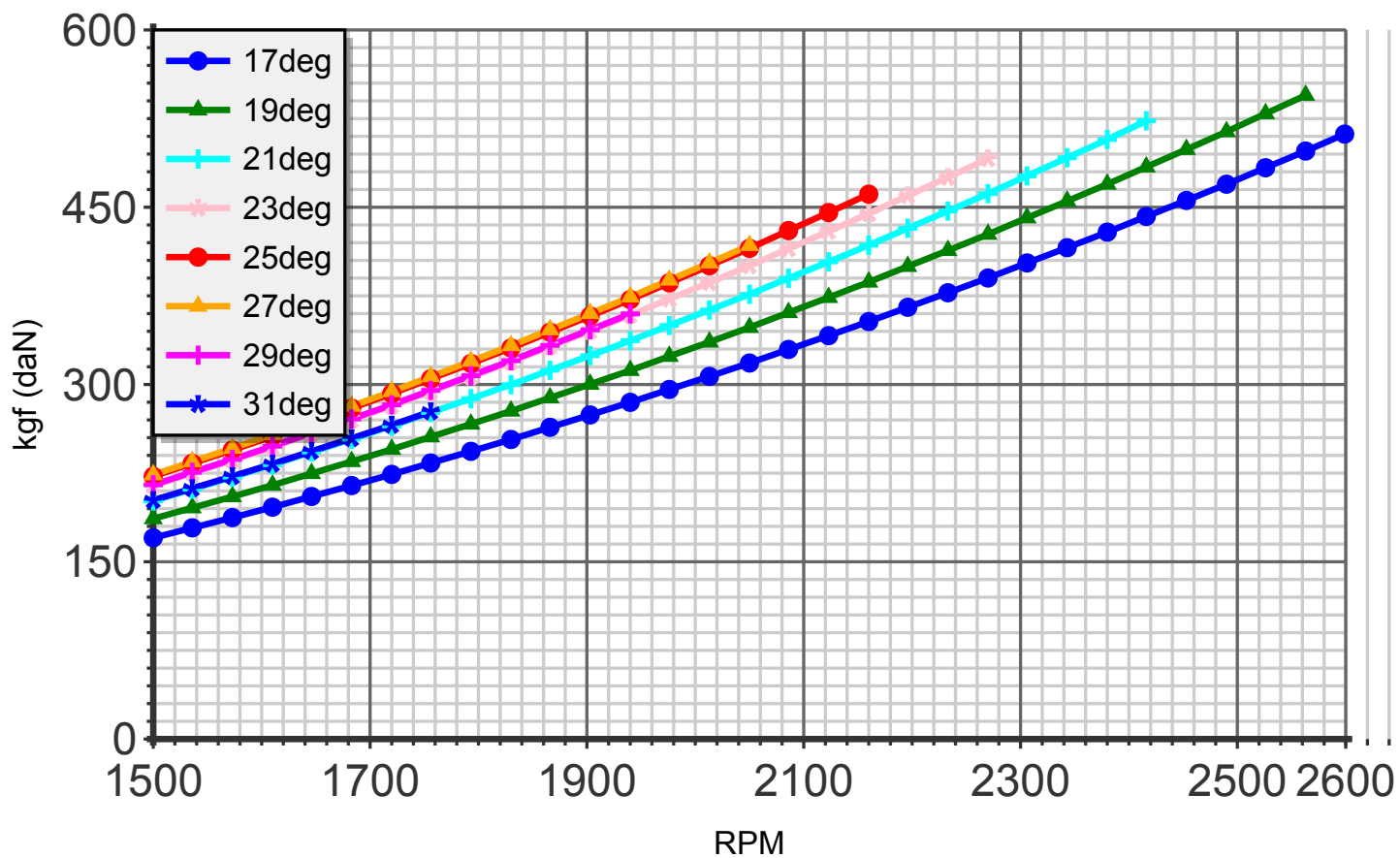
Thrust (blade:5 diameter:194cm C4)
