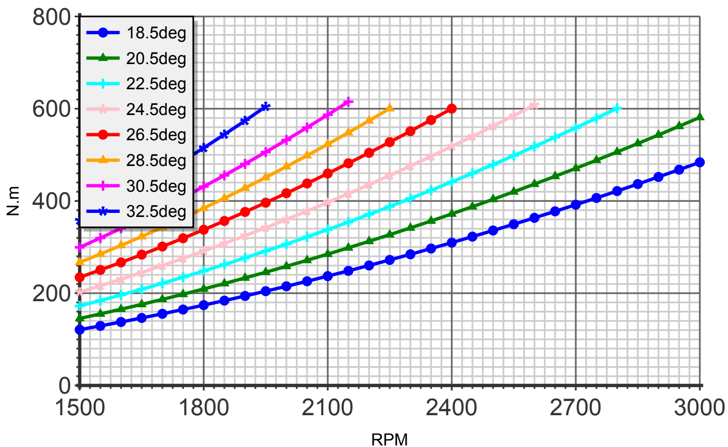
Torque (blade:4 diameter:167cm C8)
