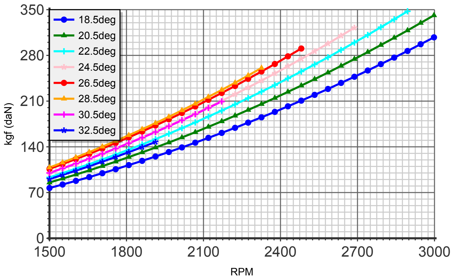
Thrust (blade:3 diameter:165cm C8)
