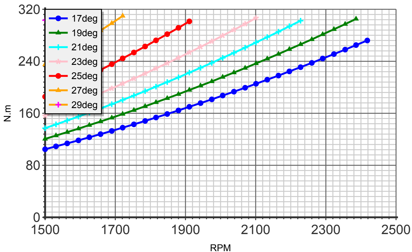
Torque (blade:2 diameter:205cm C4)
