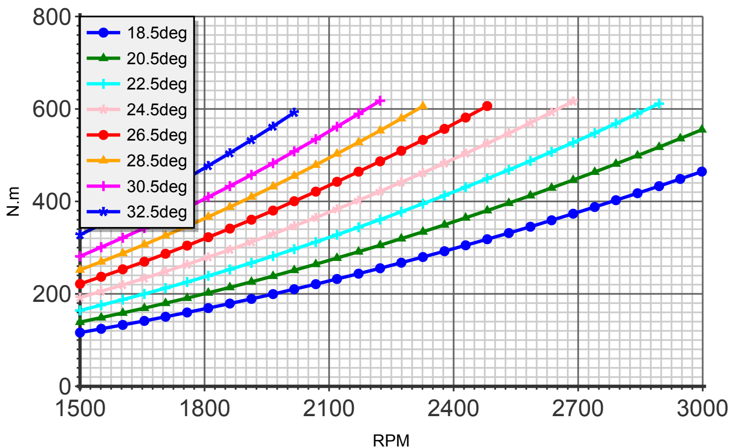
Torque (blade:4 diameter:162cm C8)
