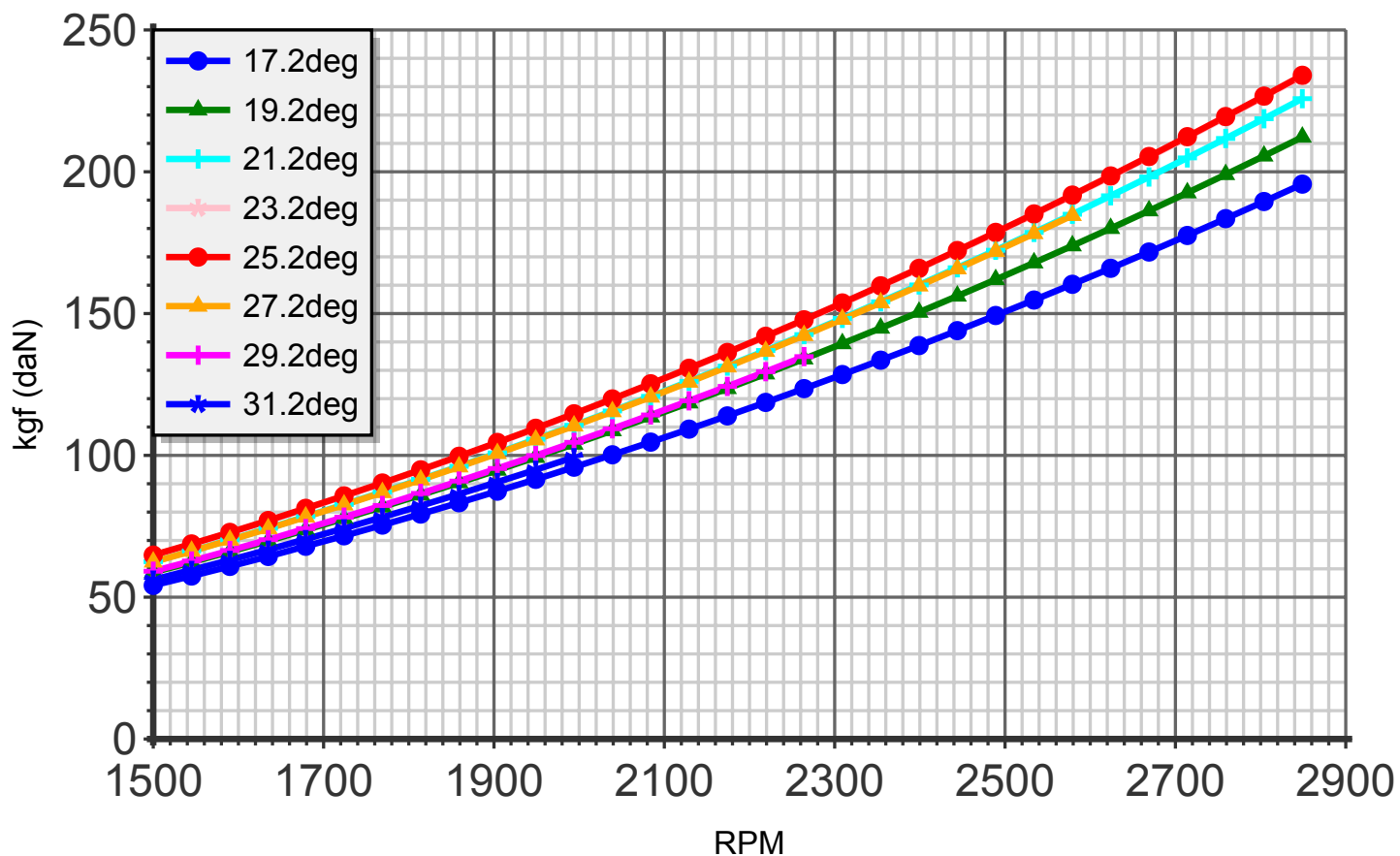
Thrust (blade:2 diameter:175cm C4)
