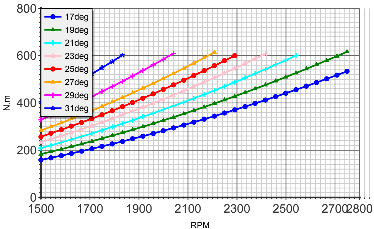
Torque (blade:4 diameter:182cm C4)
