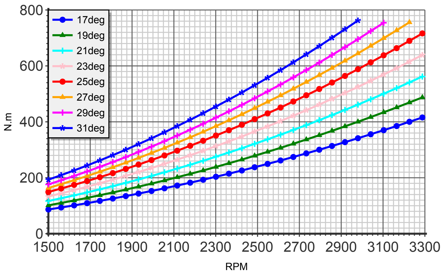
Torque (blade:5 diameter:149cm C4)
