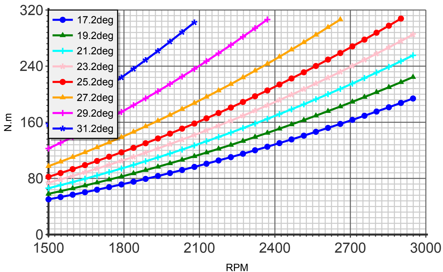
Torque (blade:2 diameter:170cm C4)
