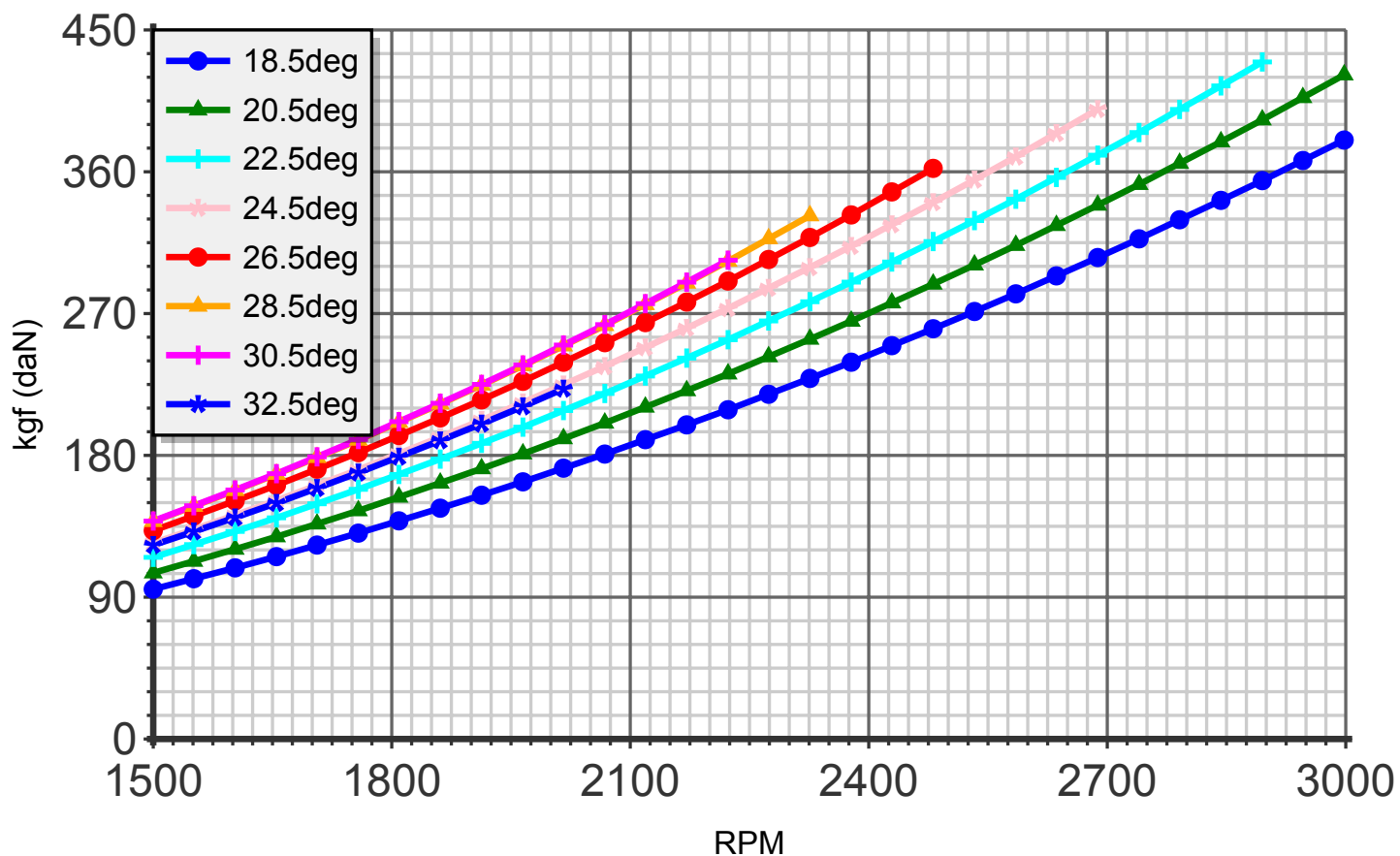
Thrust (blade:4 diameter:162cm C8)
