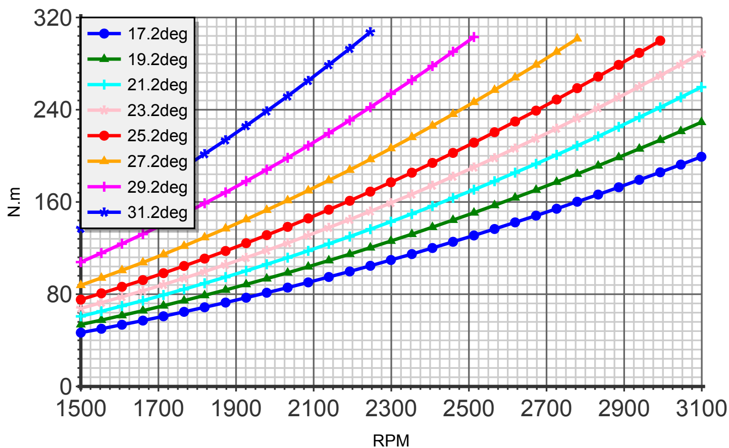
Torque (blade:2 diameter:160cm C4)
