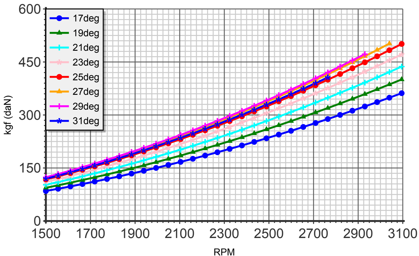
Thrust (blade:5 diameter:159cm C4)
