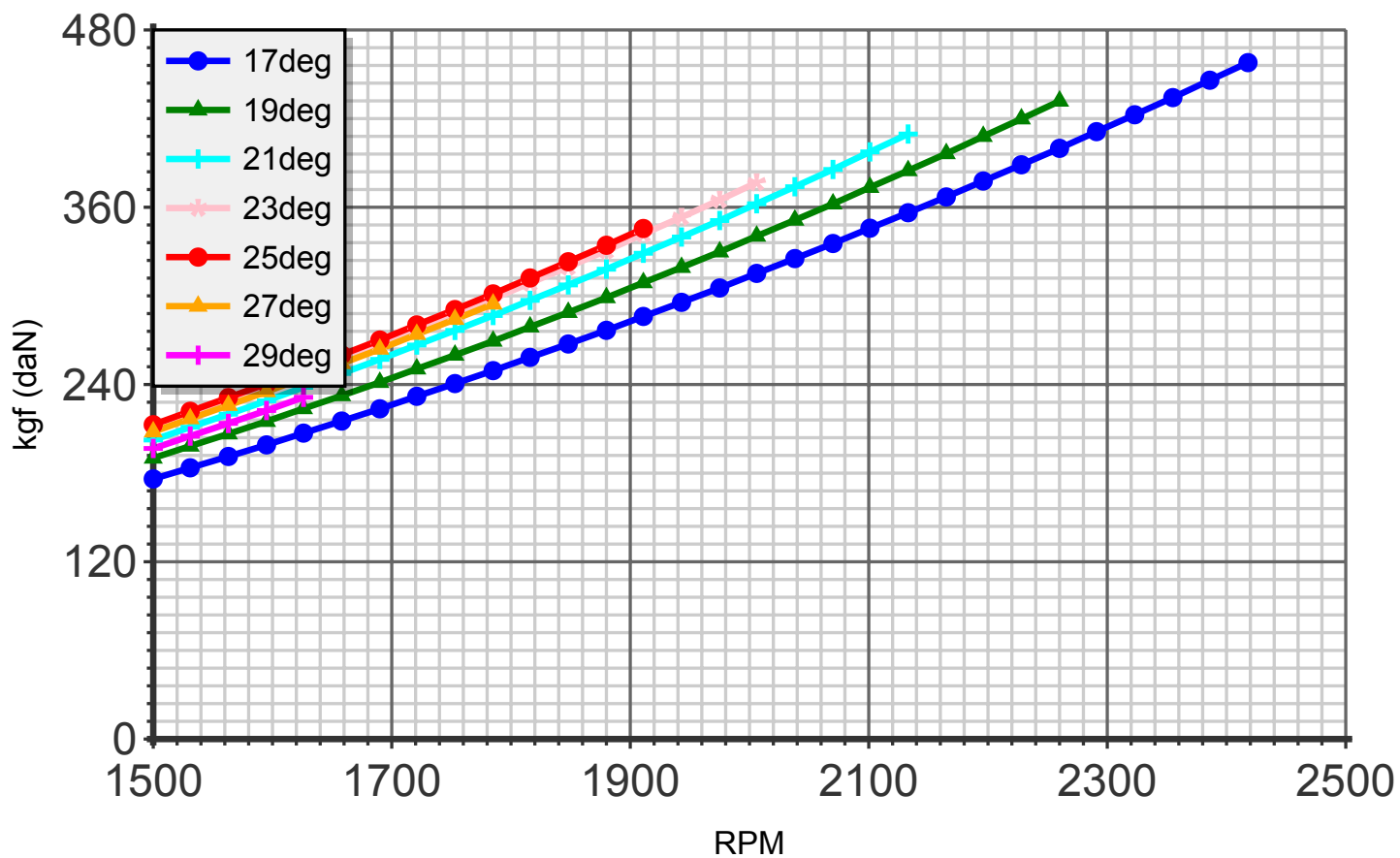
Thrust (blade:4 diameter:203cm C4)
