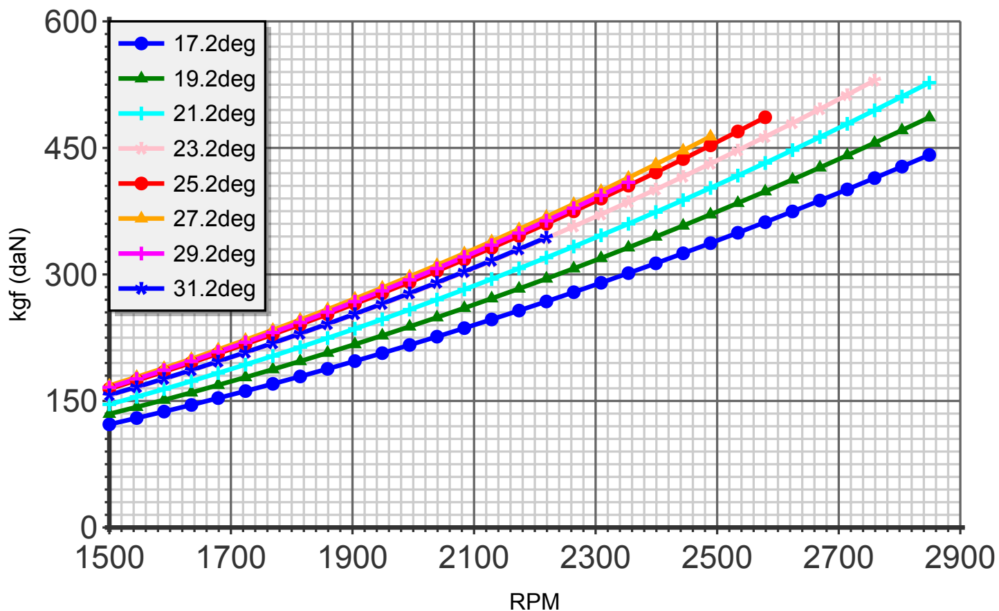
Thrust (blade:5 diameter:176cm C4)
