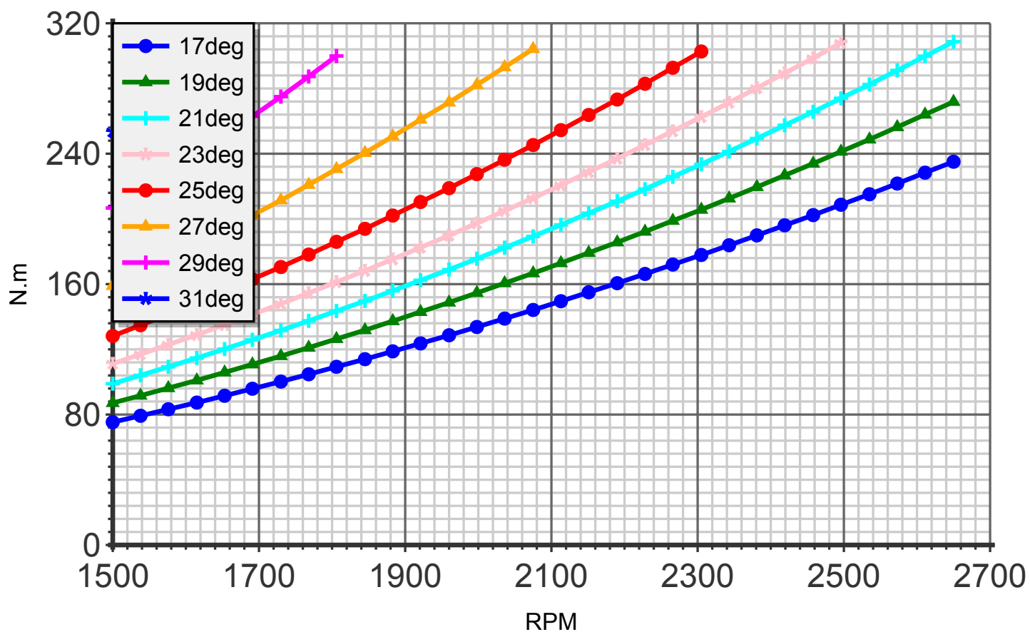
Torque (blade:2 diameter:190cm C4)
