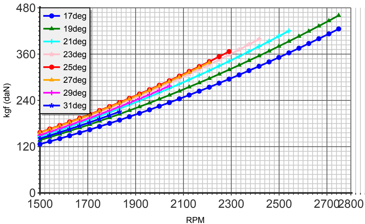
Thrust (blade:4 diameter:182cm C4)
