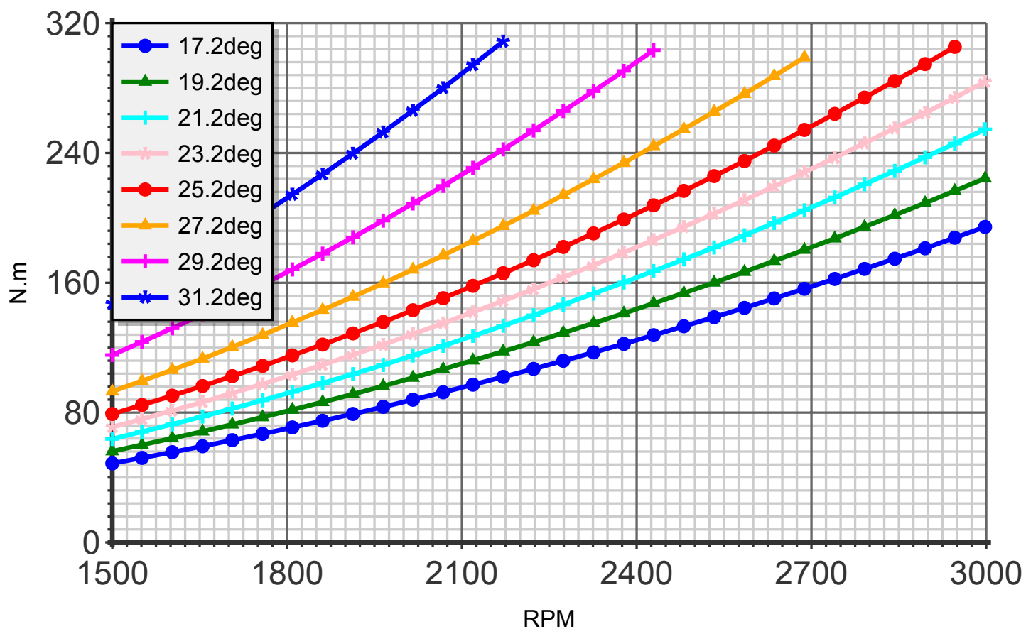
Torque (blade:2 diameter:165cm C4)
