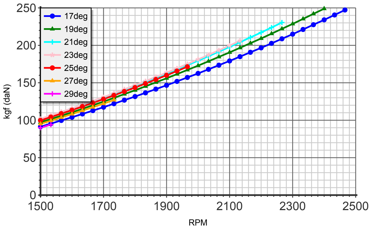
Thrust (blade:2 diameter:200cm C4)
