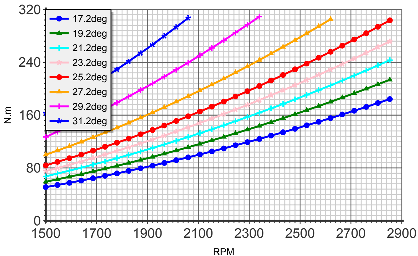
Torque (blade:2 diameter:172cm C4)
