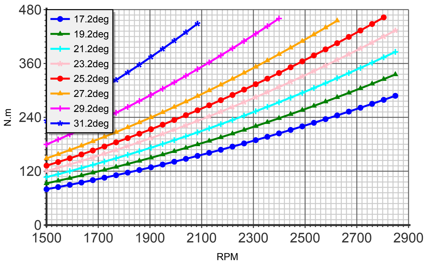
Torque (blade:3 diameter:175cm C4)
