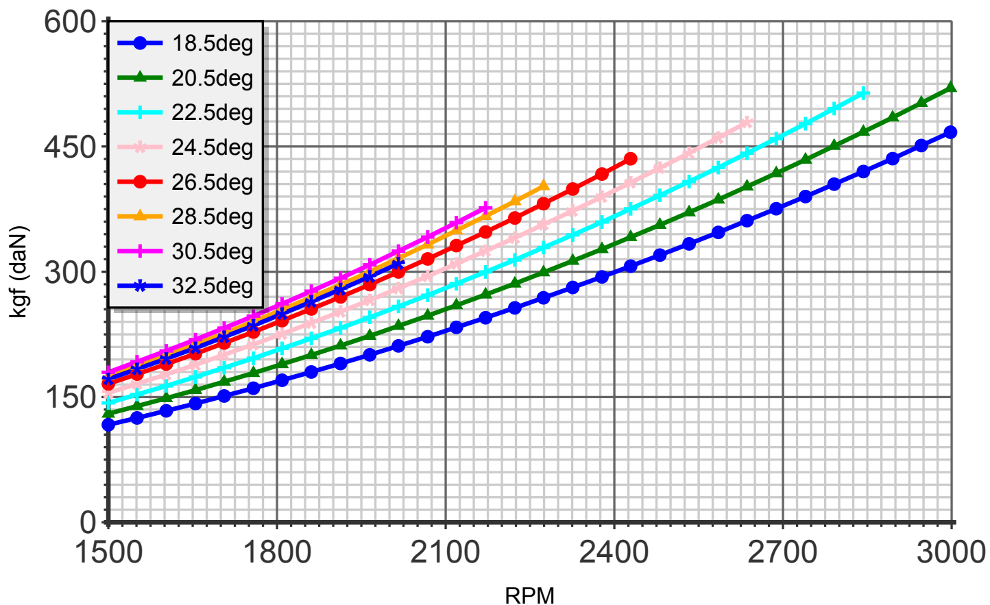
Thrust (blade:5 diameter:164cm C8)
