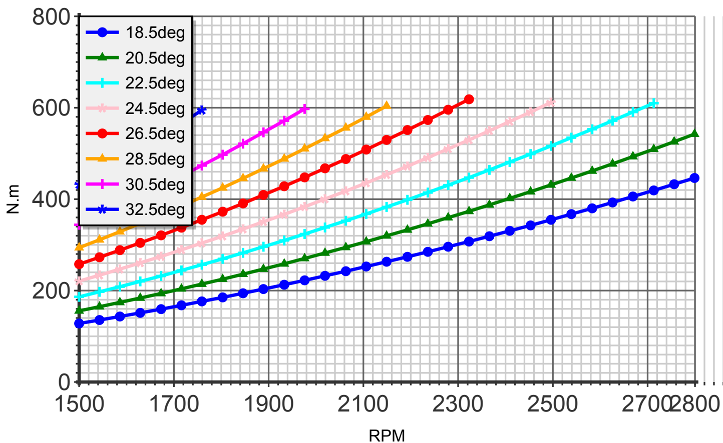
Torque (blade:4 diameter:177cm C8)
