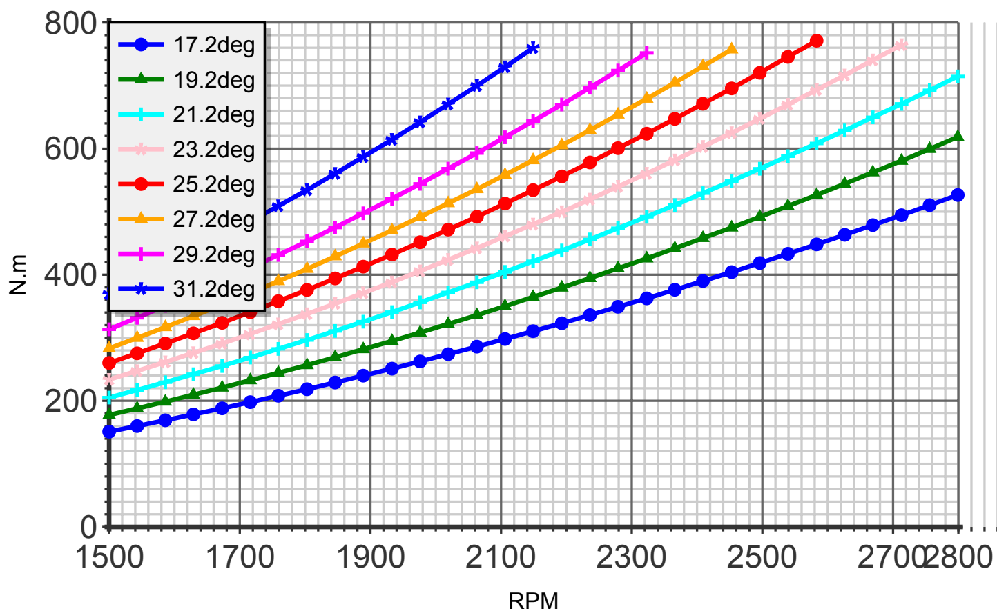
Torque (blade:5 diameter:179cm C4)
