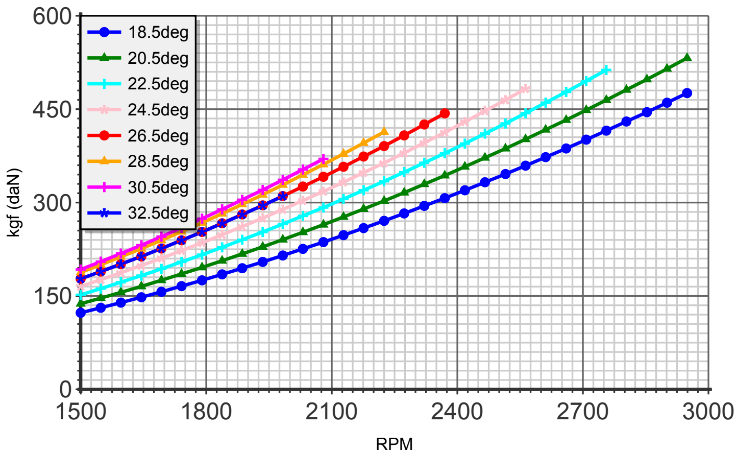
Thrust (blade:5 diameter:169cm C8)
