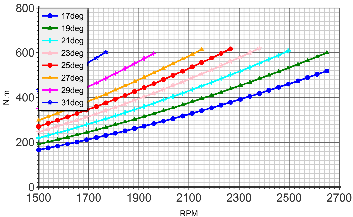
Torque (blade:4 diameter:187cm C4)
