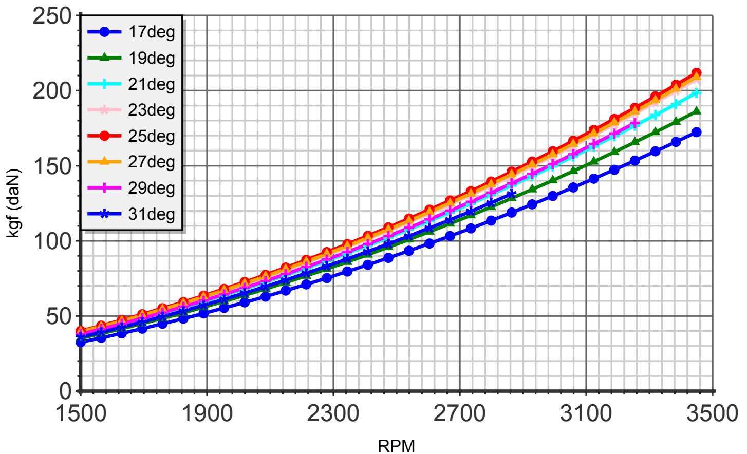
Thrust (blade:2 diameter:145cm C4)
