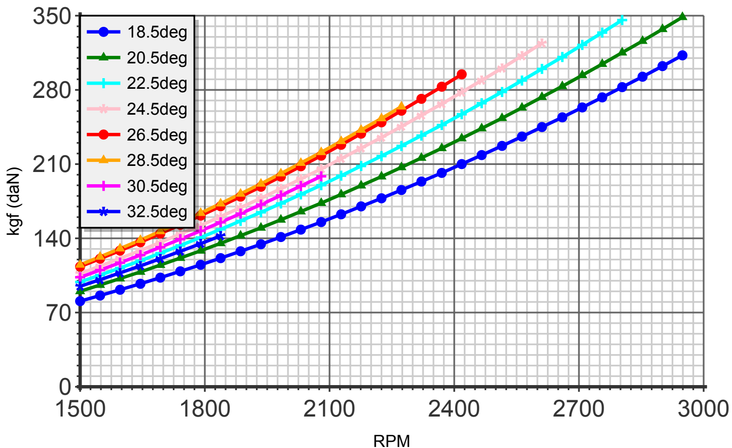
Thrust (blade:3 diameter:170cm C8)
