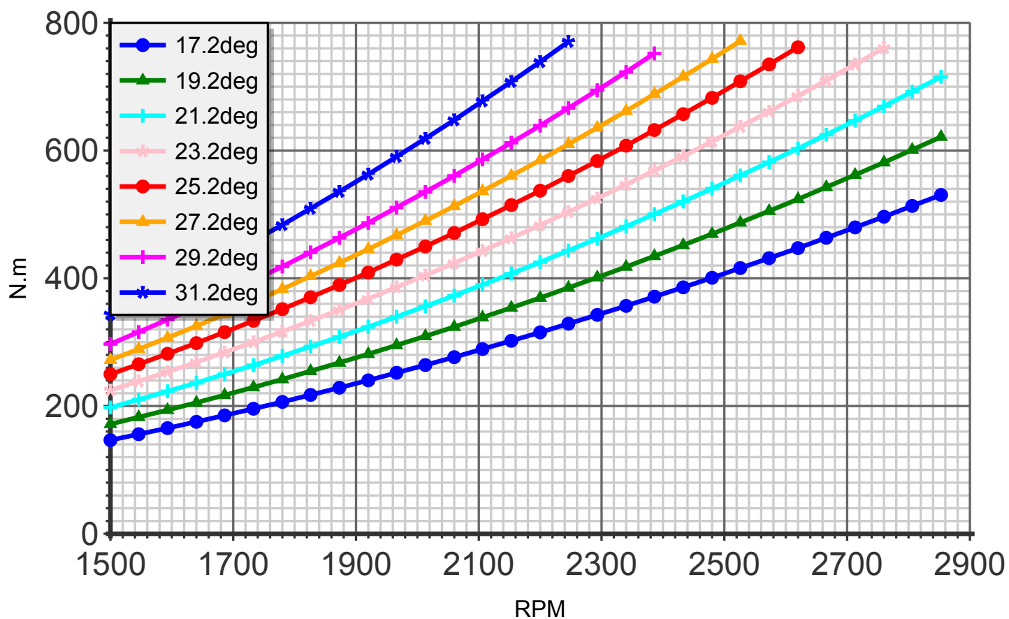
Torque (blade:5 diameter:174cm C4)
