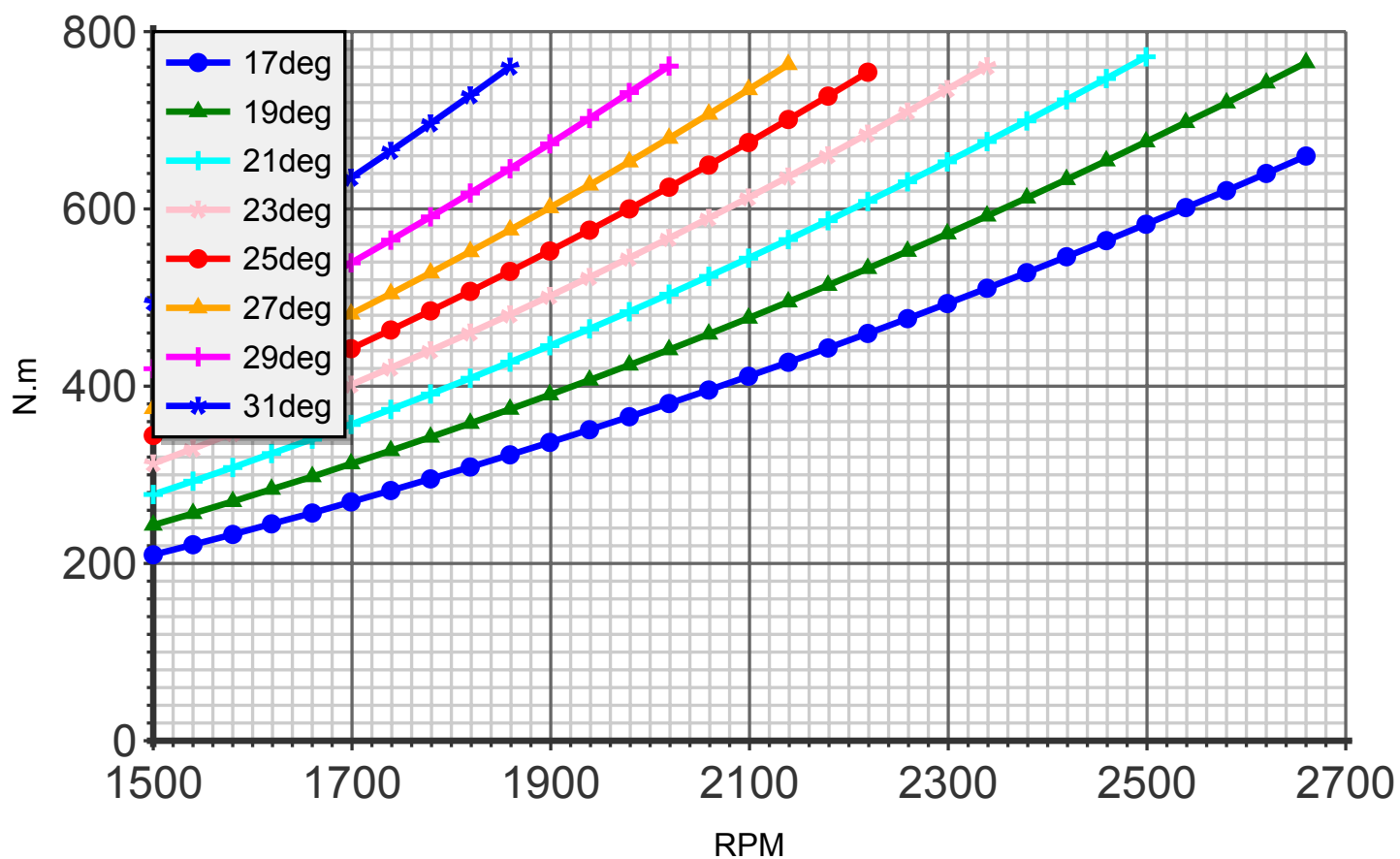
Torque (blade:5 diameter:184cm C4)
