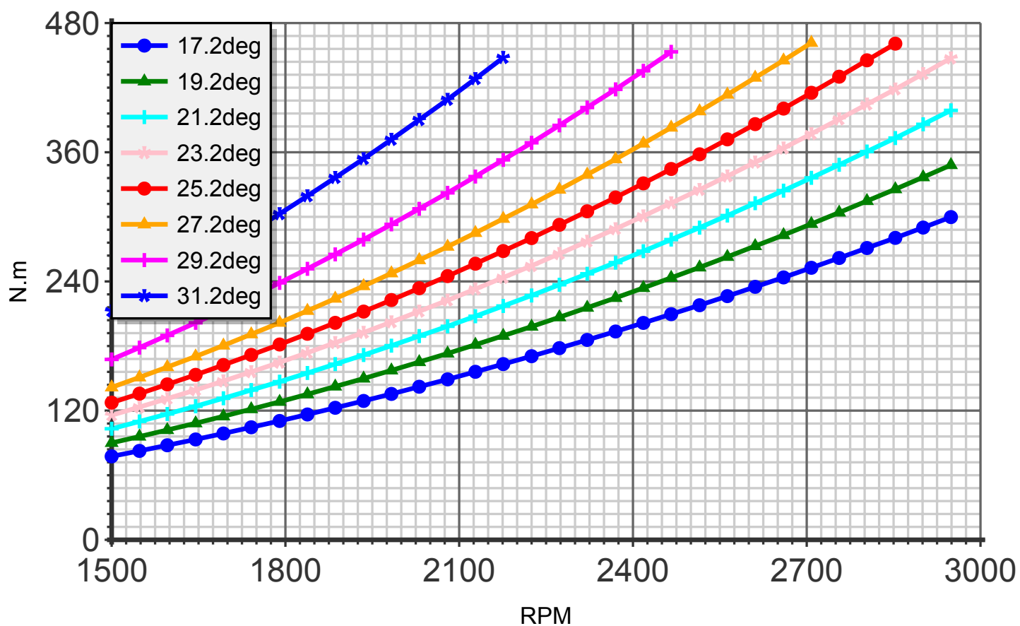
Torque (blade:3 diameter:170cm C4)
