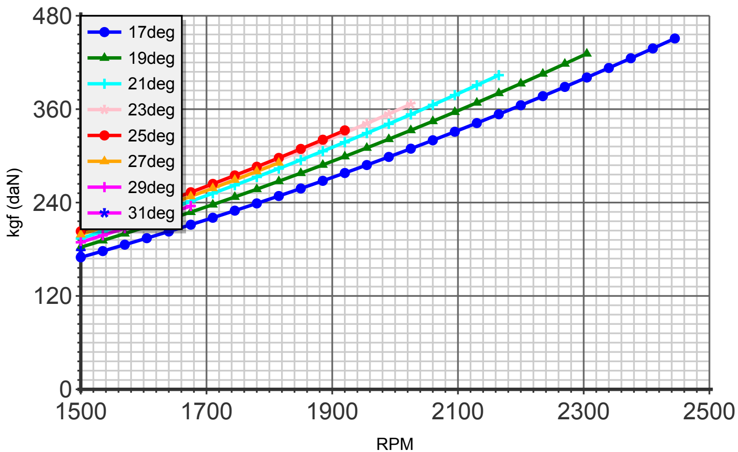
Thrust (blade:4 diameter:198cm C4)
