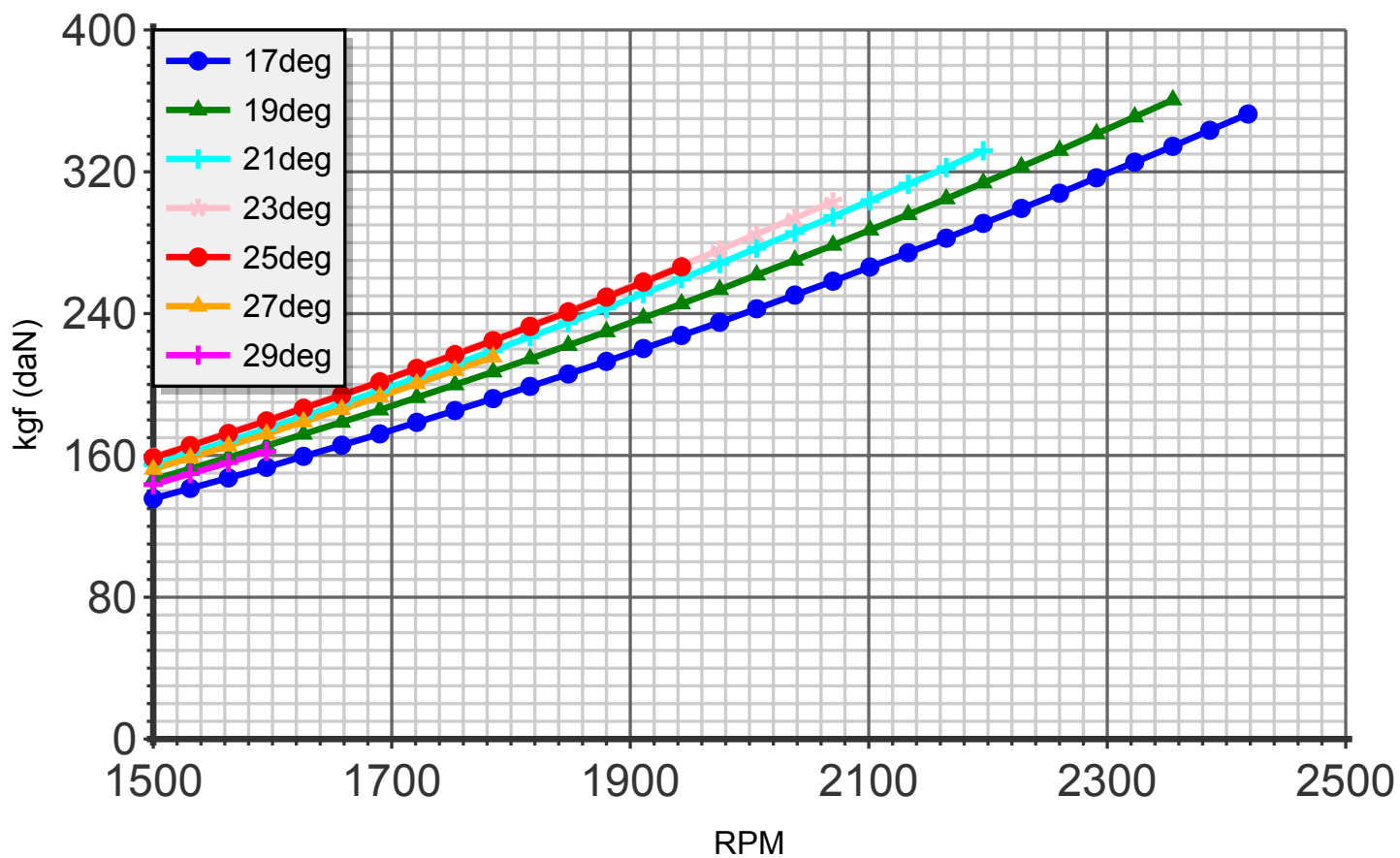
Thrust (blade:3 diameter:205cm C4)
