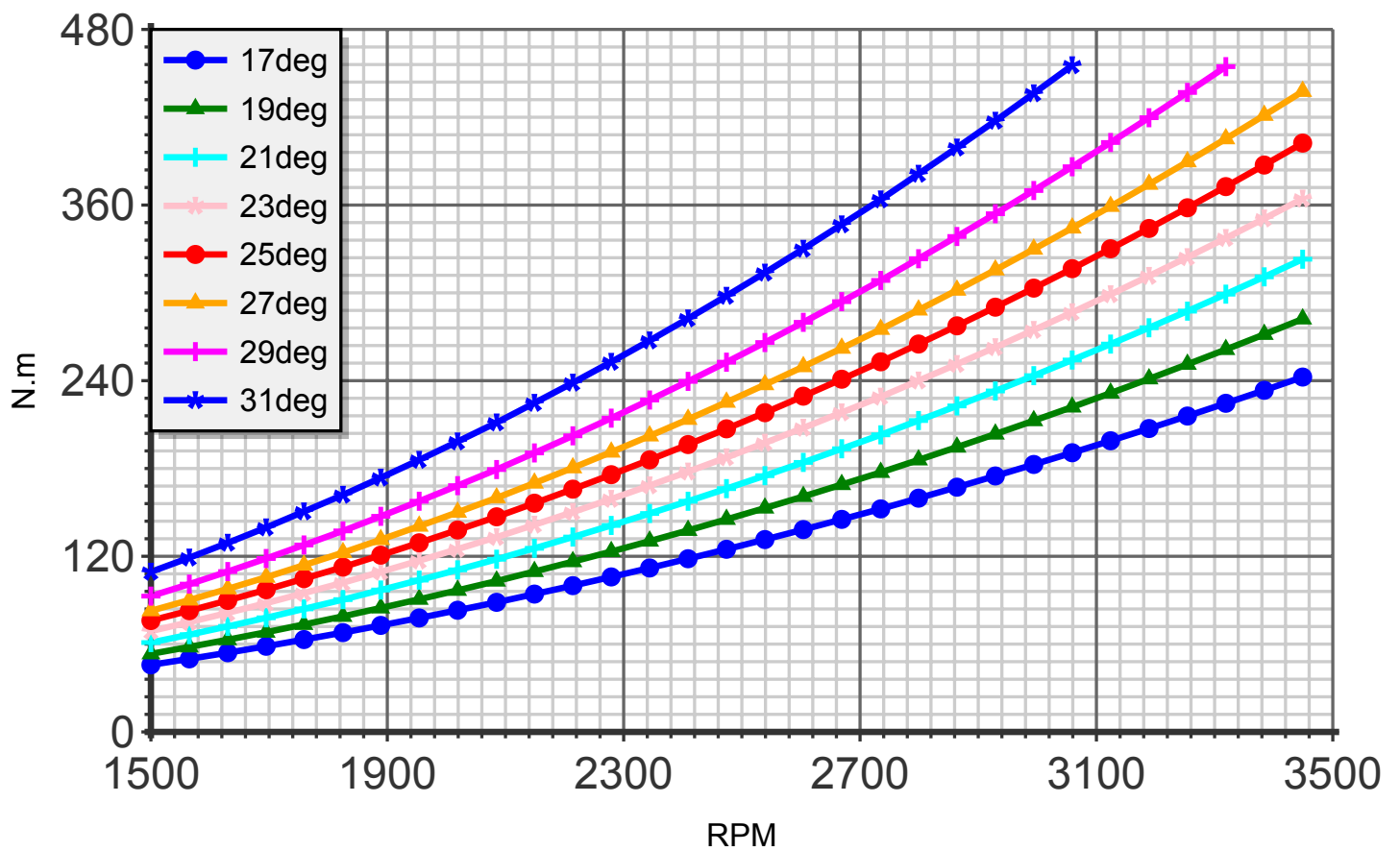
Torque (blade:3 diameter:145cm C4)
