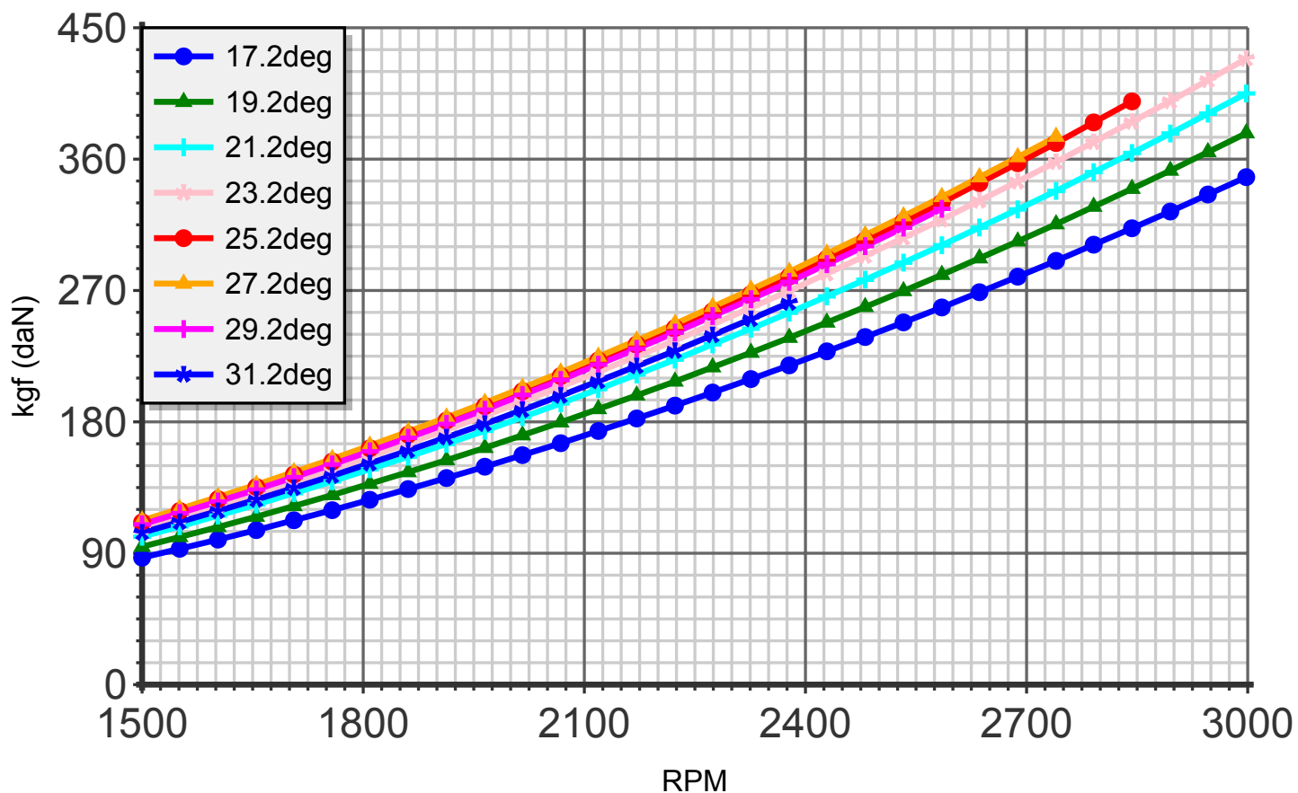
Thrust (blade:4 diameter:162cm C4)
