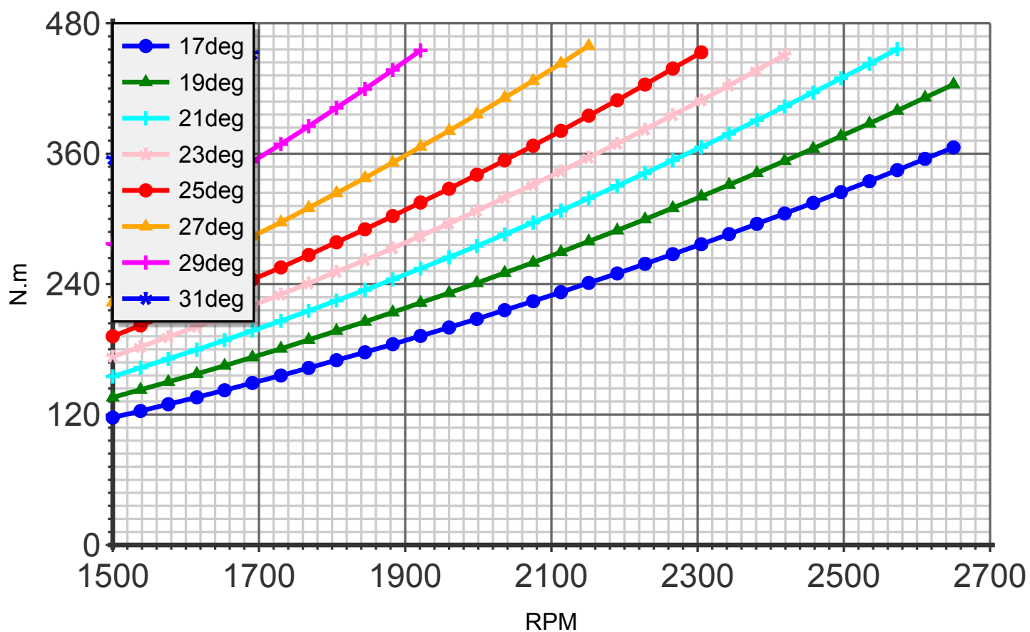
Torque (blade:3 diameter:190cm C4)
