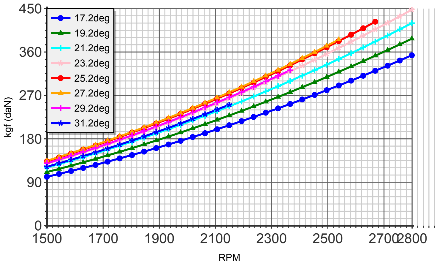
Thrust (blade:4 diameter:177cm C4)
