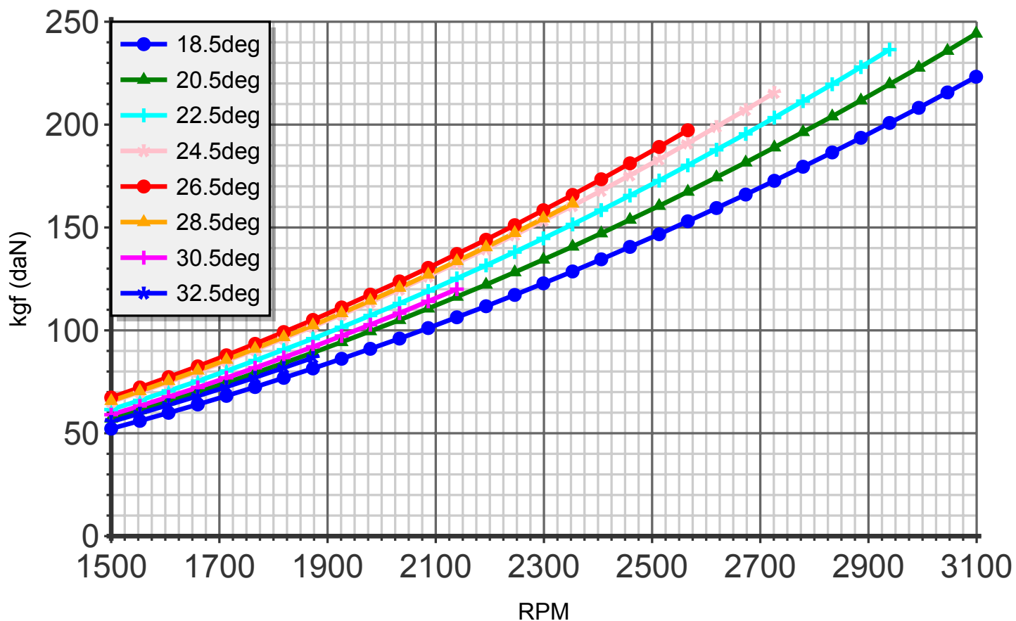
Thrust (blade:2 diameter:160cm C8)
