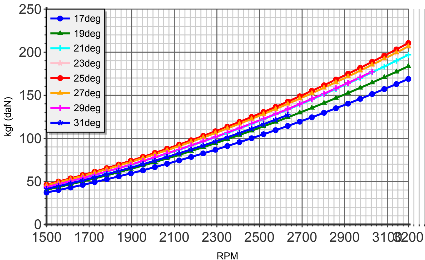
Thrust (blade:2 diameter:155cm C4)
