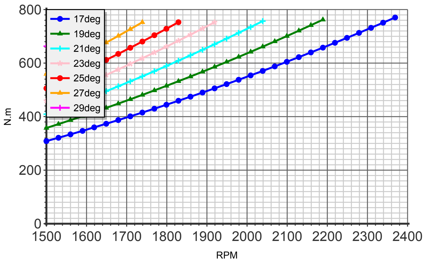
Torque (blade:5 diameter:209cm C4)
