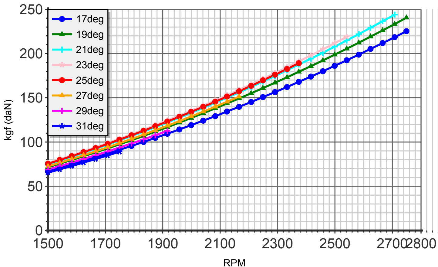
Thrust (blade:2 diameter:180cm C4)
