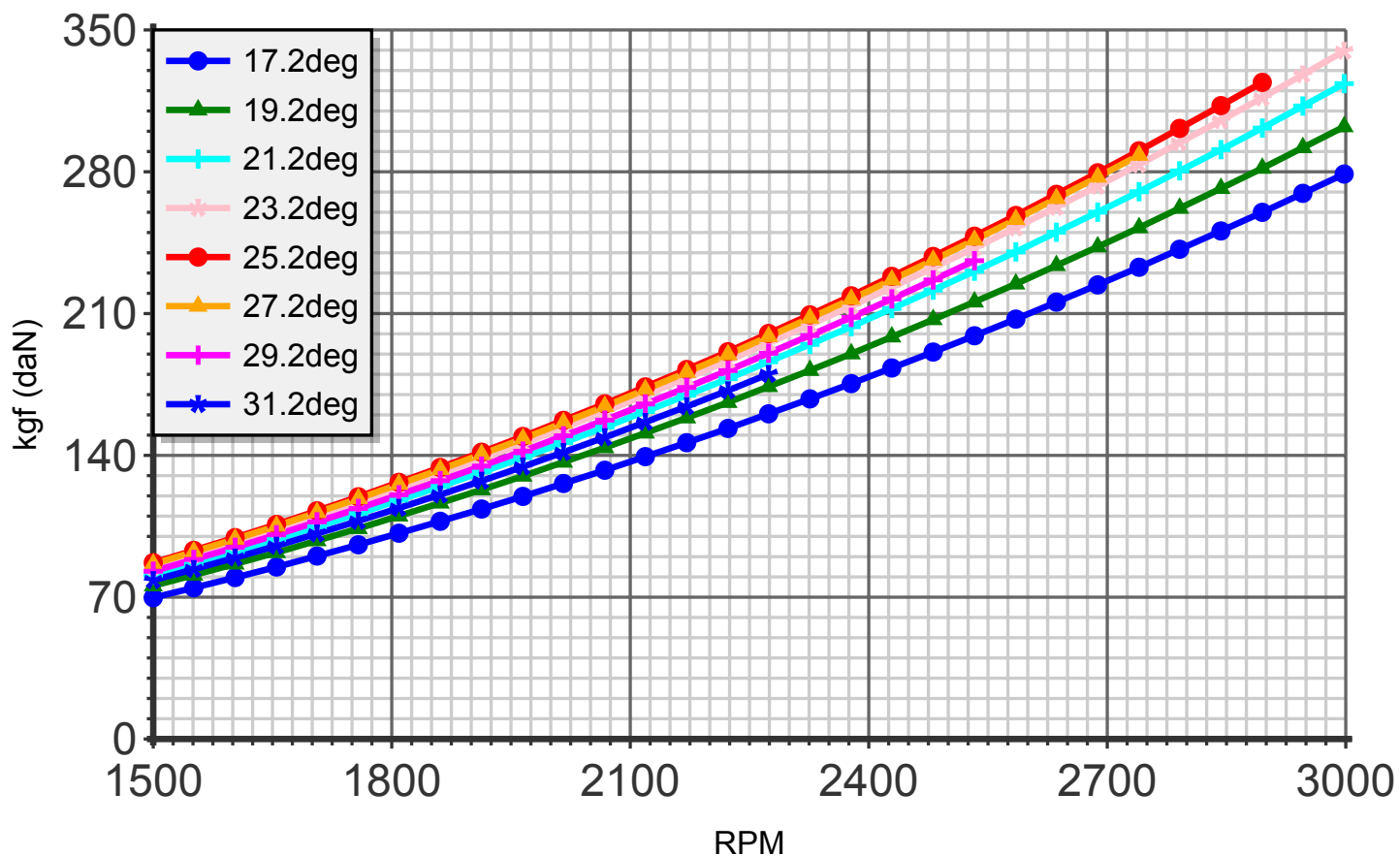
Thrust (blade:3 diameter:165cm C4)
