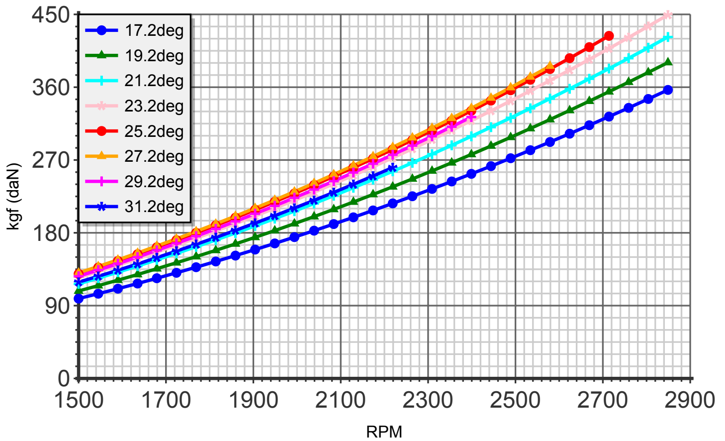
Thrust (blade:4 diameter:174cm C4)
