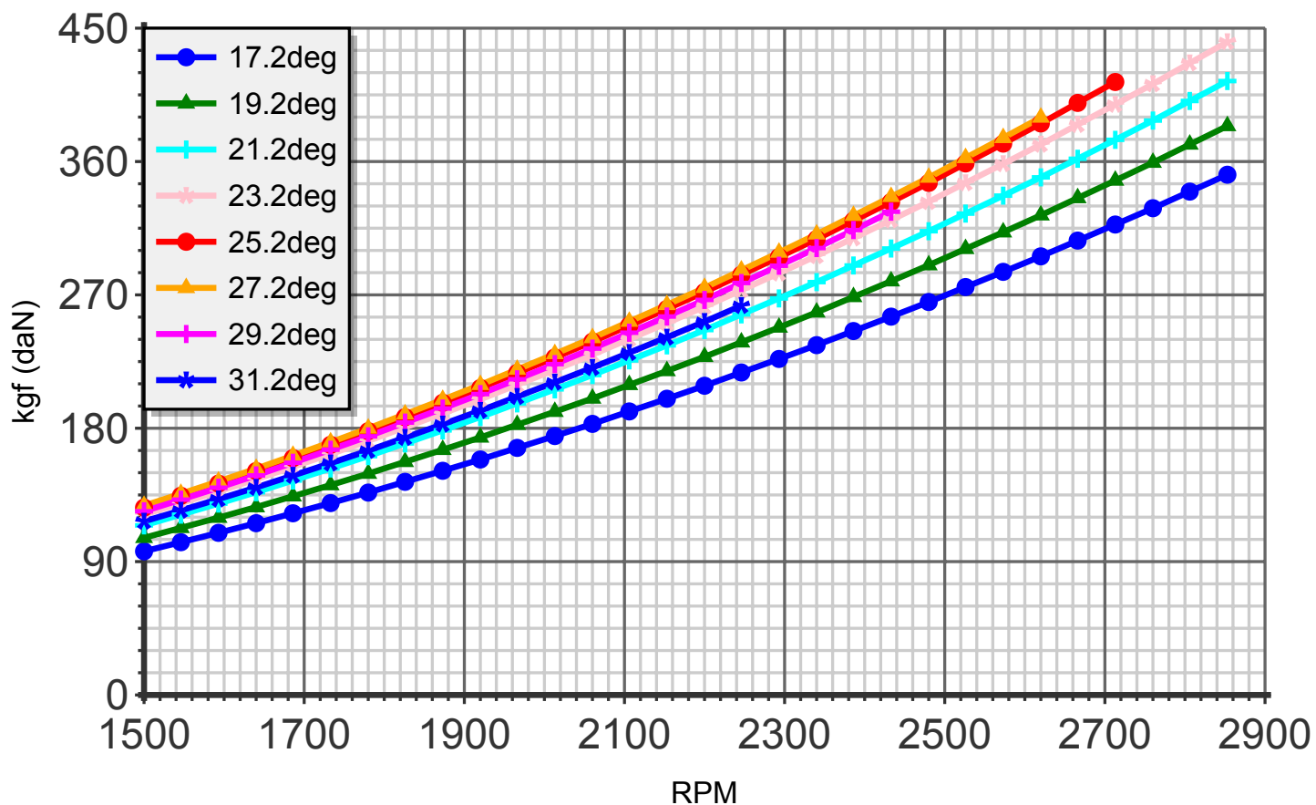
Thrust (blade:4 diameter:172cm C4)
