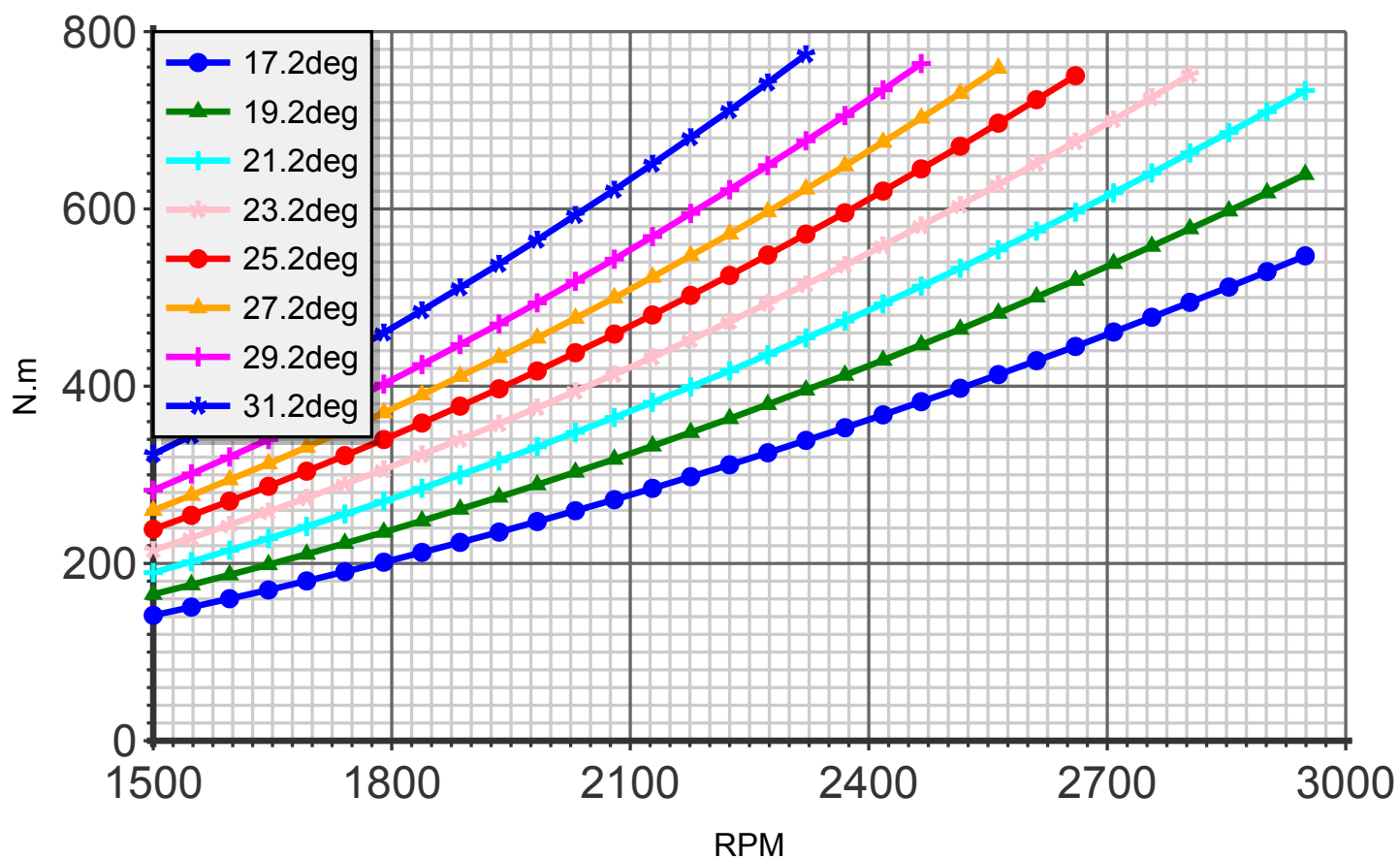
Torque (blade:5 diameter:169cm C4)
