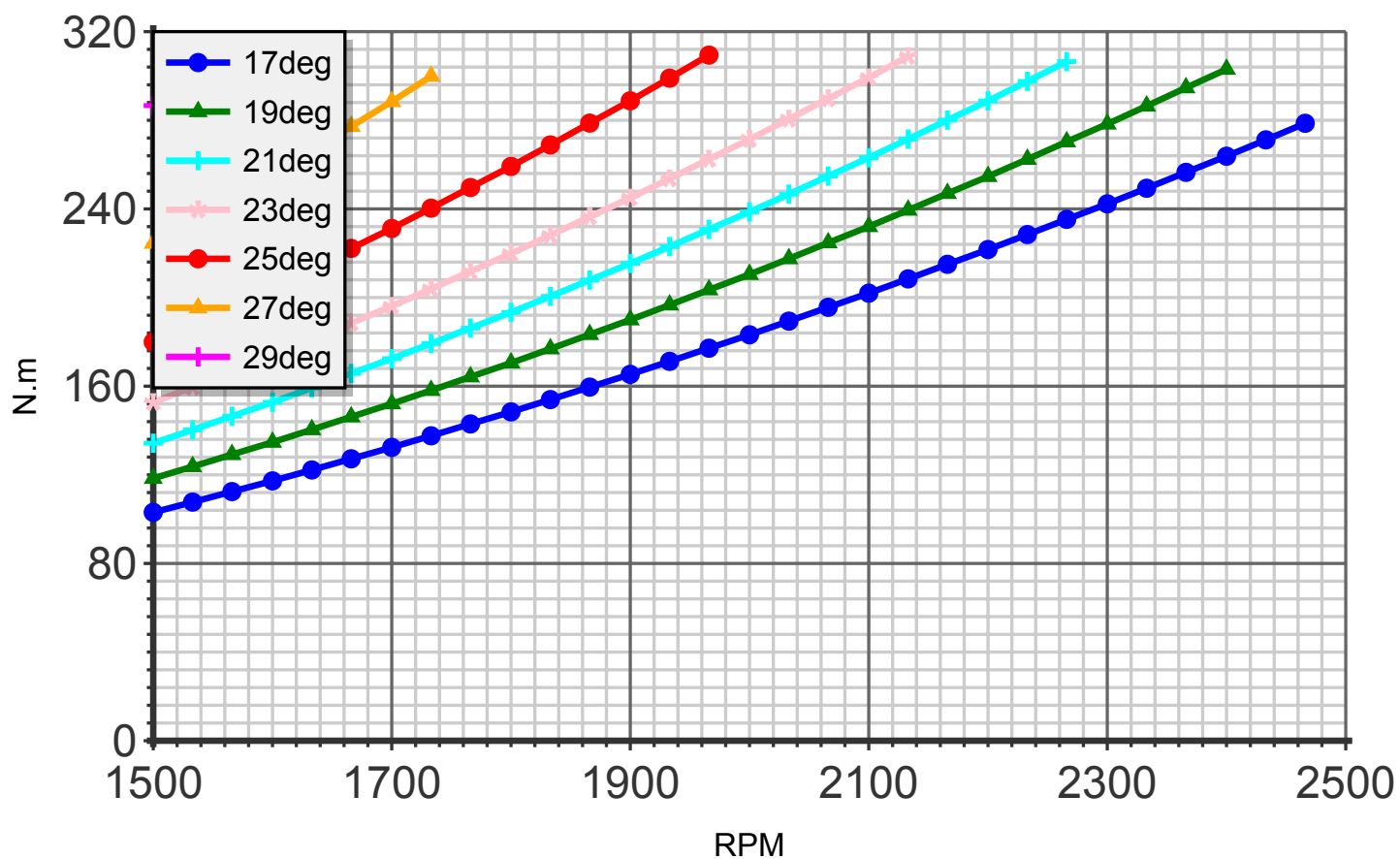
Torque (blade:2 diameter:200cm C4)
