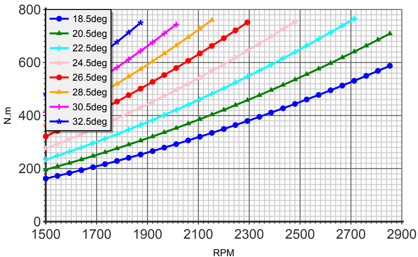
Torque (blade:5 diameter:174cm C8)
