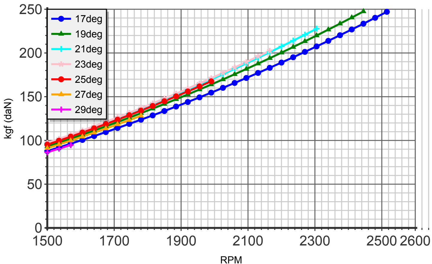
Thrust (blade:2 diameter:195cm C4)
