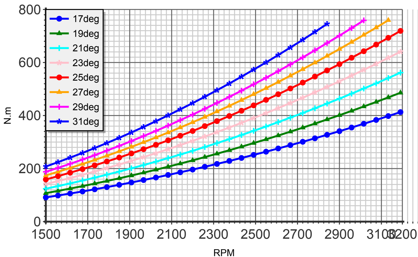
Torque (blade:5 diameter:154cm C4)
