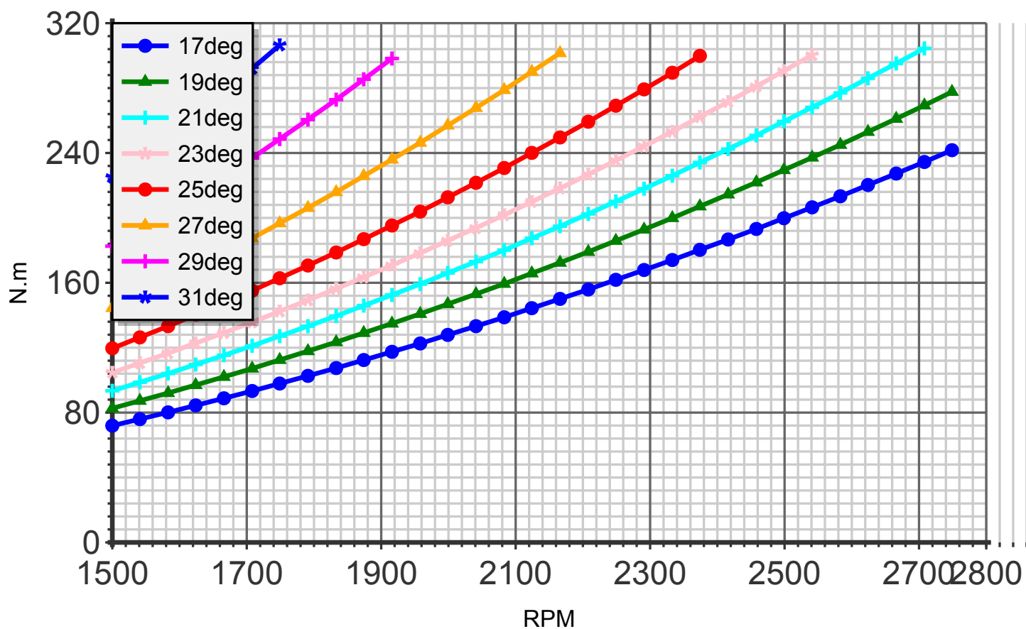
Torque (blade:2 diameter:180cm C4)
