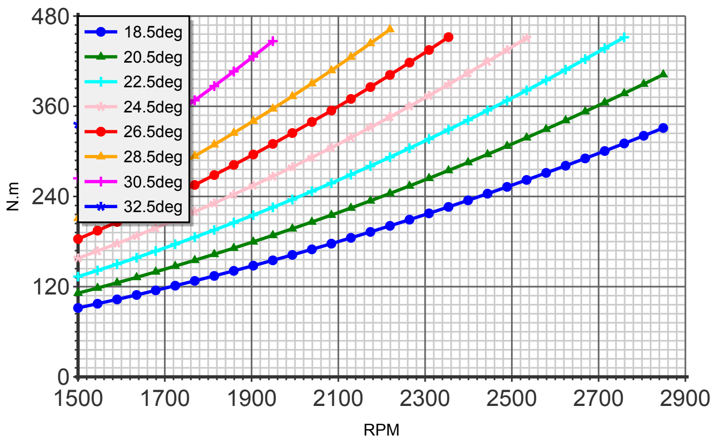
Torque (blade:3 diameter:175cm C8)
