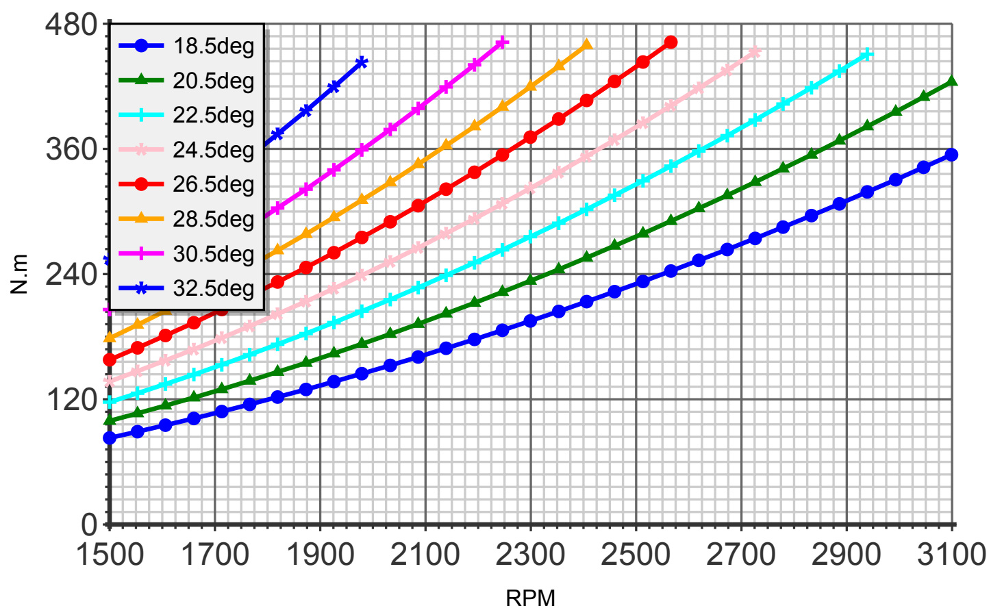
Torque (blade:3 diameter:160cm C8)
