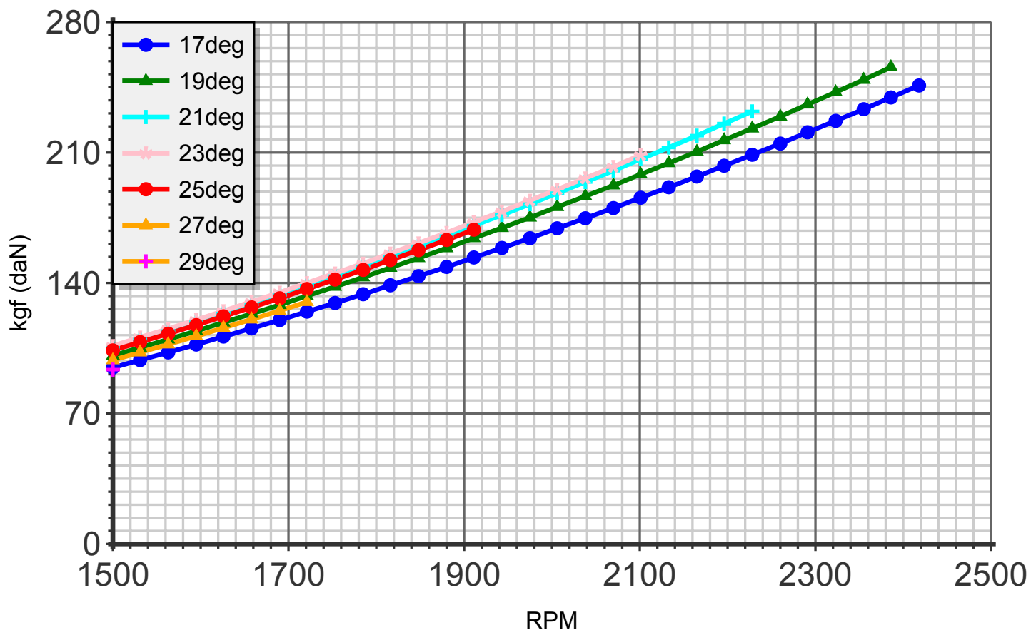
Thrust (blade:2 diameter:205cm C4)
