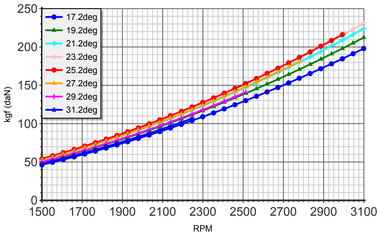
Thrust (blade:2 diameter:160cm C4)
