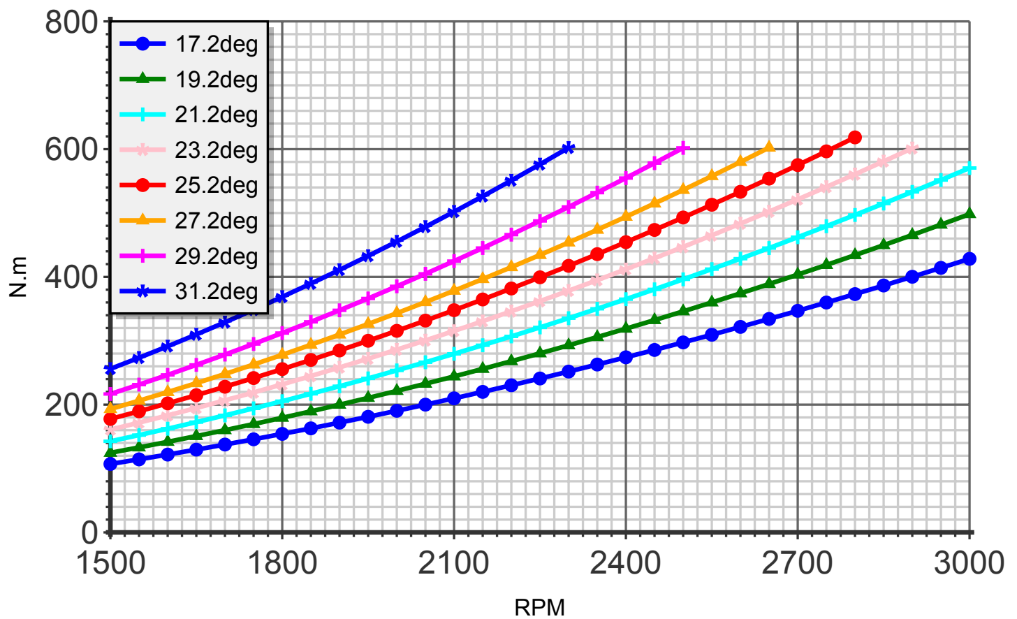
Torque (blade:4 diameter:167cm C4)
