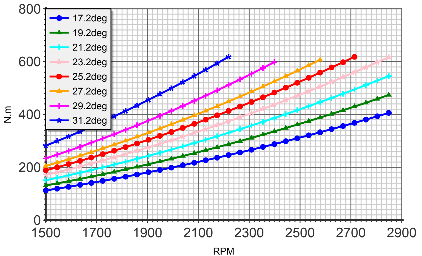
Torque (blade:4 diameter:174cm C4)
