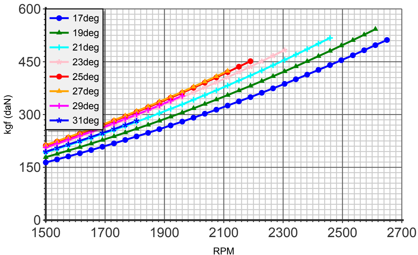
Thrust (blade:5 diameter:189cm C4)
