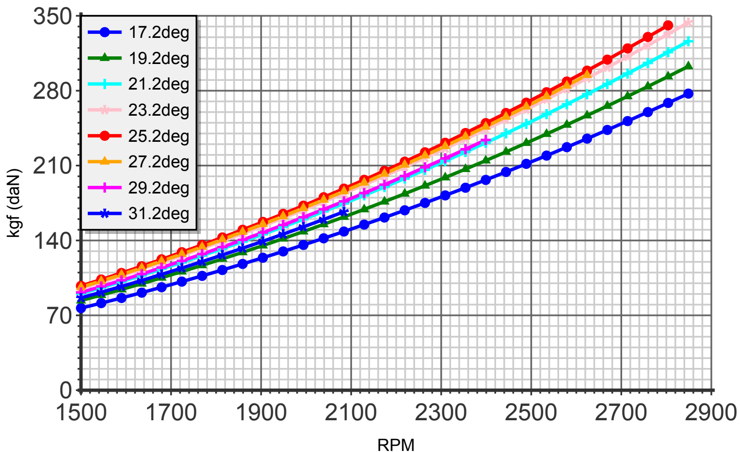
Thrust (blade:3 diameter:175cm C4)
