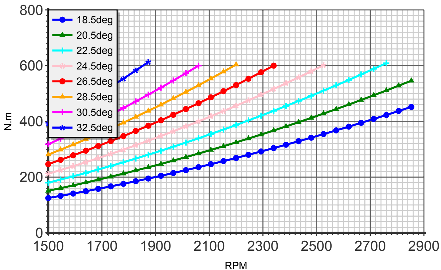
Torque (blade:4 diameter:172cm C8)
