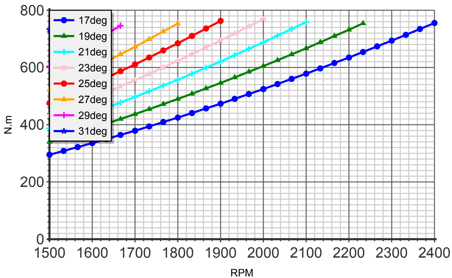
Torque (blade:5 diameter:199cm C4)
