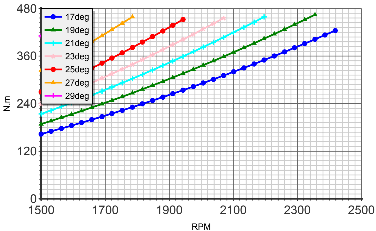
Torque (blade:3 diameter:205cm C4)
