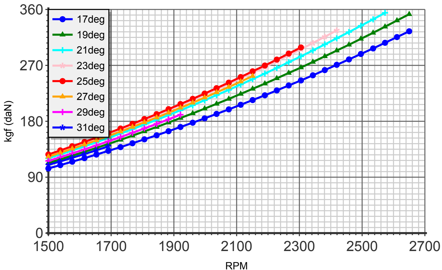
Thrust (blade:3 diameter:190cm C4)
