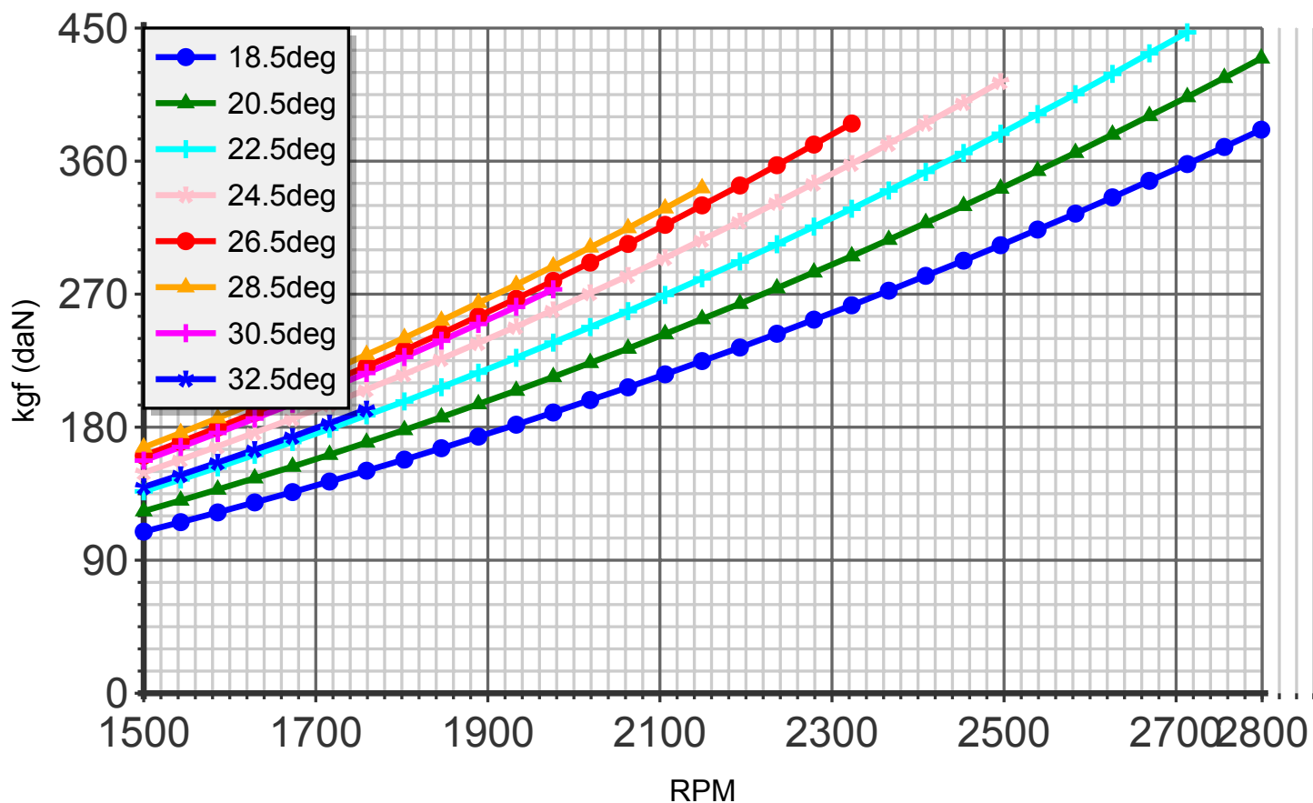
Thrust (blade:4 diameter:177cm C8)
