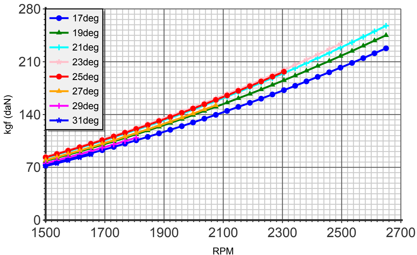
Thrust (blade:2 diameter:190cm C4)
