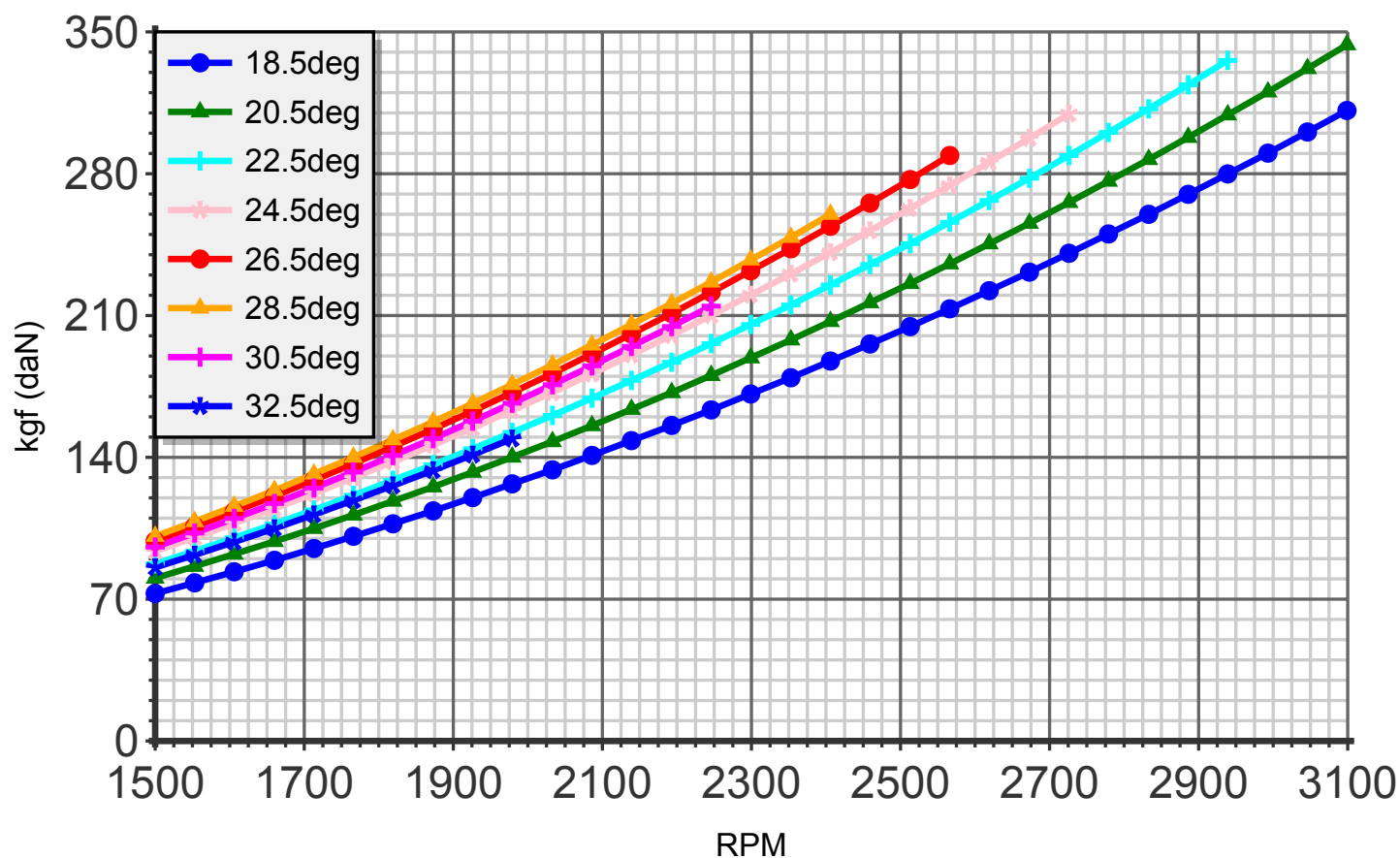
Thrust (blade:3 diameter:160cm C8)
