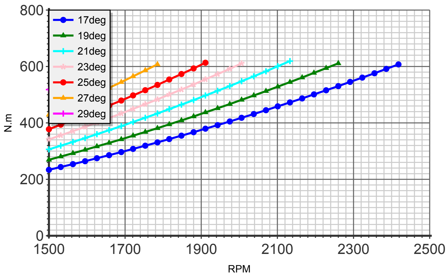
Torque (blade:4 diameter:203cm C4)
