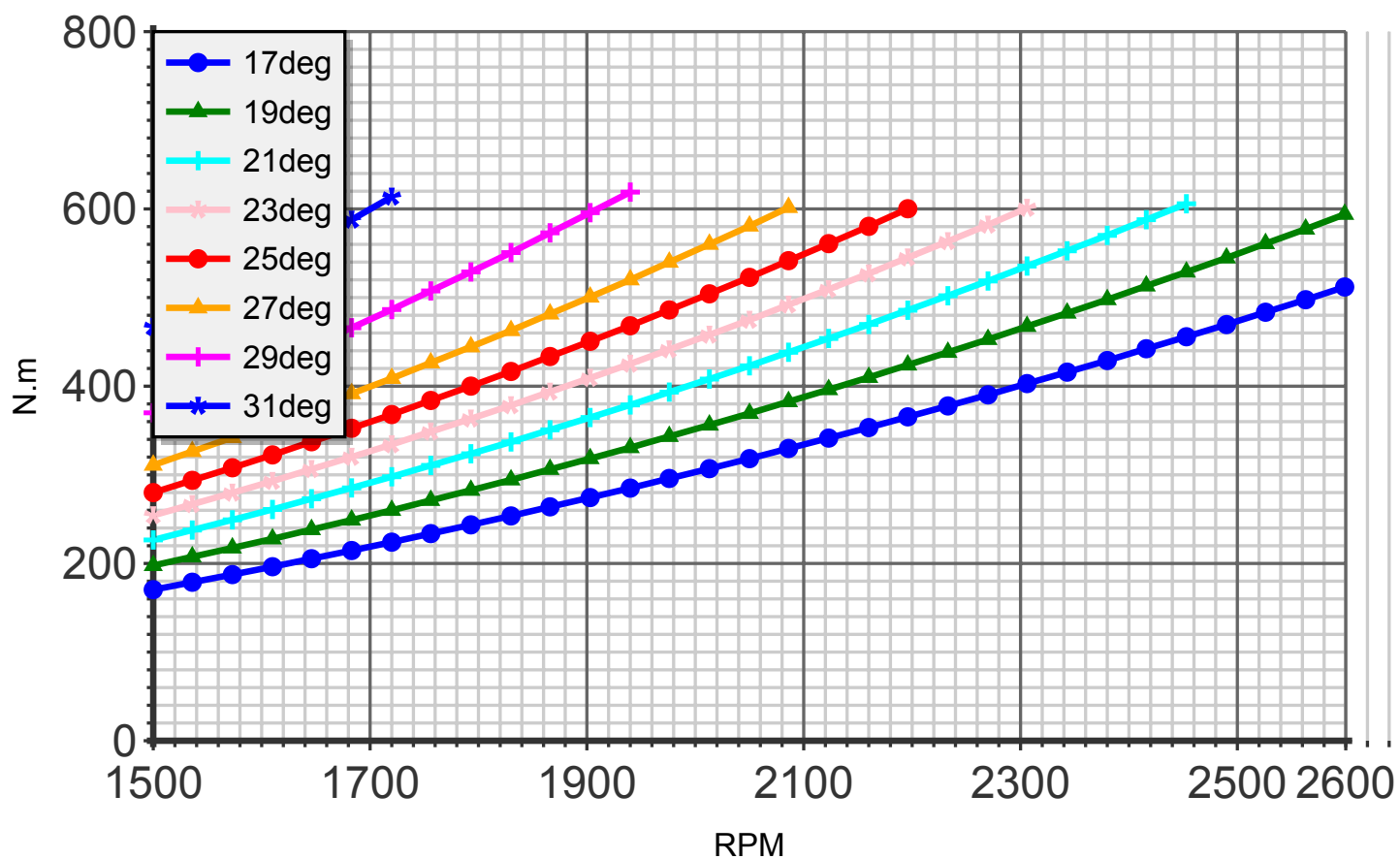
Torque (blade:4 diameter:192cm C4)
