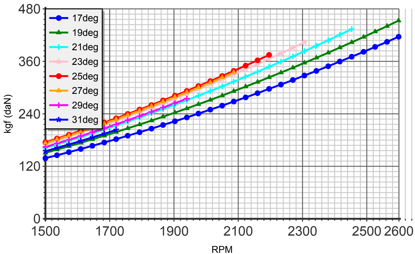
Thrust (blade:4 diameter:192cm C4)
