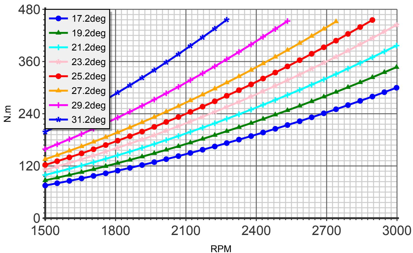
Torque (blade:3 diameter:165cm C4)
