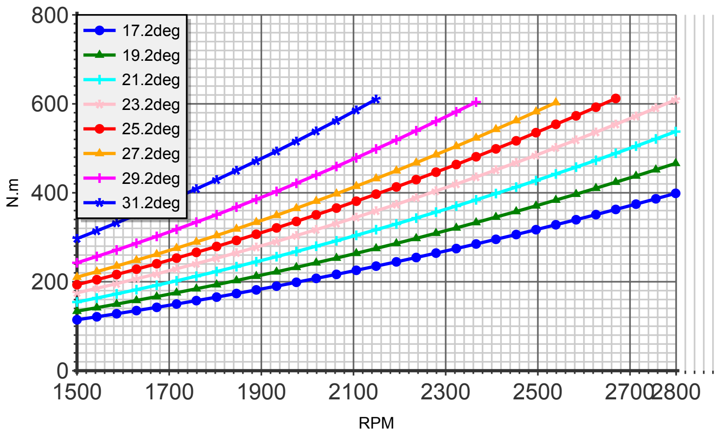
Torque (blade:4 diameter:177cm C4)
