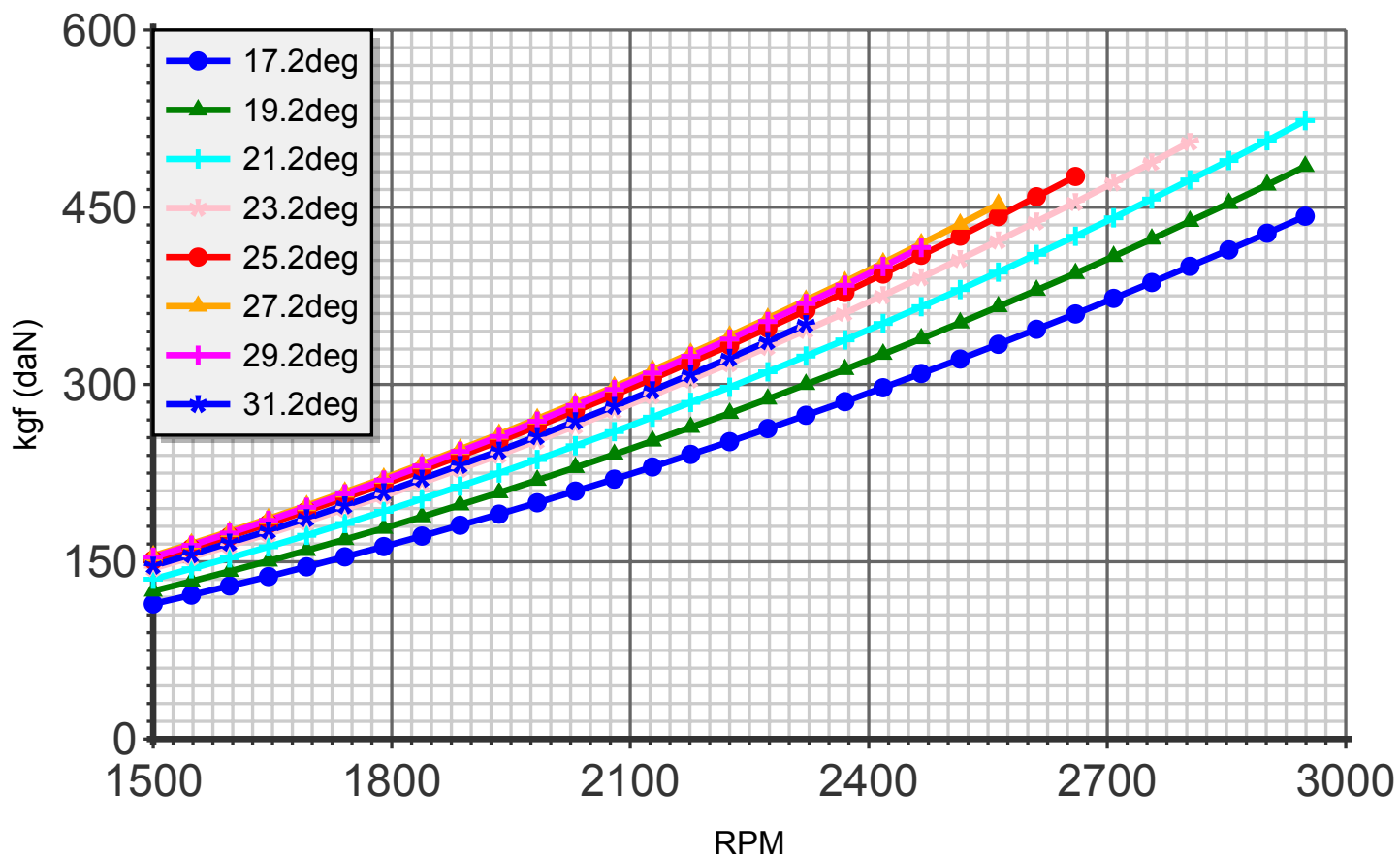
Thrust (blade:5 diameter:169cm C4)
