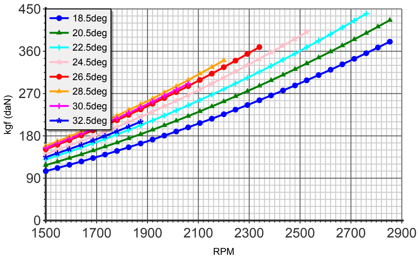
Thrust (blade:4 diameter:172cm C8)
