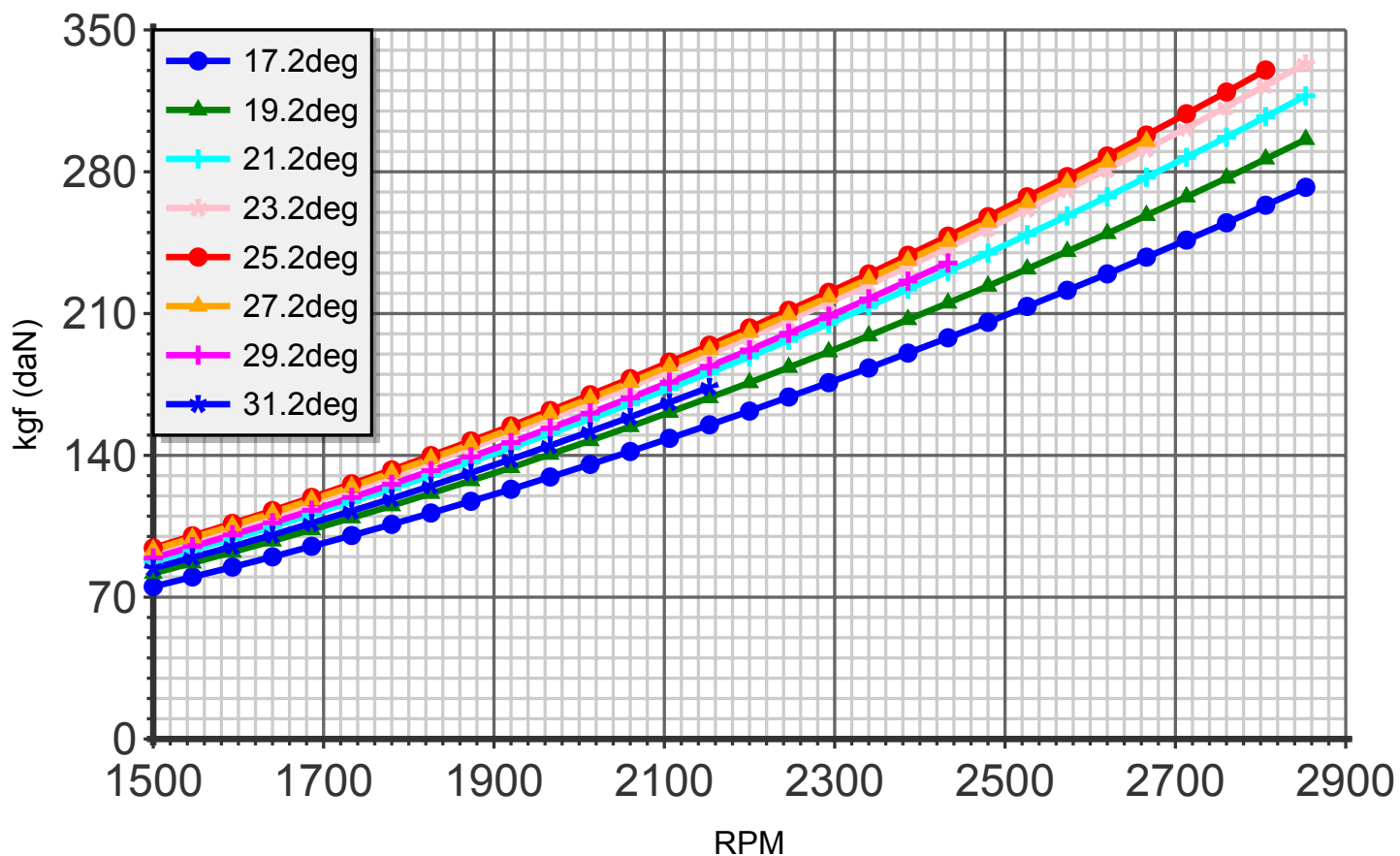
Thrust (blade:3 diameter:172cm C4)
