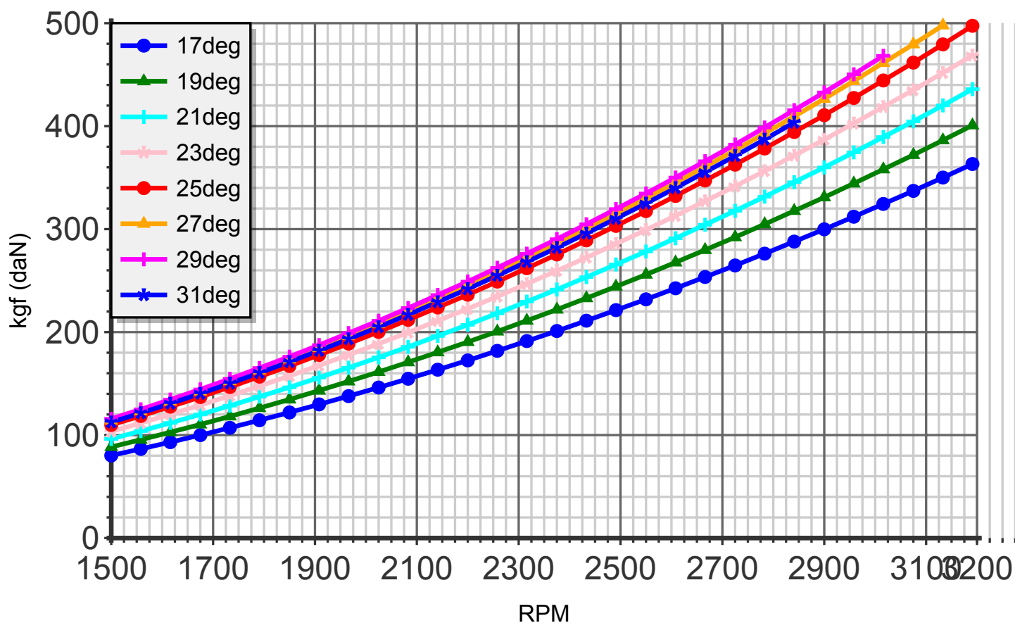
Thrust (blade:5 diameter:154cm C4)
