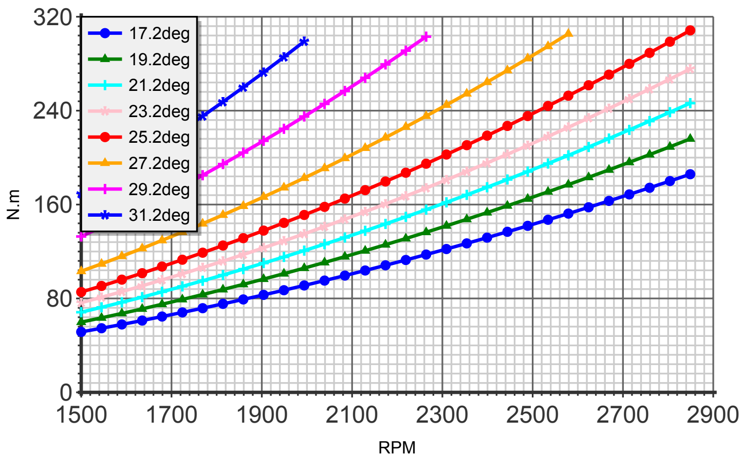
Torque (blade:2 diameter:175cm C4)
