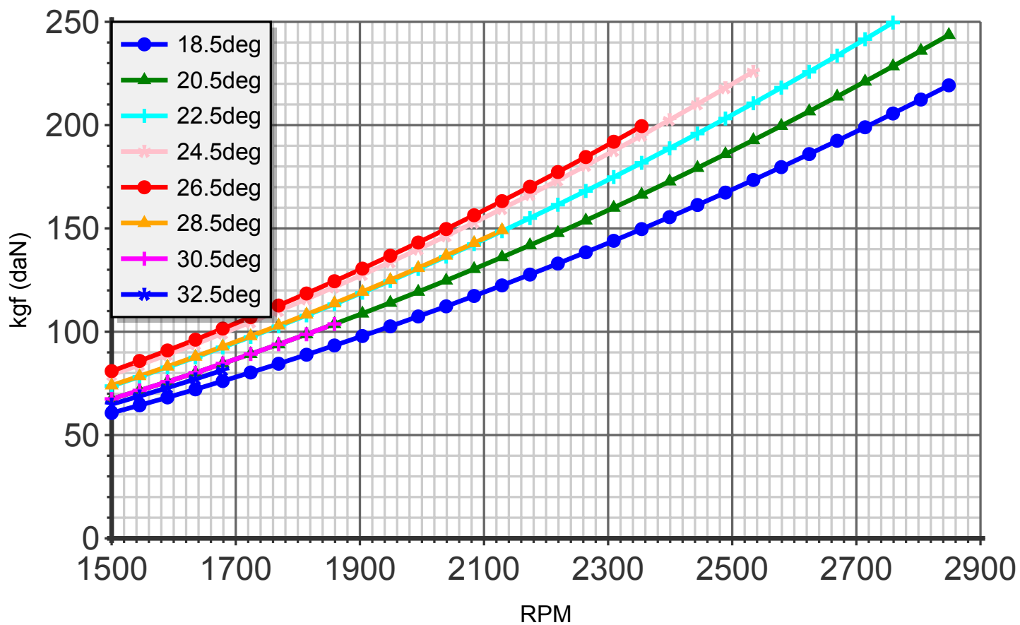
Thrust (blade:2 diameter:175cm C8)
