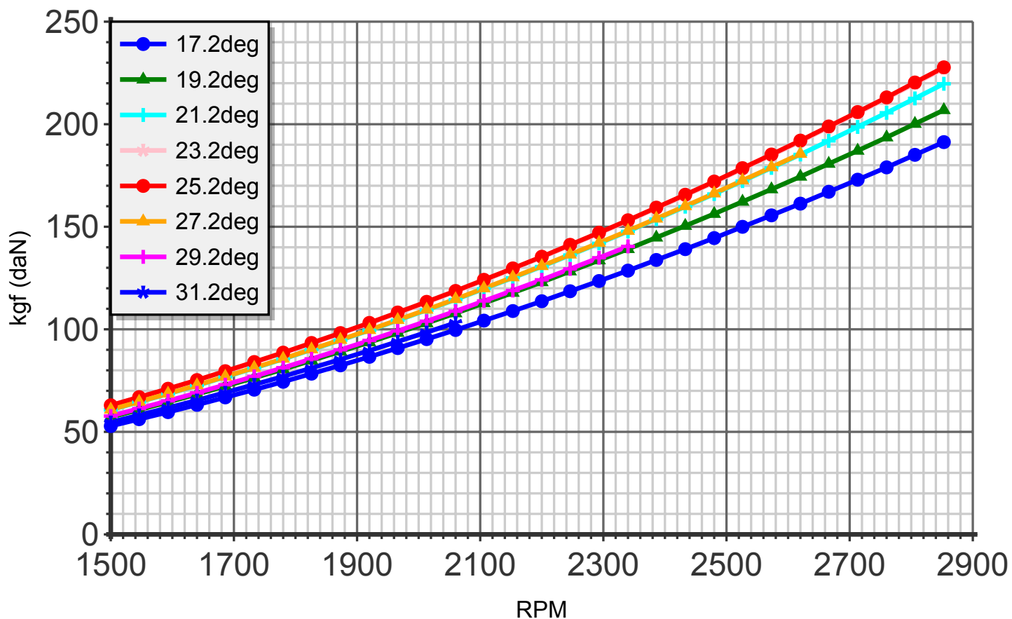
Thrust (blade:2 diameter:172cm C4)
