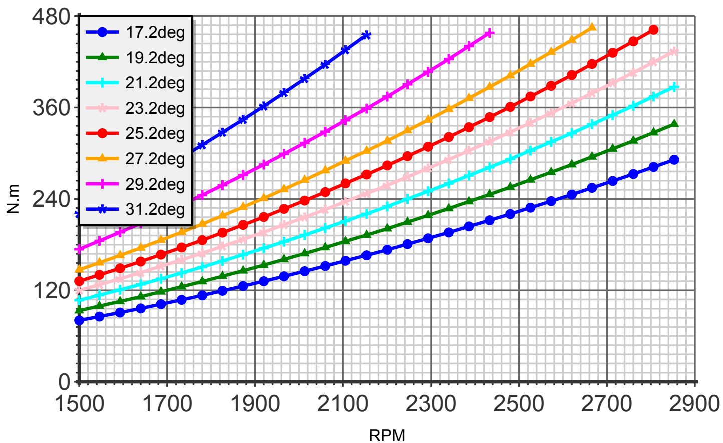
Torque (blade:3 diameter:172cm C4)
