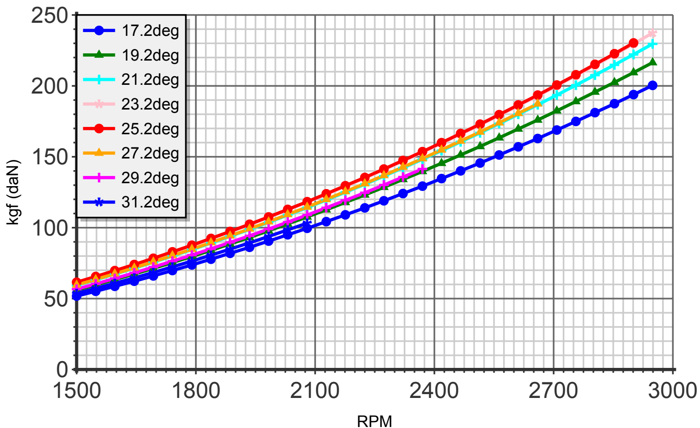
Thrust (blade:2 diameter:170cm C4)
