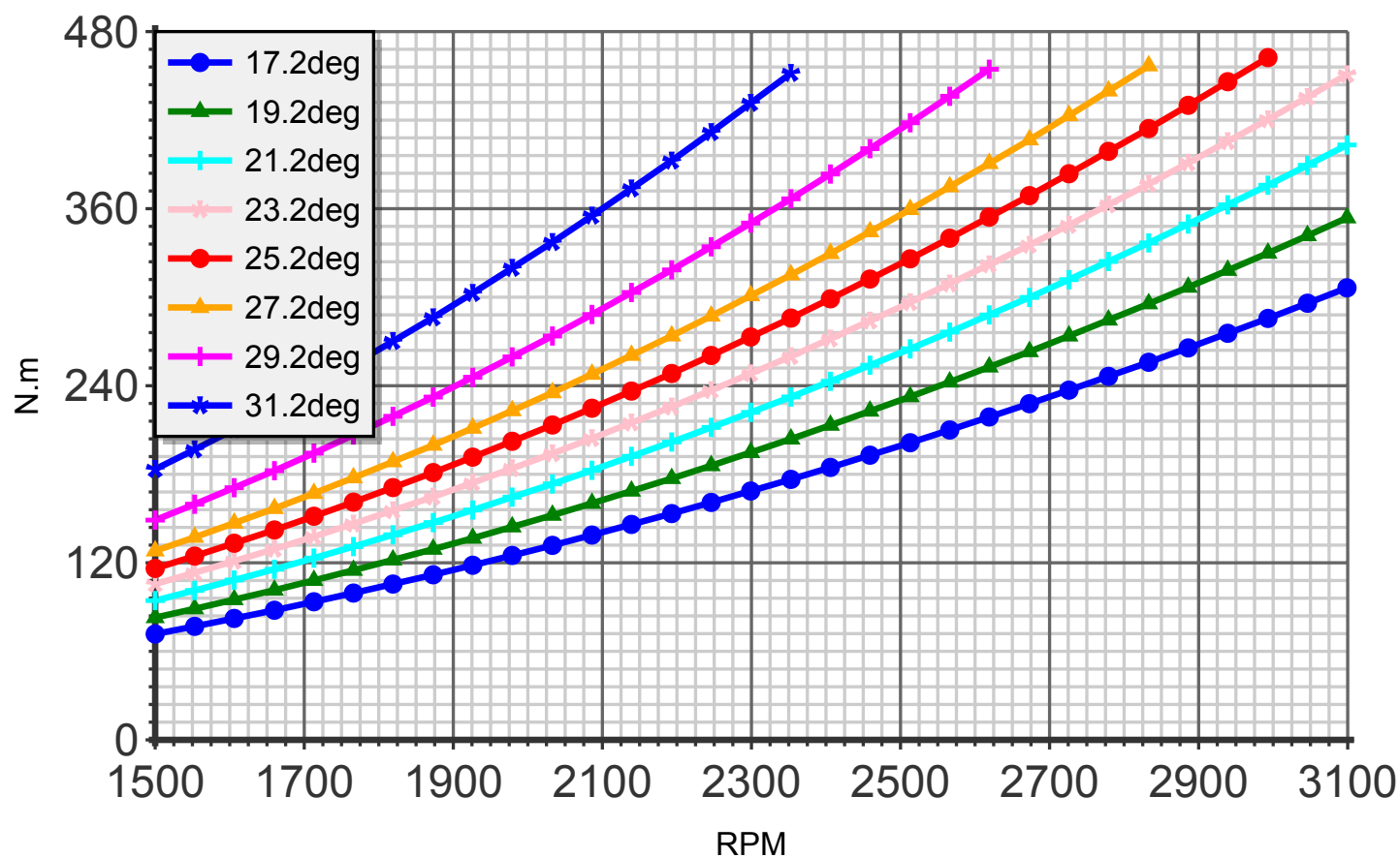
Torque (blade:3 diameter:160cm C4)
