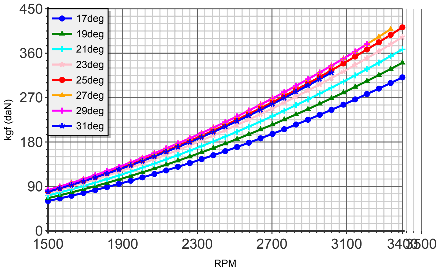
Thrust (blade:4 diameter:147cm C4)
