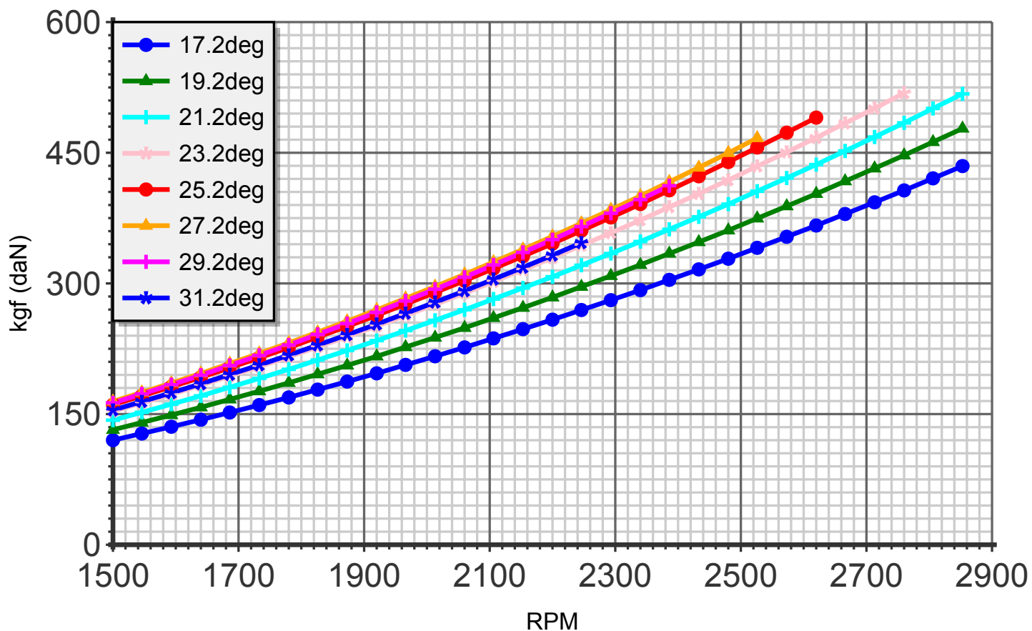
Thrust (blade:5 diameter:174cm C4)
