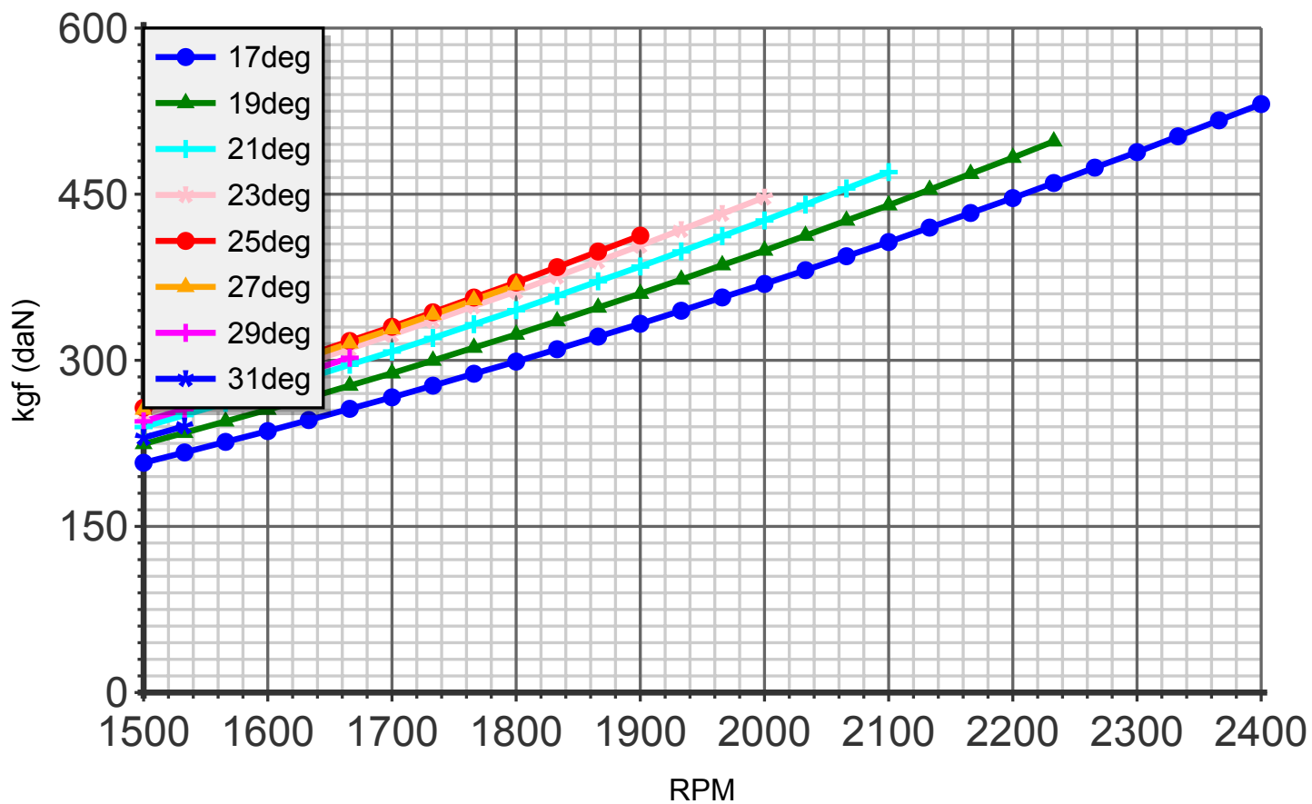
Thrust (blade:5 diameter:199cm C4)
