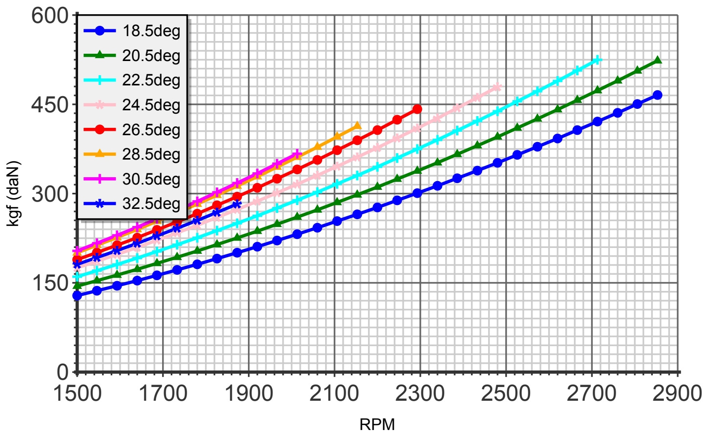
Thrust (blade:5 diameter:174cm C8)
