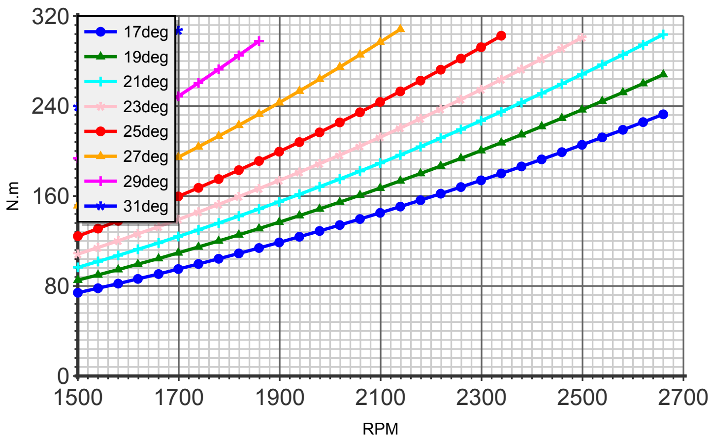
Torque (blade:2 diameter:185cm C4)
