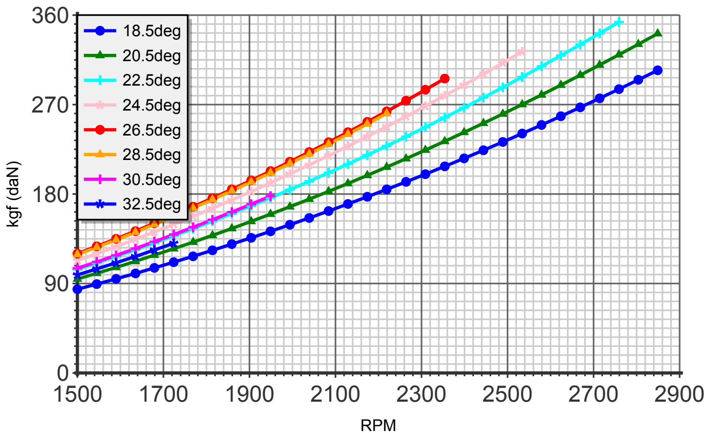
Thrust (blade:3 diameter:175cm C8)
