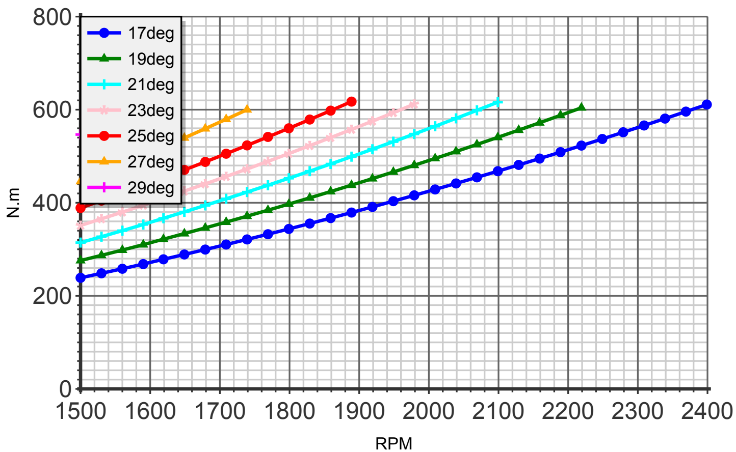
Torque (blade:4 diameter:208cm C4)
