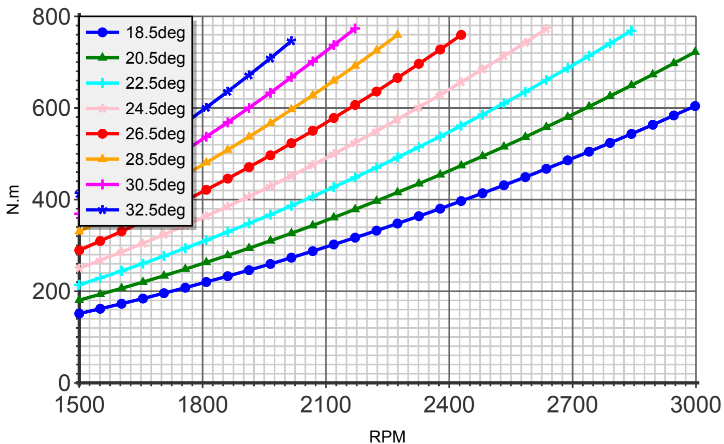
Torque (blade:5 diameter:164cm C8)
