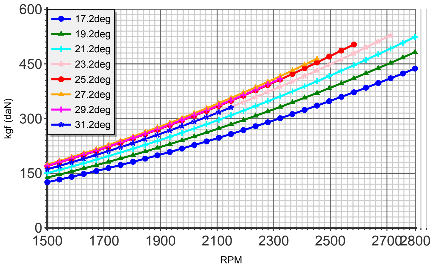
Thrust (blade:5 diameter:179cm C4)
