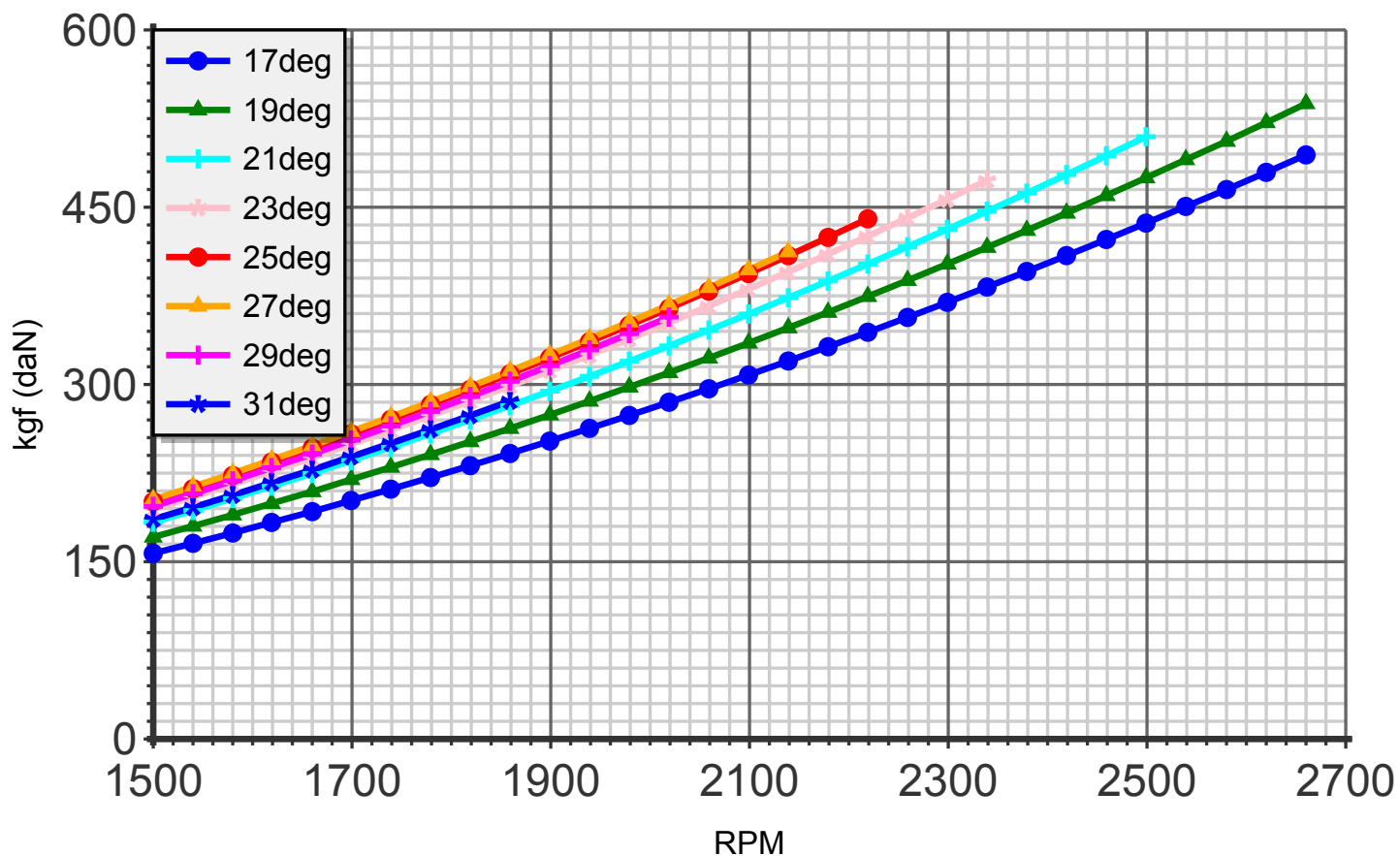
Thrust (blade:5 diameter:184cm C4)
