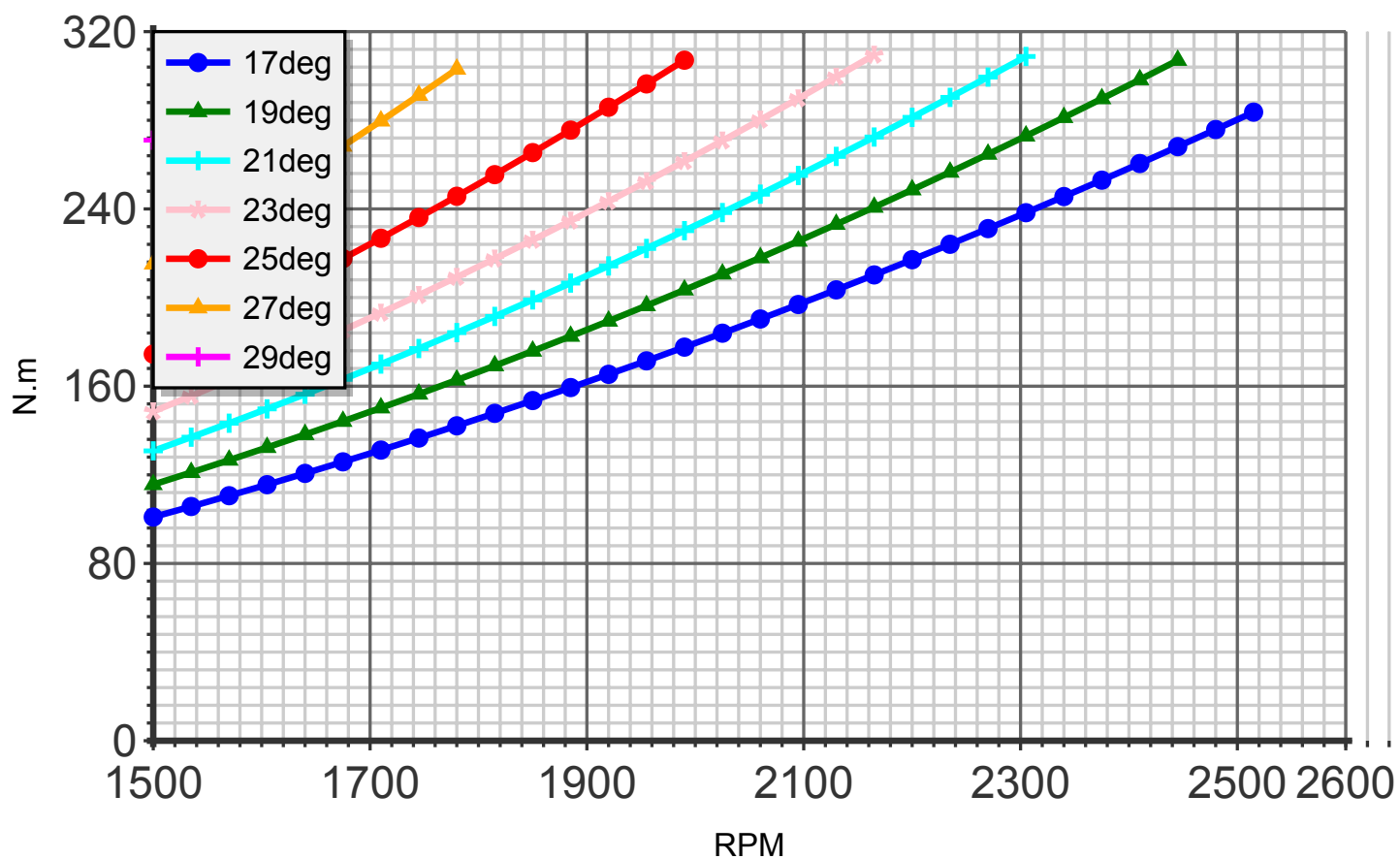
Torque (blade:2 diameter:195cm C4)
