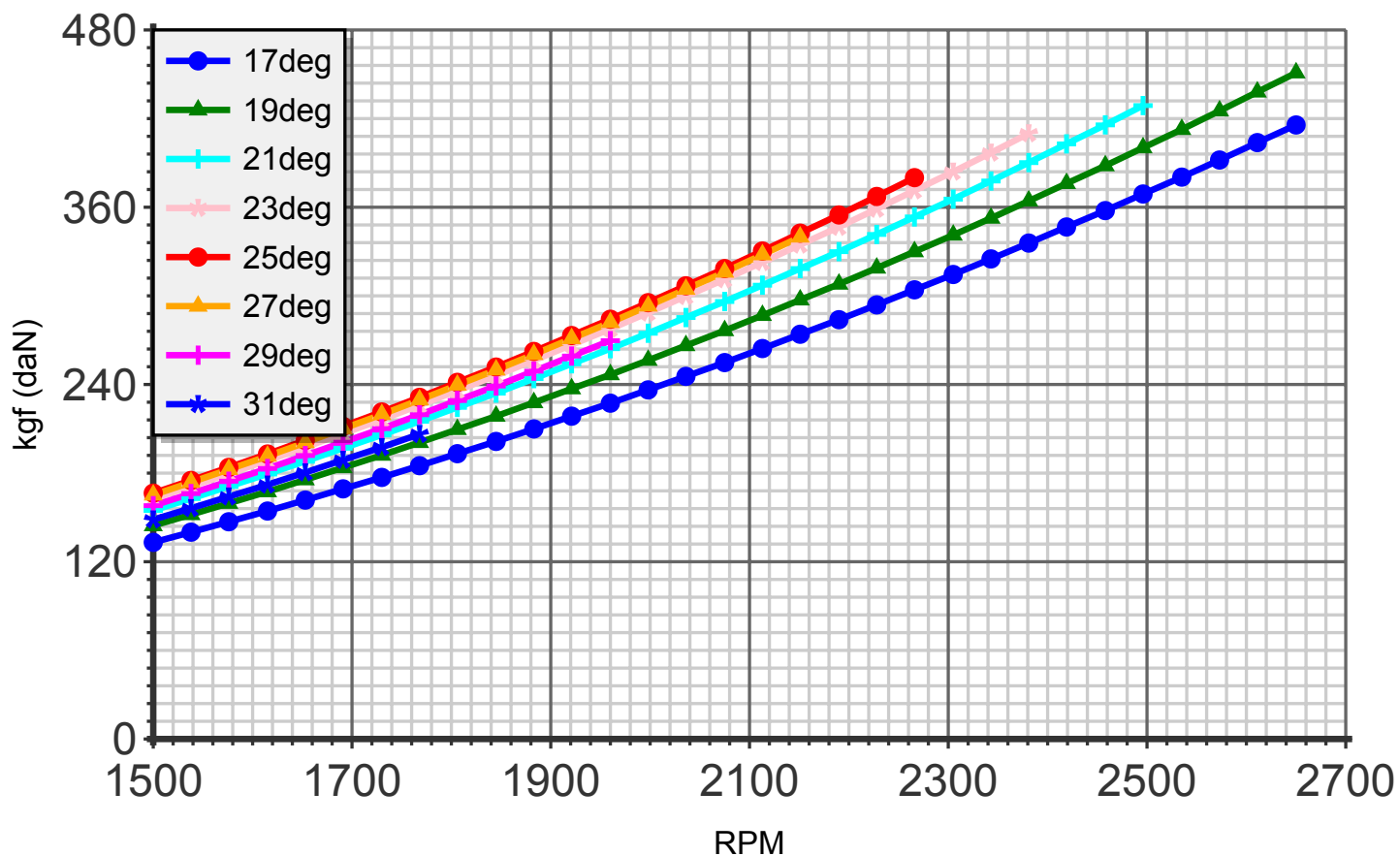
Thrust (blade:4 diameter:187cm C4)
