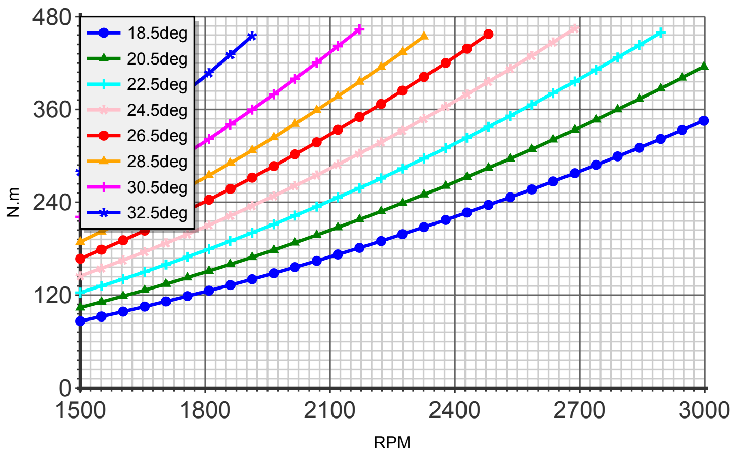
Torque (blade:3 diameter:165cm C8)
