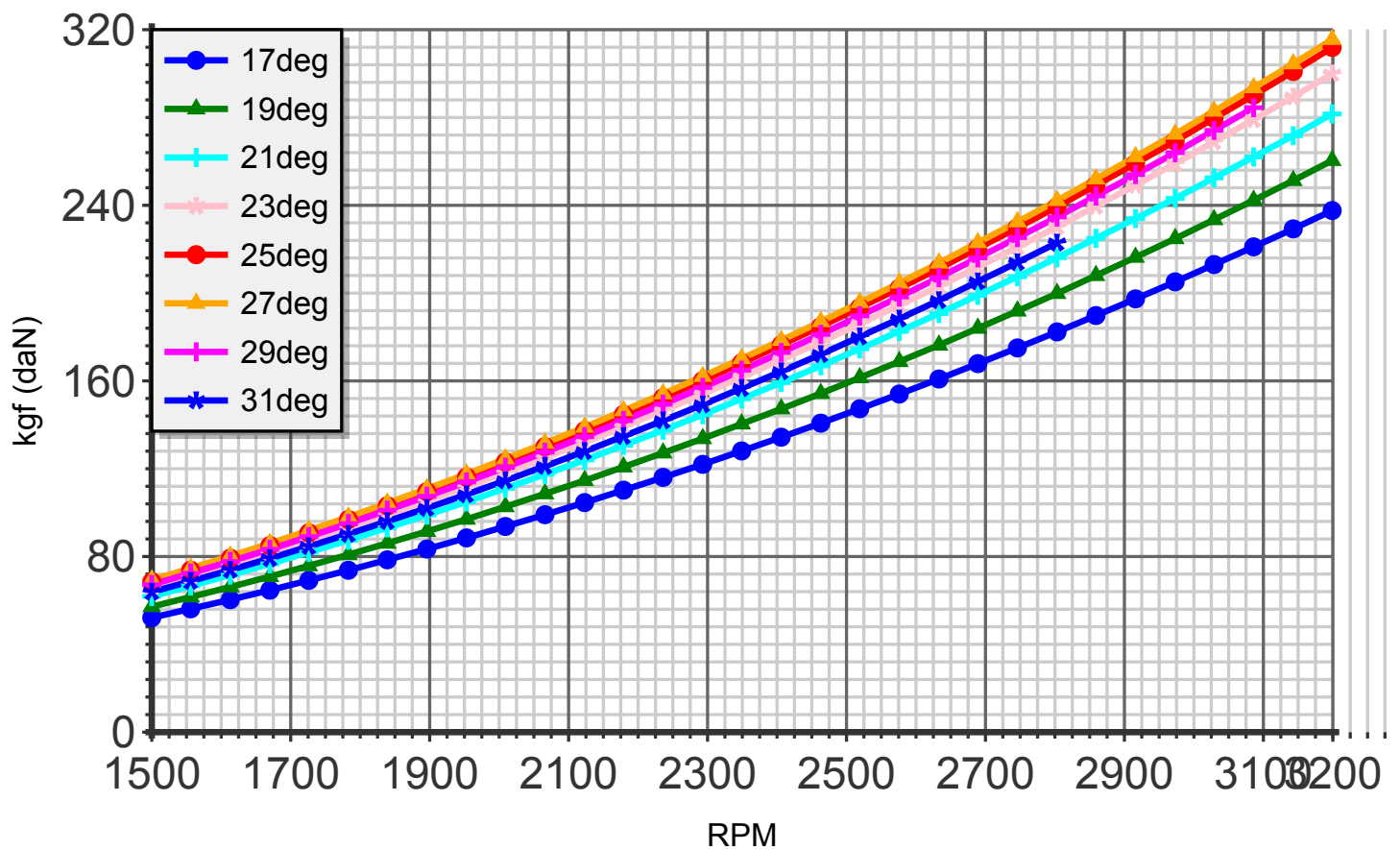
Thrust (blade:3 diameter:155cm C4)
