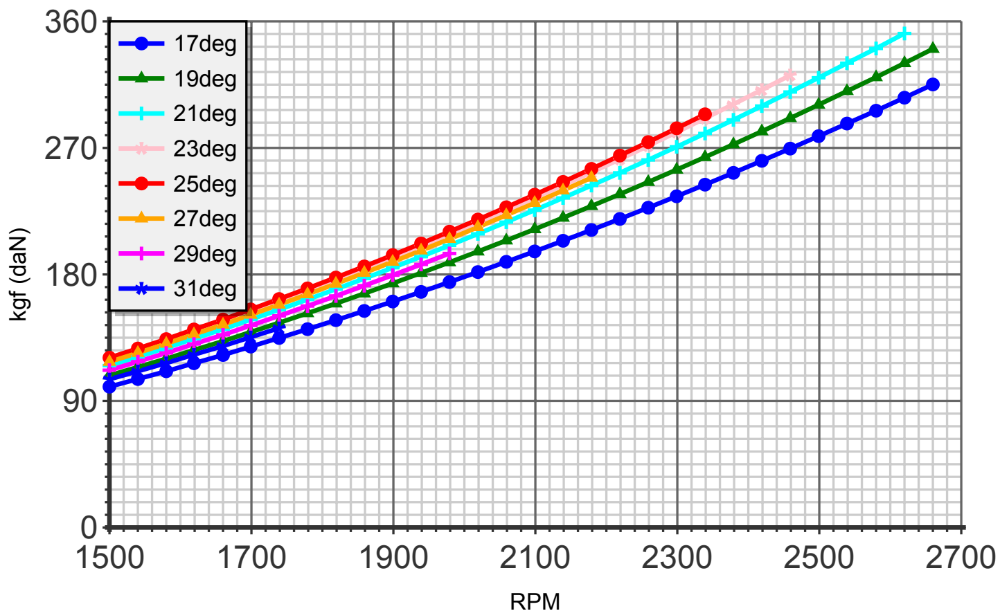
Thrust (blade:3 diameter:185cm C4)
