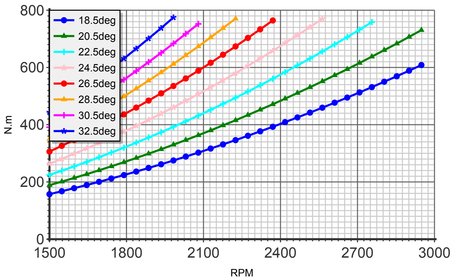
Torque (blade:5 diameter:169cm C8)
