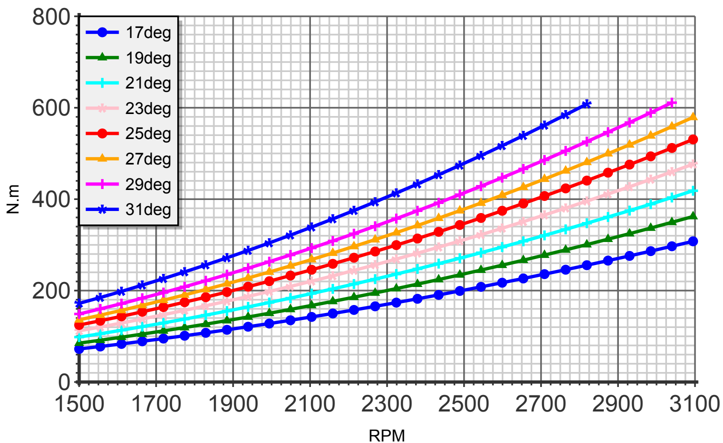
Torque (blade:4 diameter:157cm C4)
