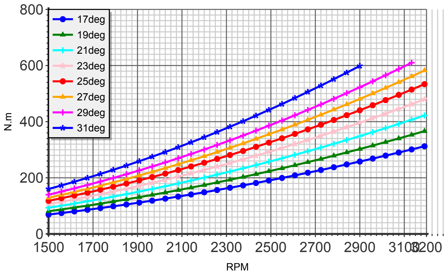
Torque (blade:4 diameter:152cm C4)
