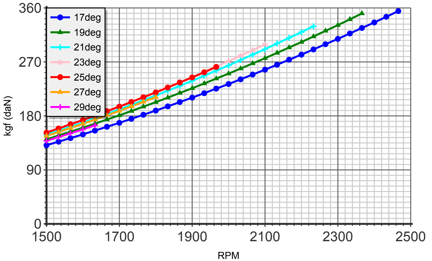
Thrust (blade:3 diameter:200cm C4)
