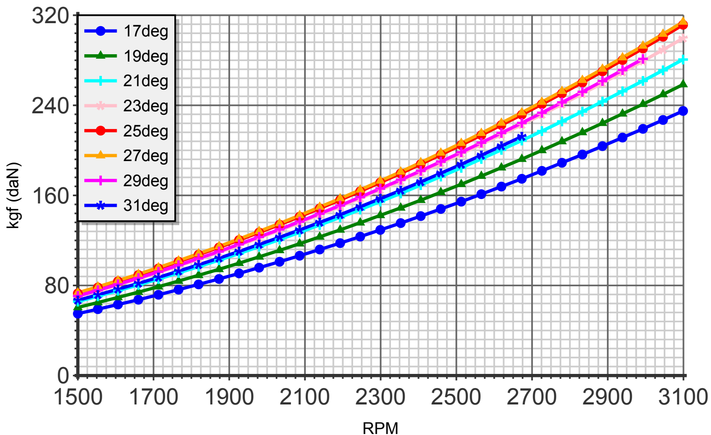
Thrust (blade:3 diameter:160cm C4)
