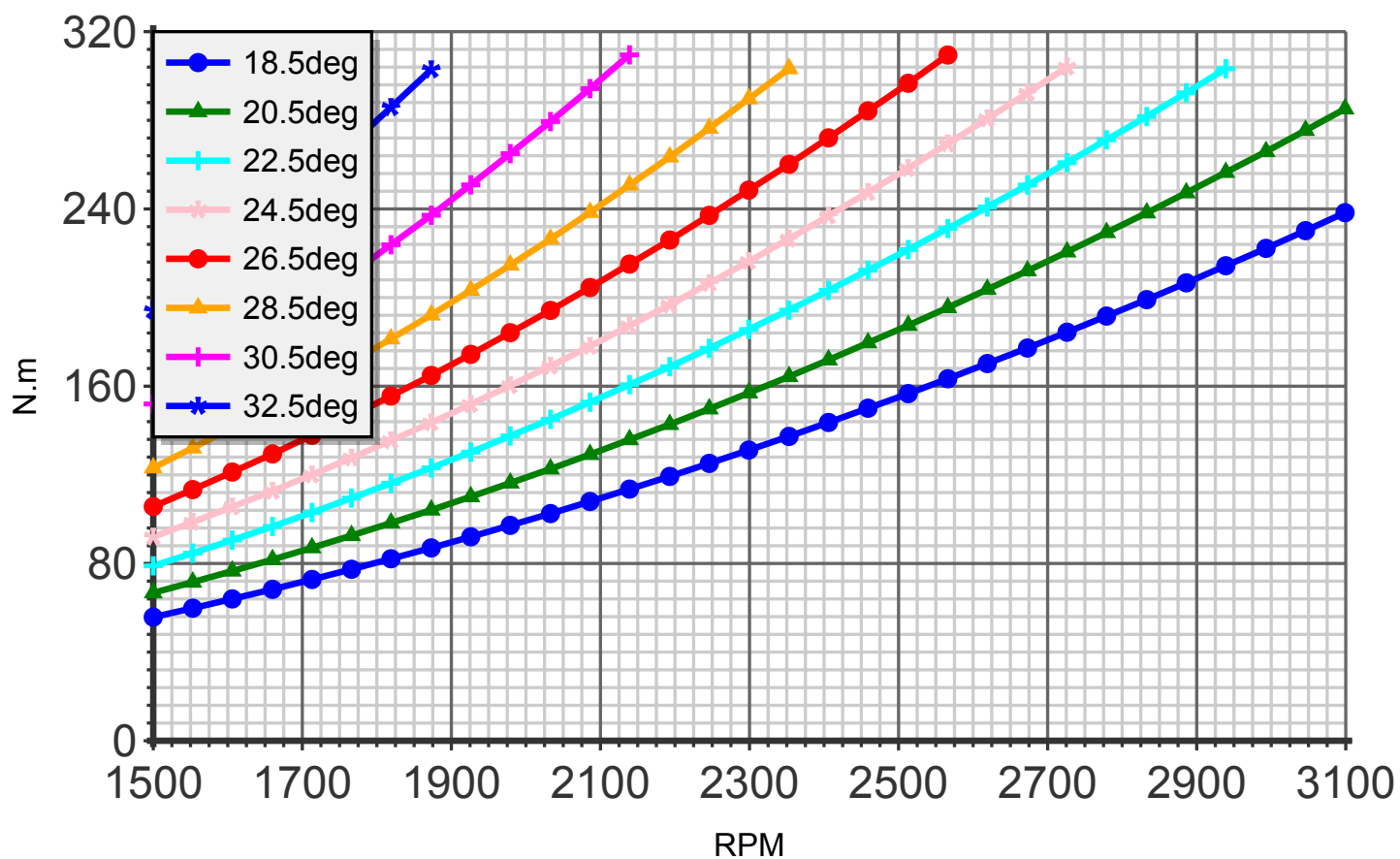
Torque (blade:2 diameter:160cm C8)
