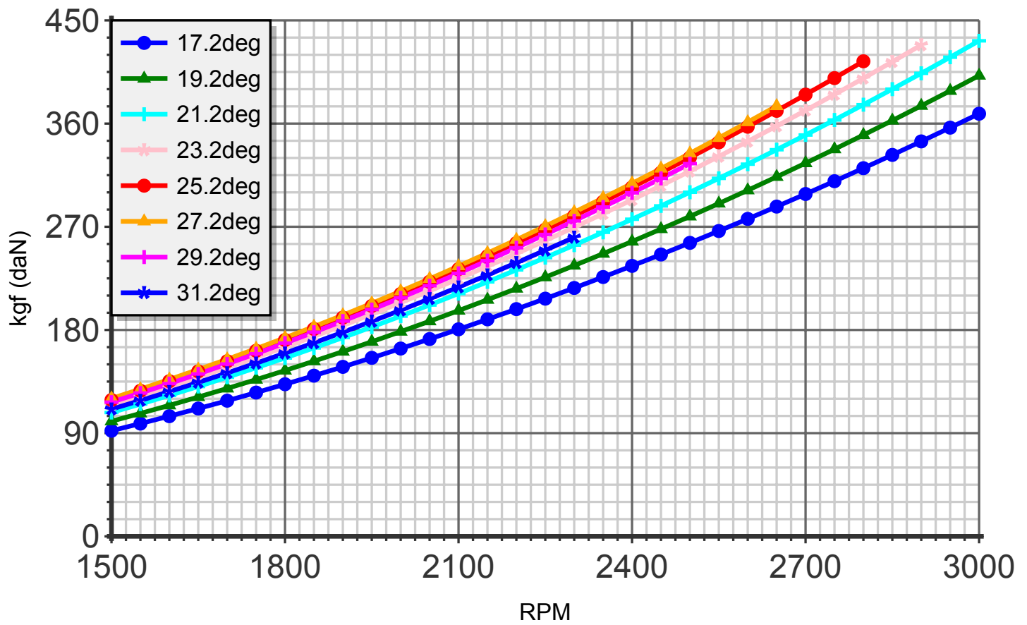
Thrust (blade:4 diameter:167cm C4)
