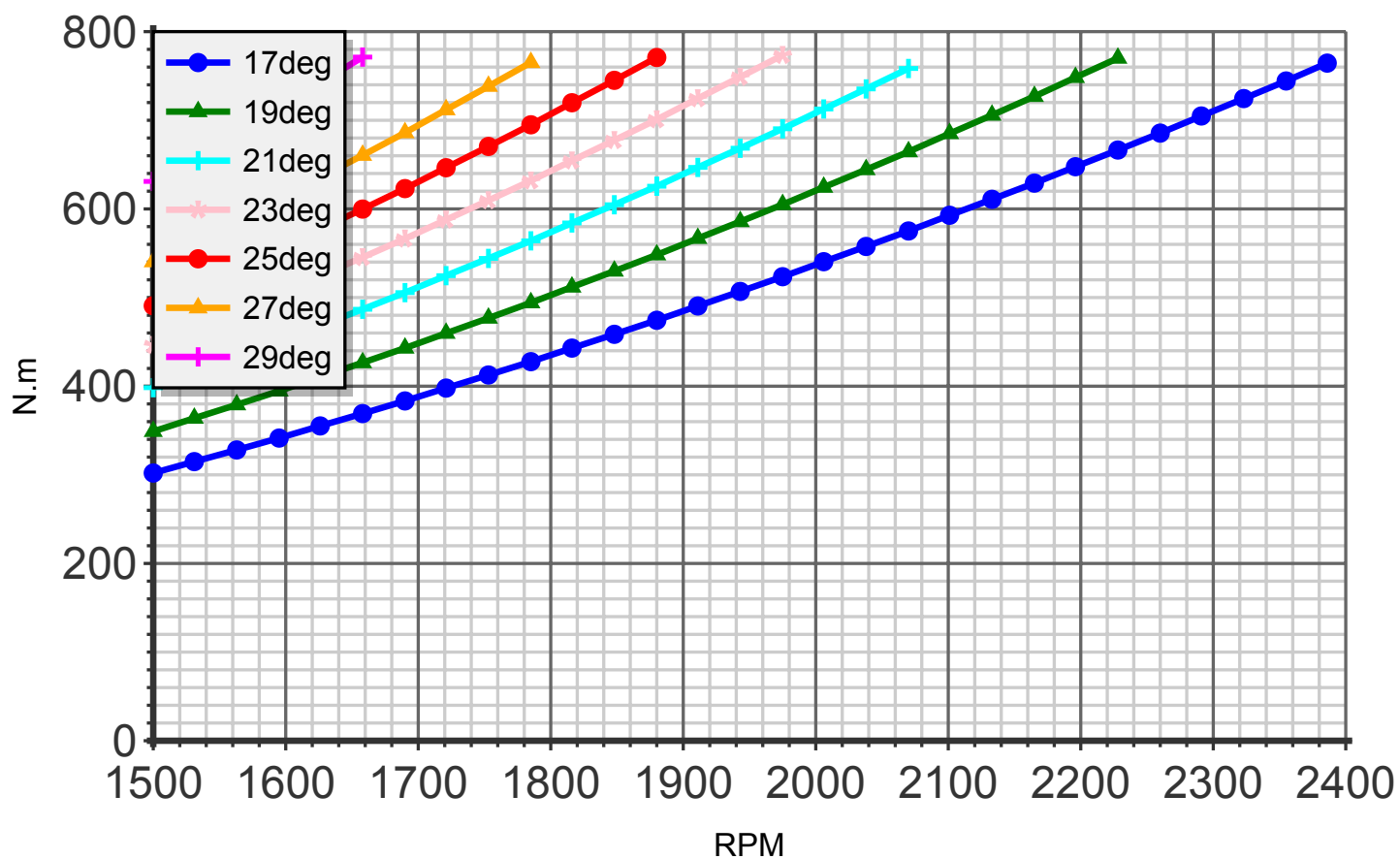
Torque (blade:5 diameter:204cm C4)
