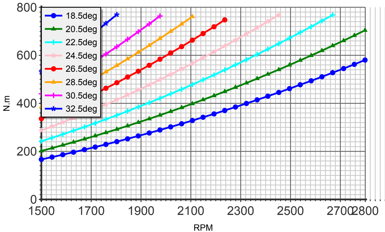
Torque (blade:5 diameter:179cm C8)
