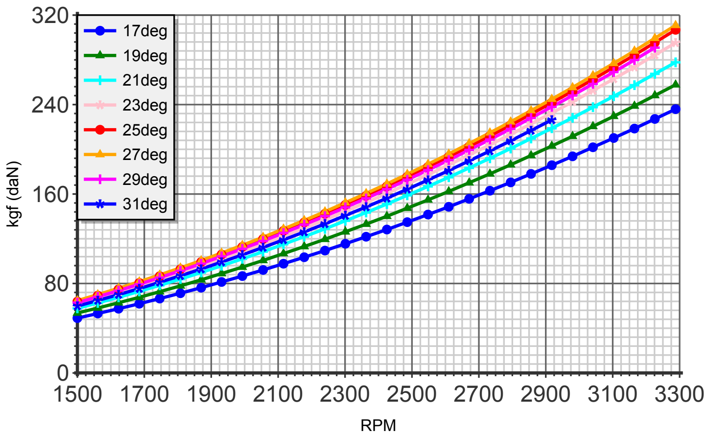
Thrust (blade:3 diameter:150cm C4)
