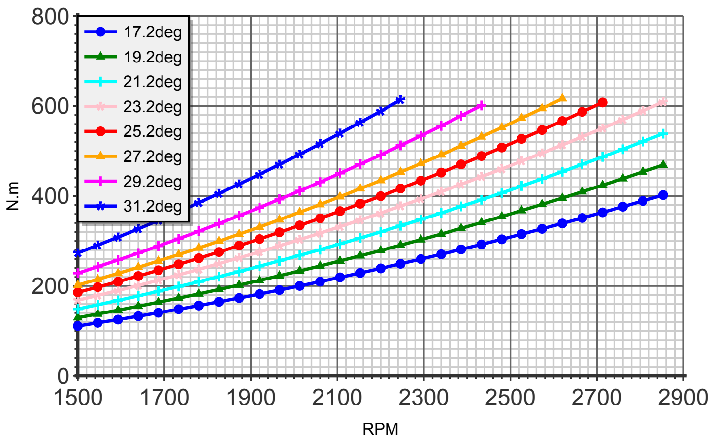
Torque (blade:4 diameter:172cm C4)
