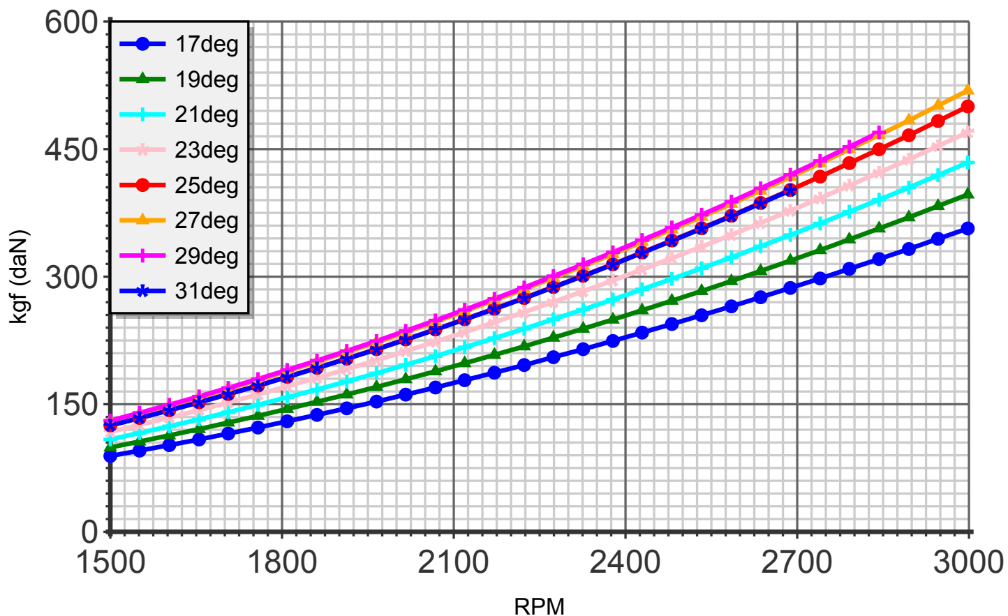
Thrust (blade:5 diameter:164cm C4)
