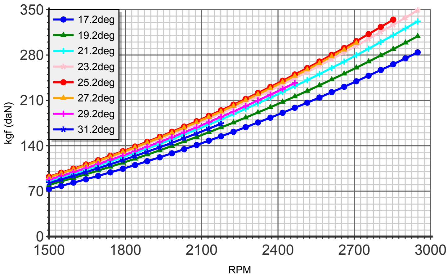
Thrust (blade:3 diameter:170cm C4)
