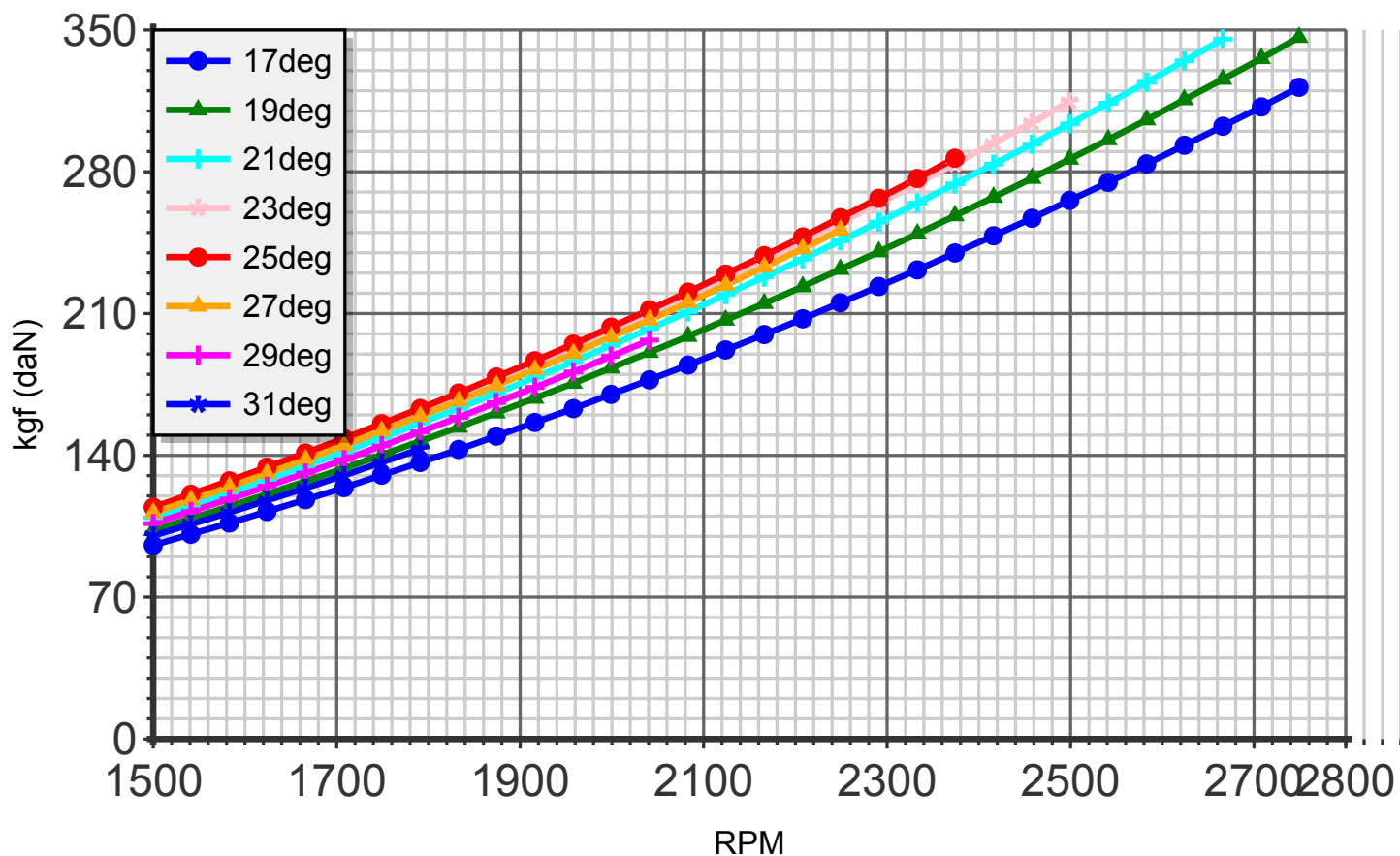
Thrust (blade:3 diameter:180cm C4)
