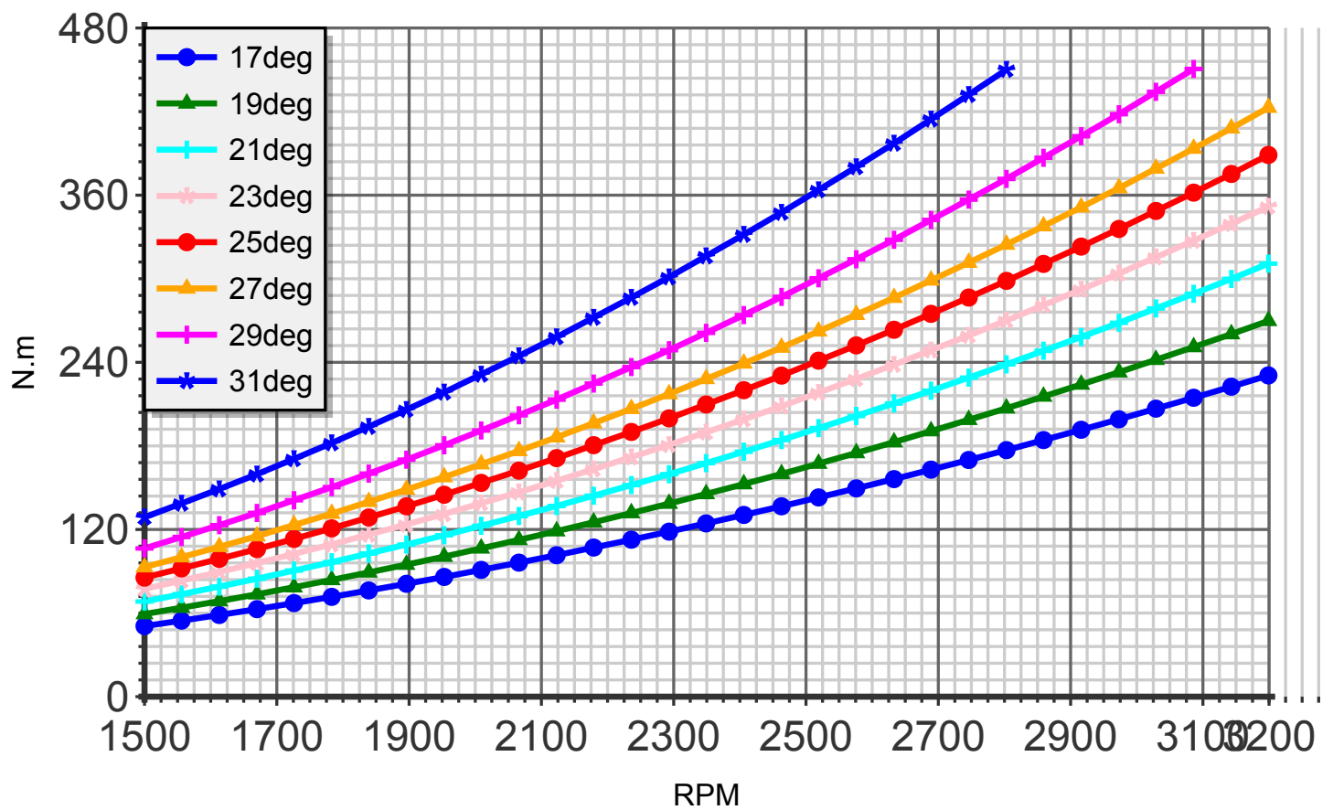
Torque (blade:3 diameter:155cm C4)
