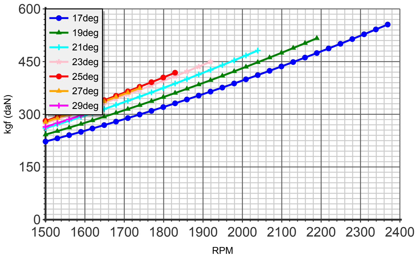
Thrust (blade:5 diameter:209cm C4)
