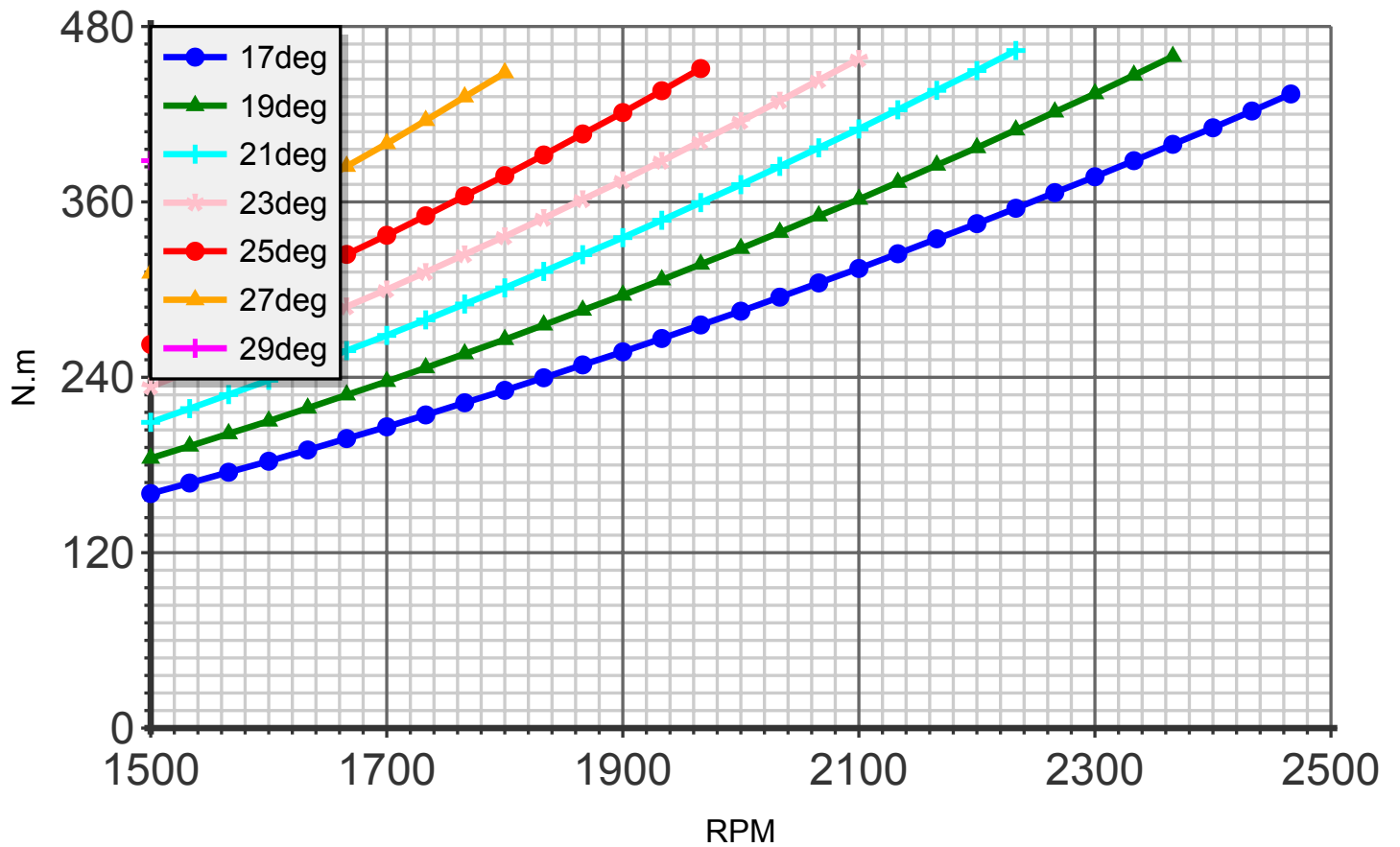
Torque (blade:3 diameter:200cm C4)
