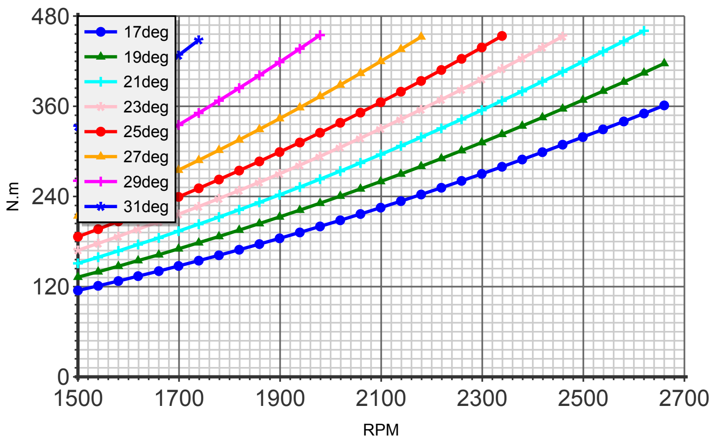
Torque (blade:3 diameter:185cm C4)
