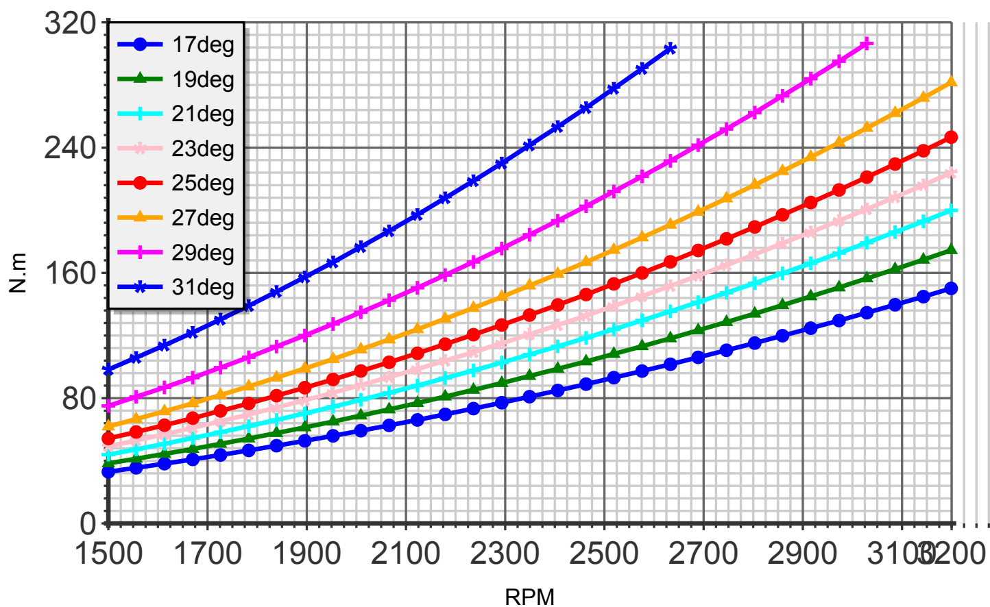
Torque (blade:2 diameter:155cm C4)
