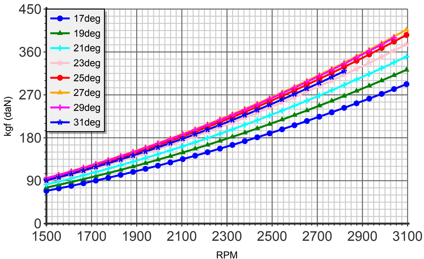
Thrust (blade:4 diameter:157cm C4)
