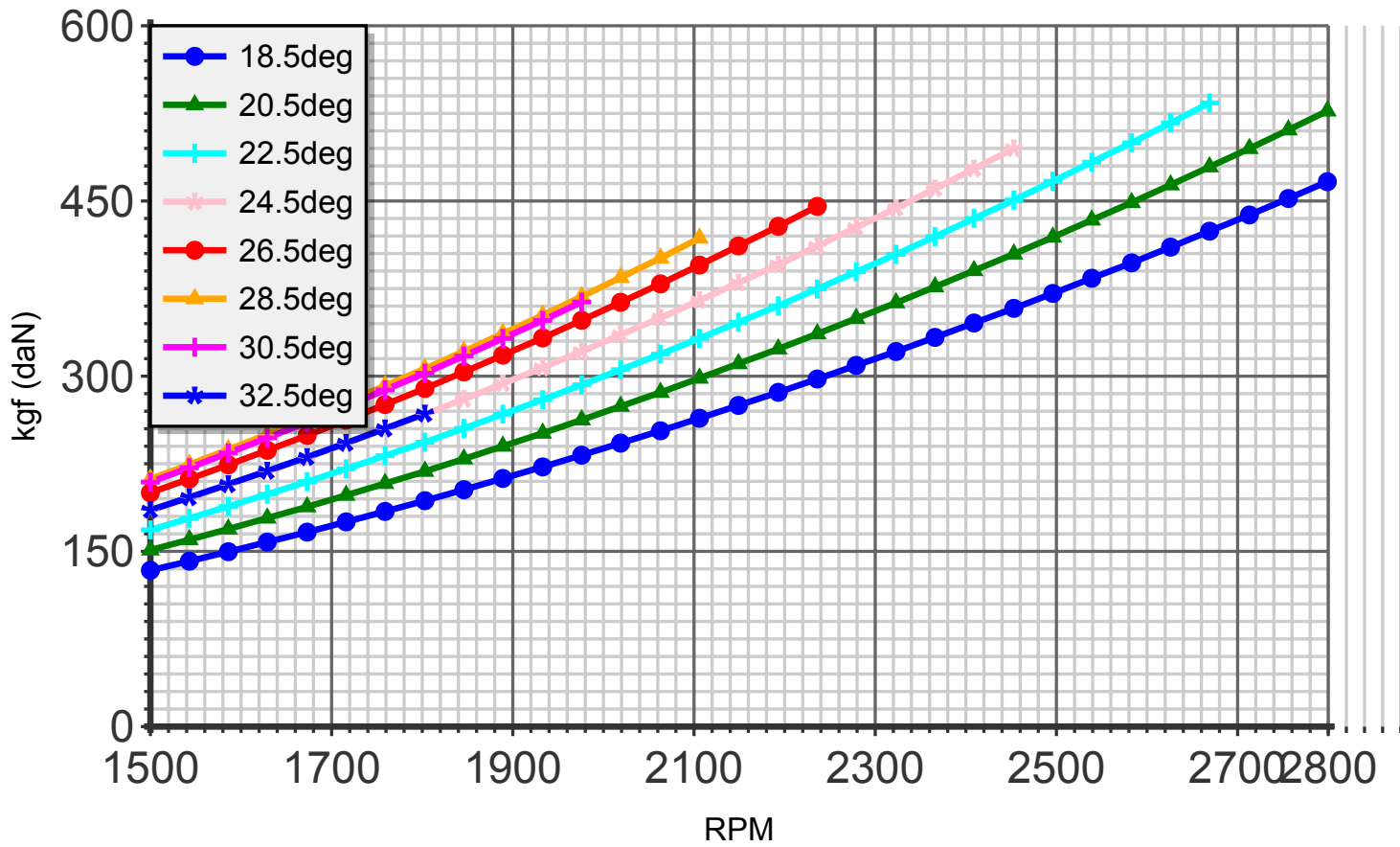
Thrust (blade:5 diameter:179cm C8)
