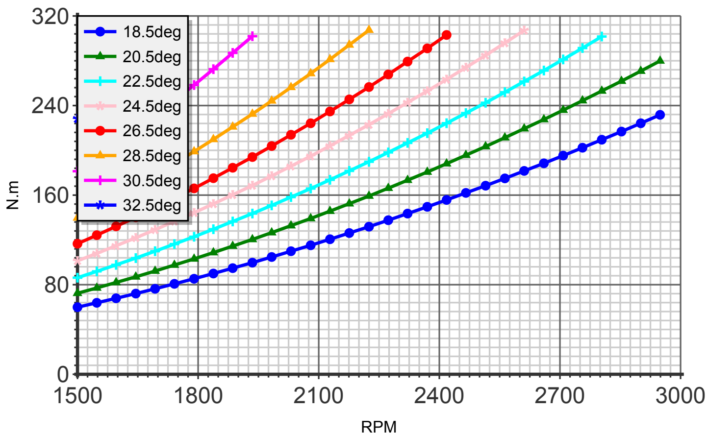
Torque (blade:2 diameter:170cm C8)
