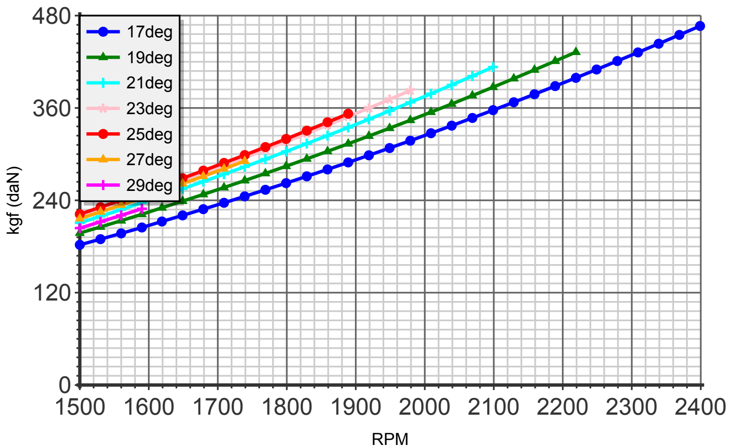
Thrust (blade:4 diameter:208cm C4)
