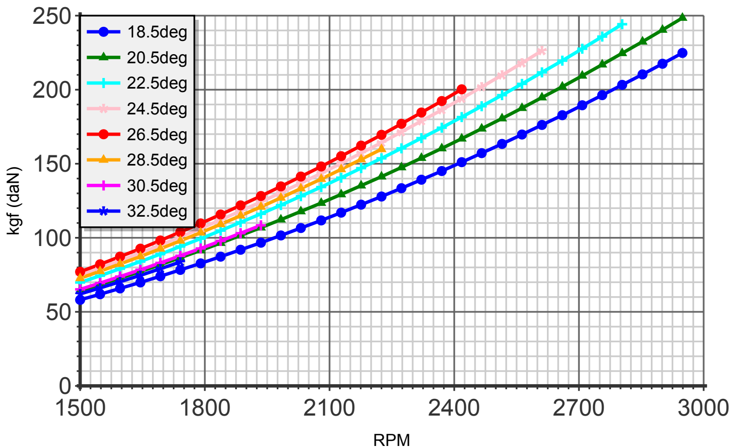
Thrust (blade:2 diameter:170cm C8)
