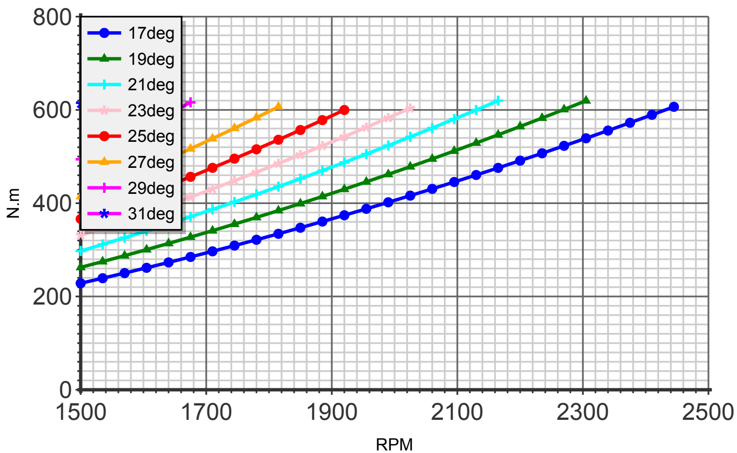
Torque (blade:4 diameter:198cm C4)
