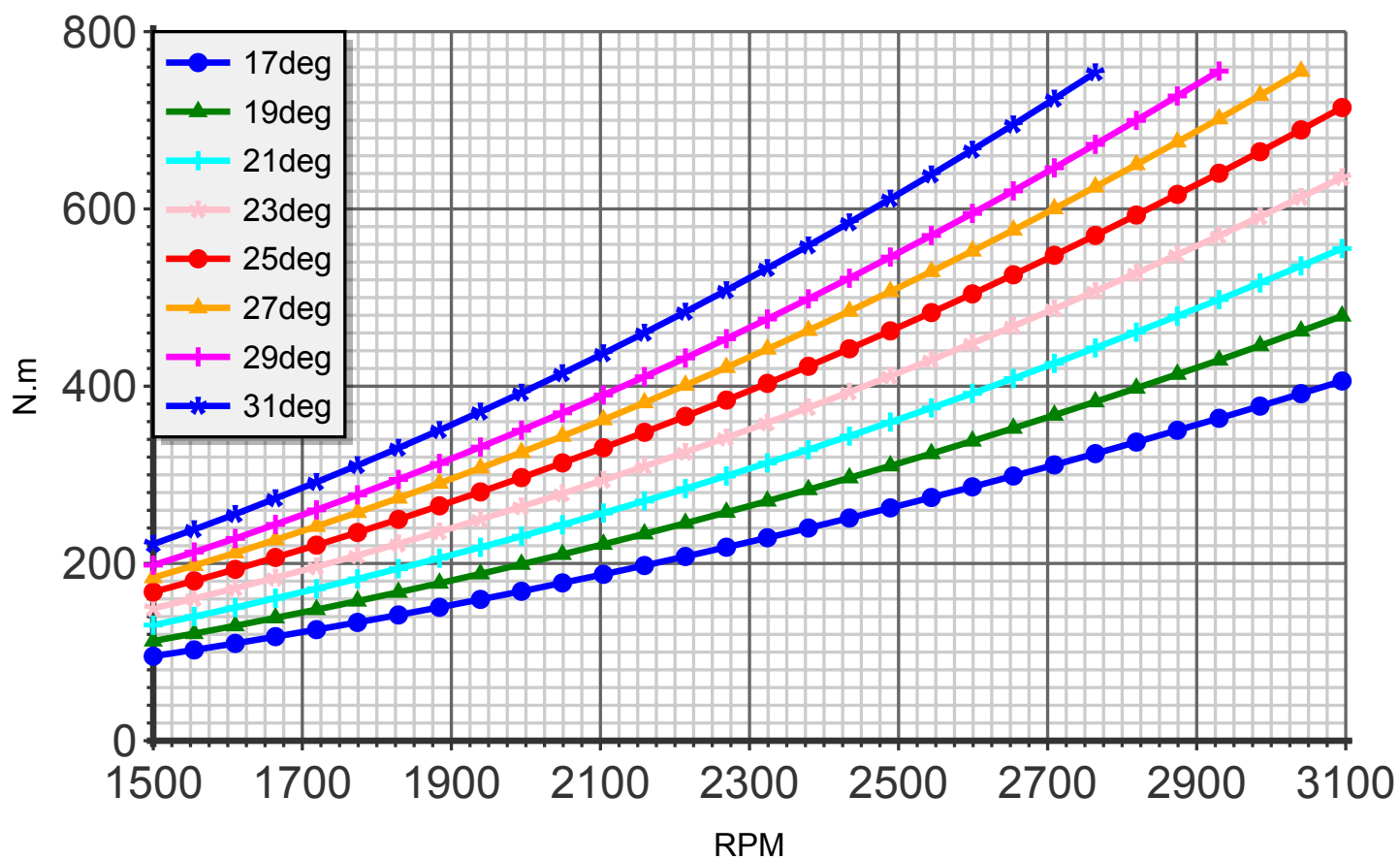
Torque (blade:5 diameter:159cm C4)
