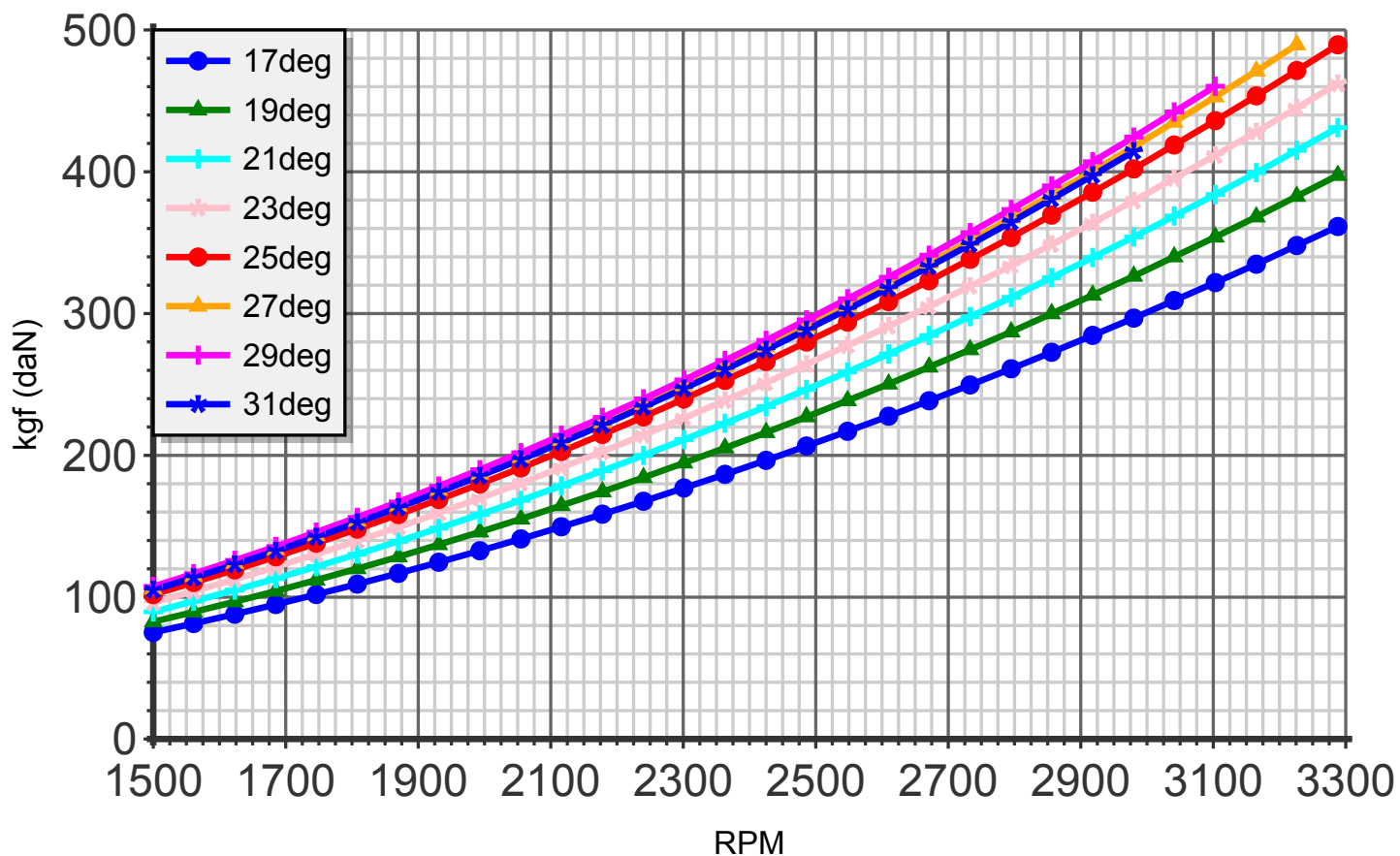
Thrust (blade:5 diameter:149cm C4)
