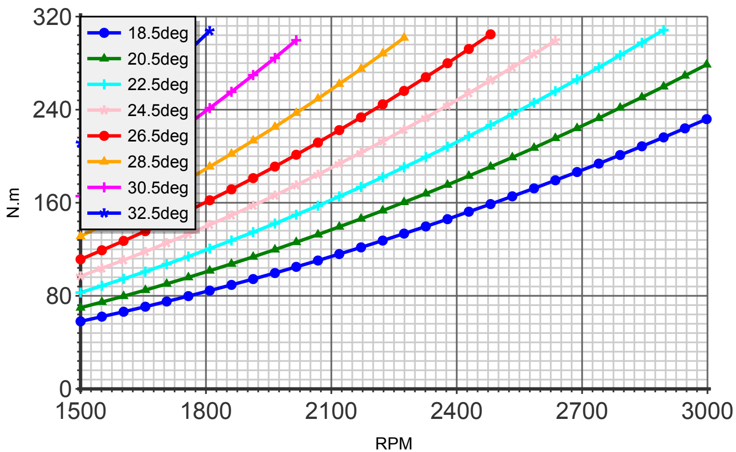
Torque (blade:2 diameter:165cm C8)
