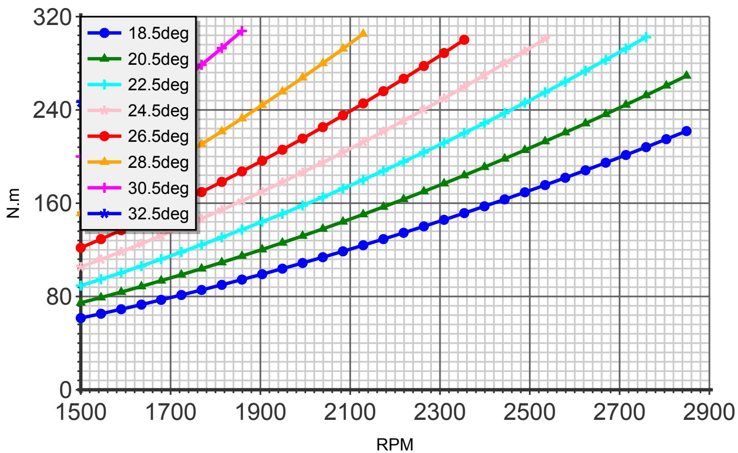
Torque (blade:2 diameter:175cm C8)
