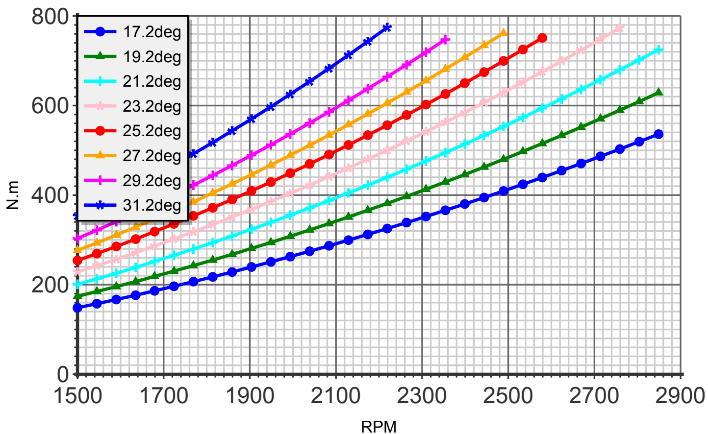
Torque (blade:5 diameter:176cm C4)
