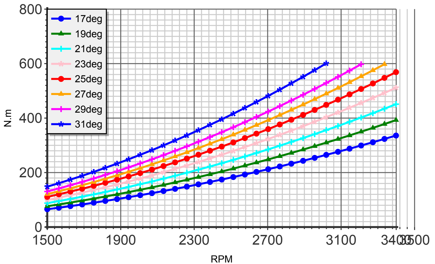
Torque (blade:4 diameter:147cm C4)
