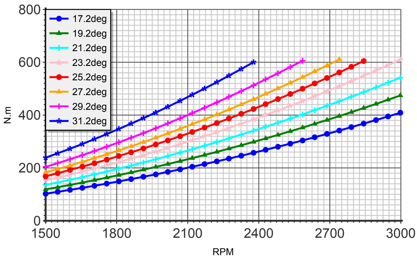
Torque (blade:4 diameter:162cm C4)
