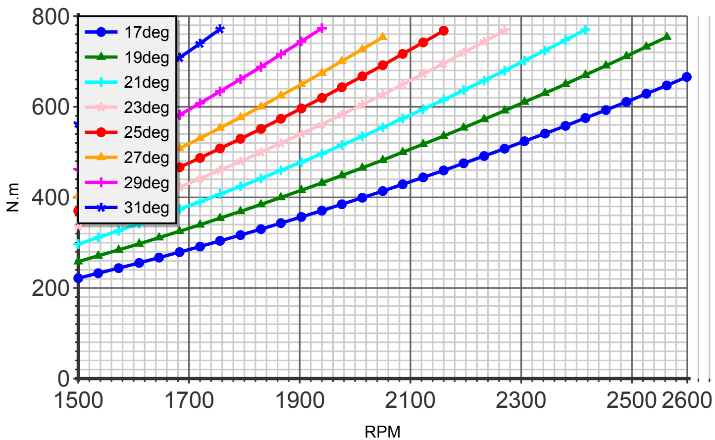
Torque (blade:5 diameter:194cm C4)
