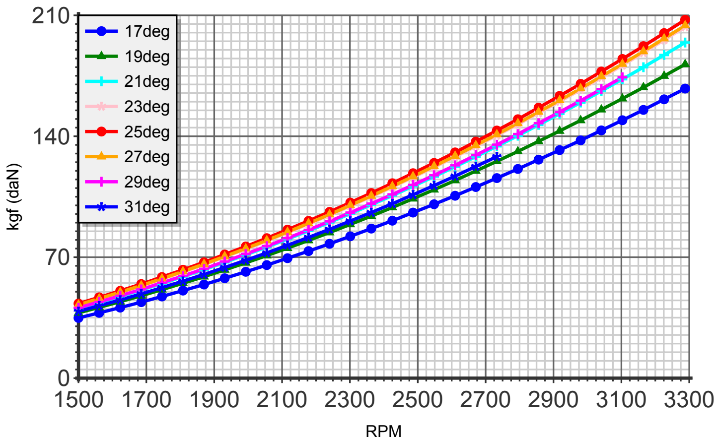
Thrust (blade:2 diameter:150cm C4)
