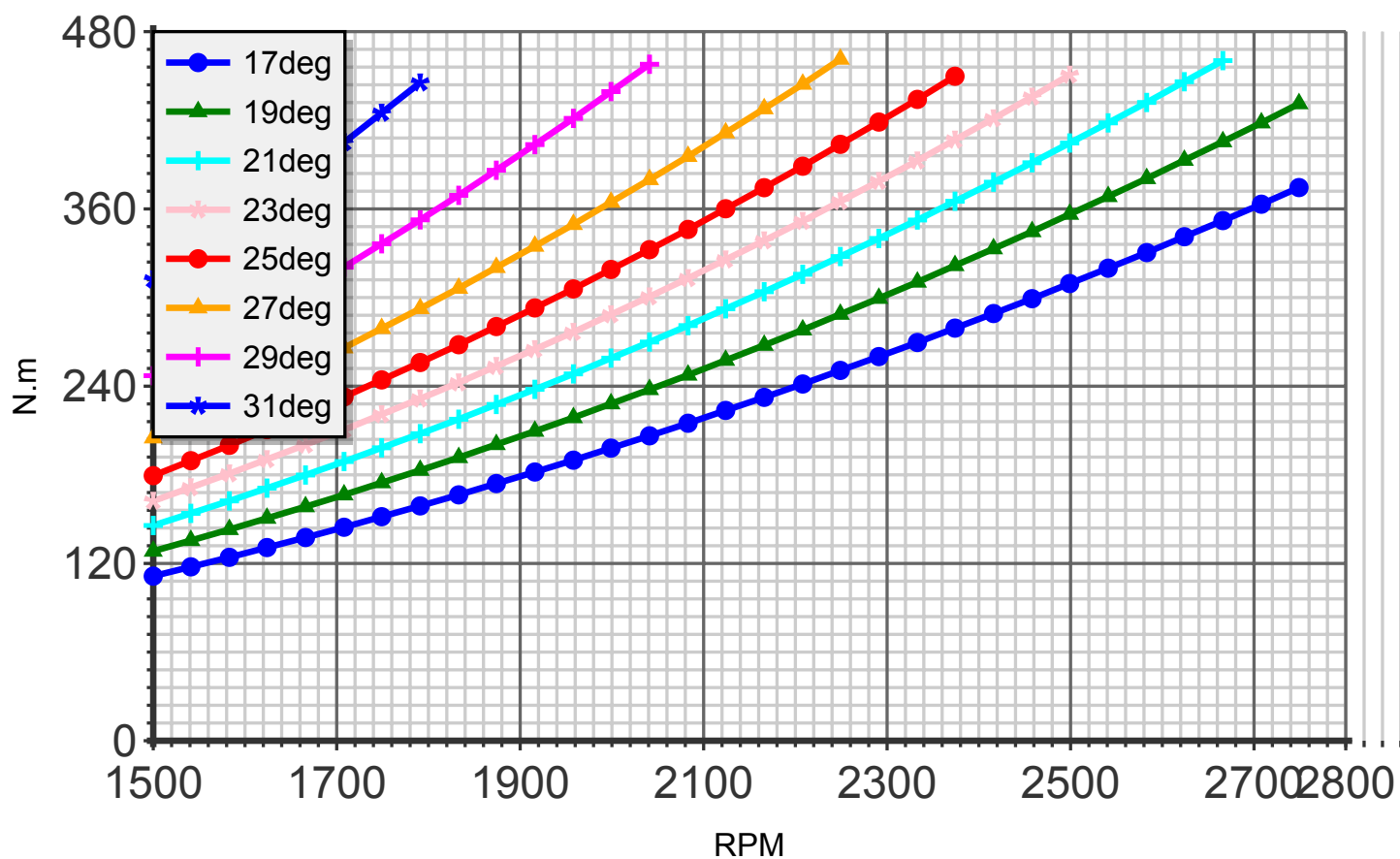
Torque (blade:3 diameter:180cm C4)
