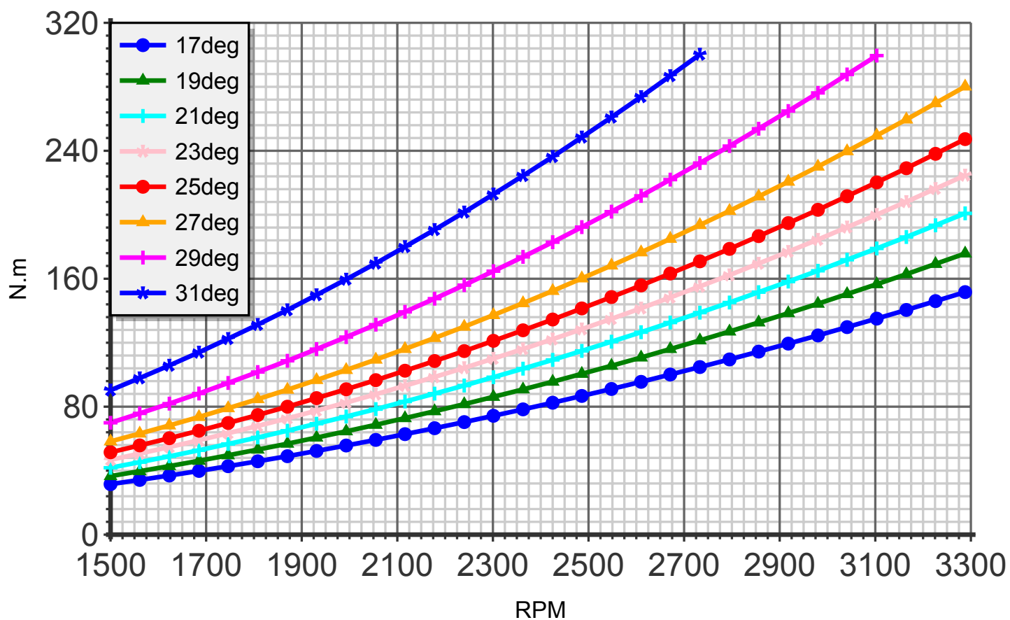
Torque (blade:2 diameter:150cm C4)
