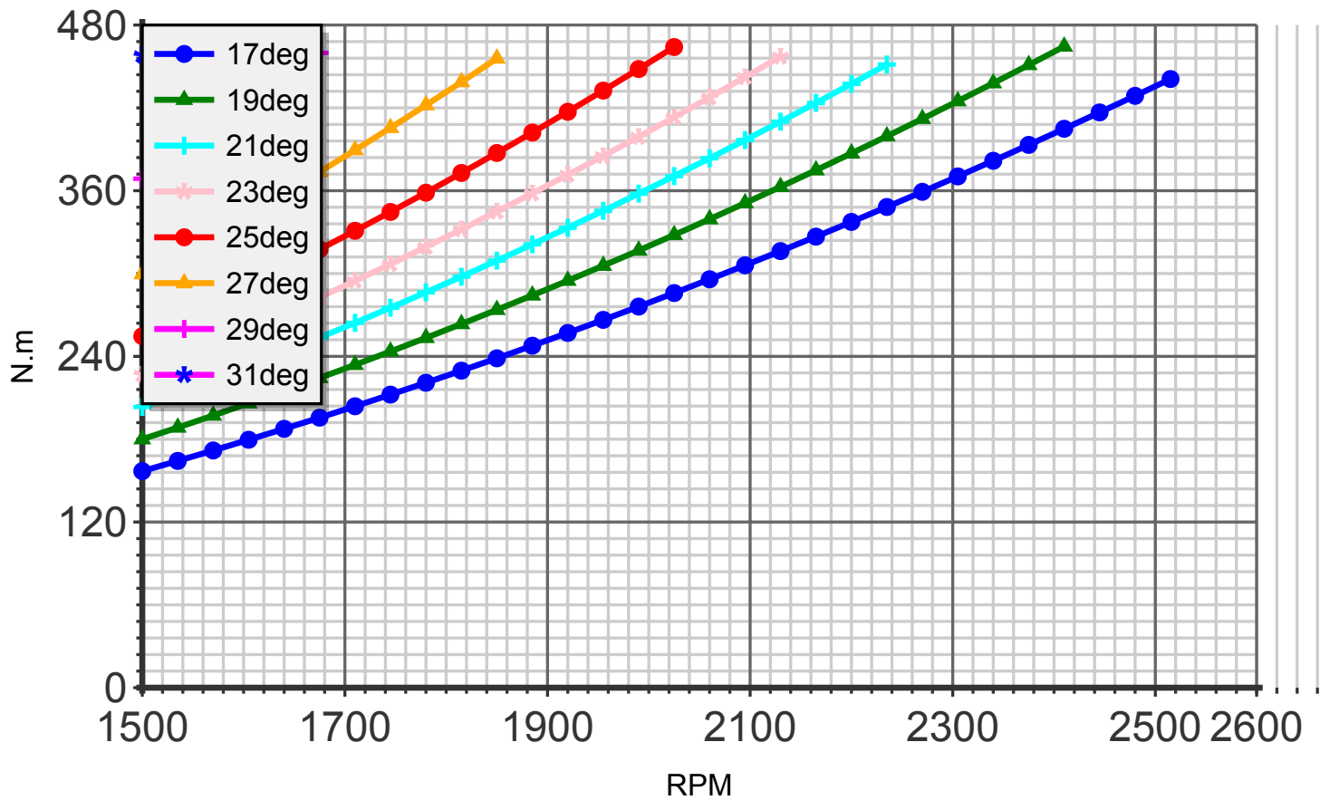
Torque (blade:3 diameter:195cm C4)
