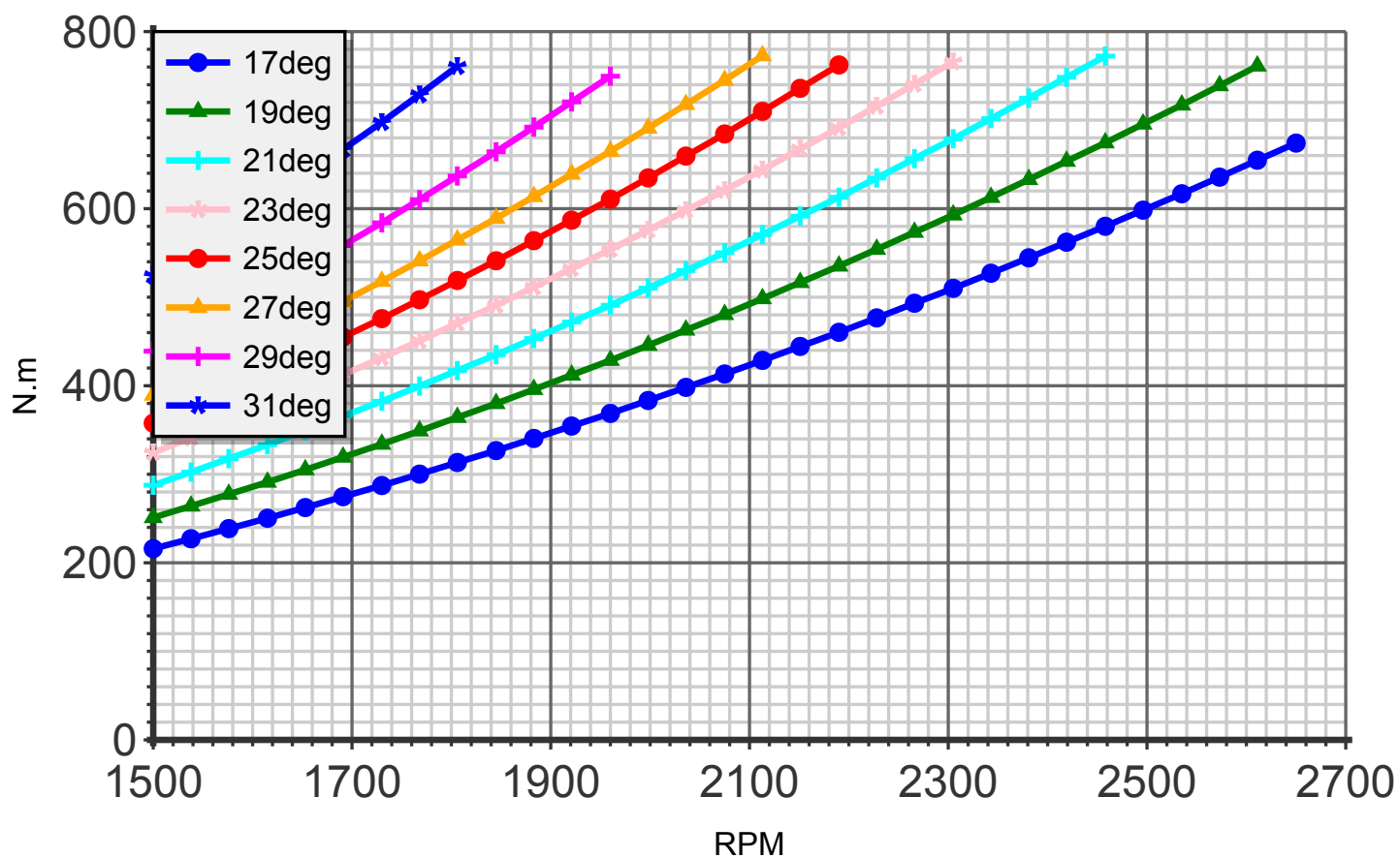
Torque (blade:5 diameter:189cm C4)
