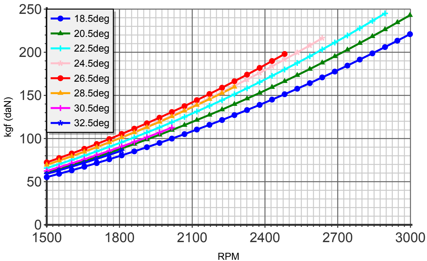
Thrust (blade:2 diameter:165cm C8)
