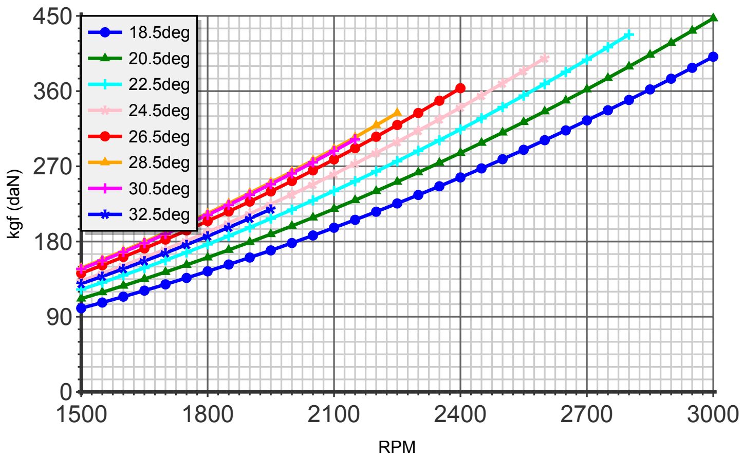
Thrust (blade:4 diameter:167cm C8)
