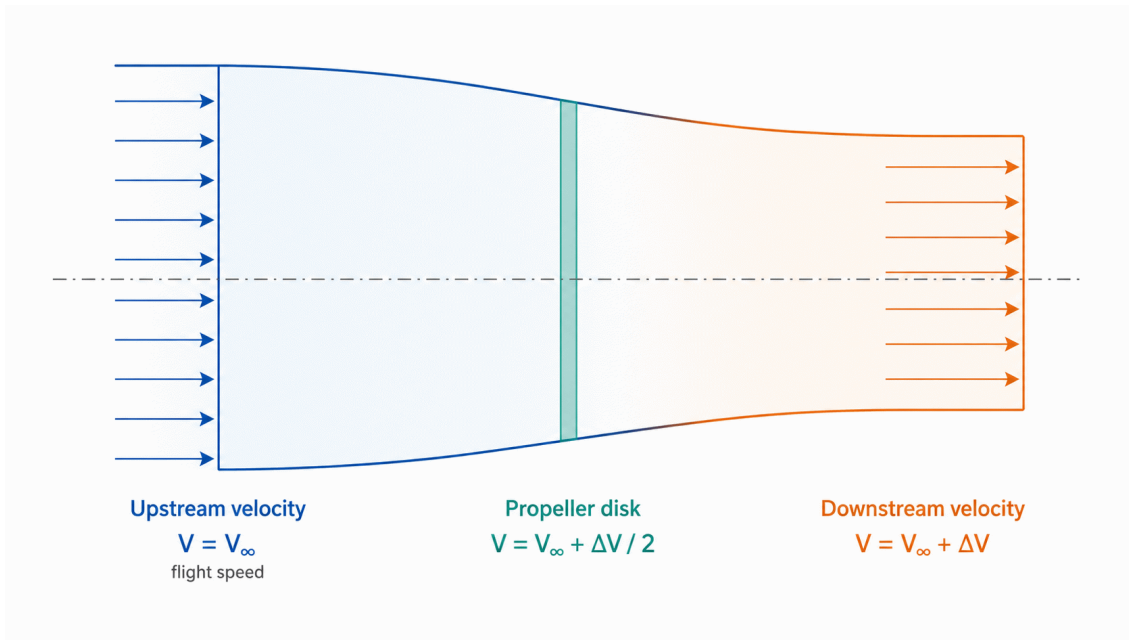
Upstream, disc and downstream flow velocities across the propeller disc
